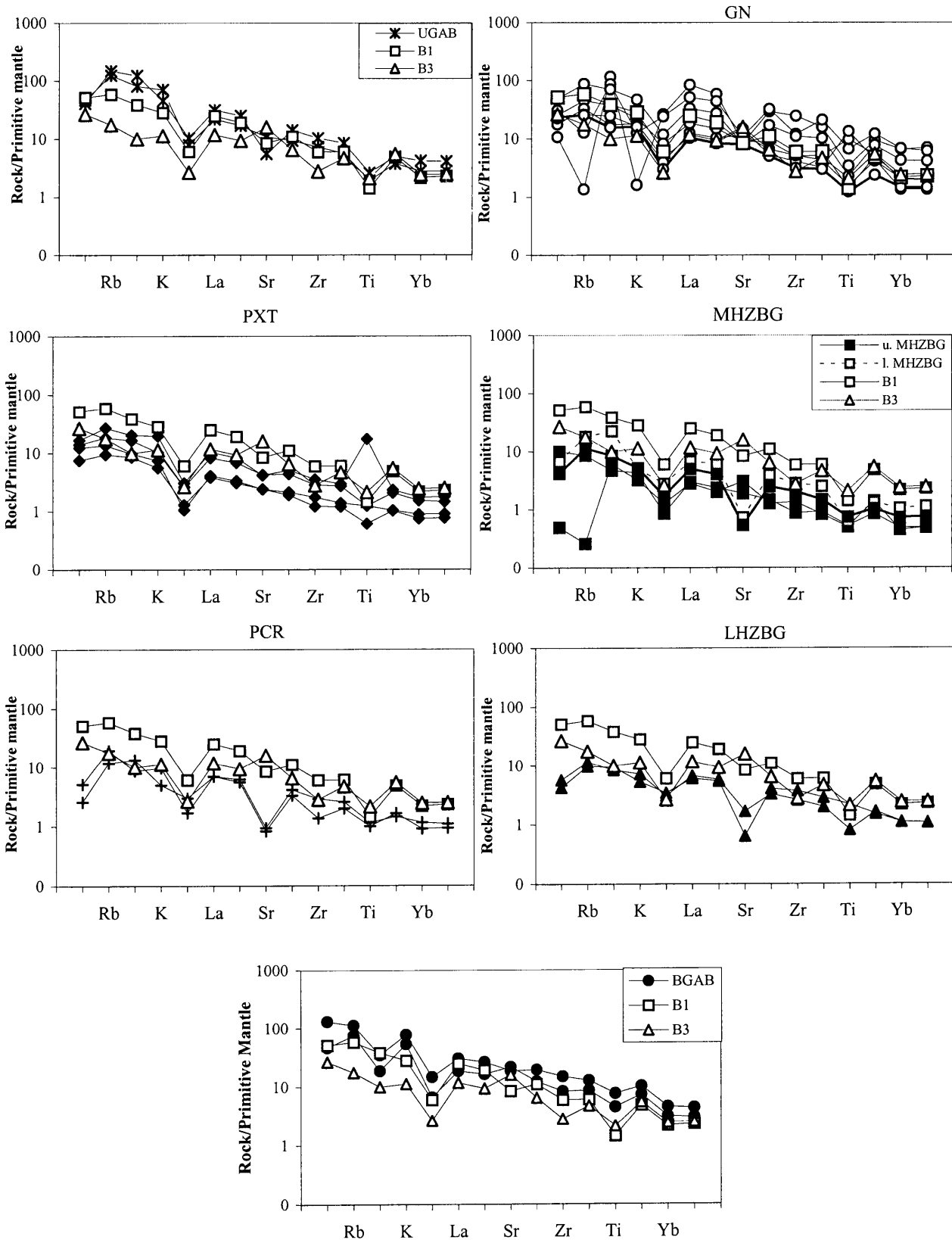
Fig. 4.8. Comparison between the average composition of B1- and B3-magmas and the different Units of the Utkomst Complex (B1 and B3 data from Curl, 2001. Mantle normalization factors are from Sun and McDonough, 1989).
