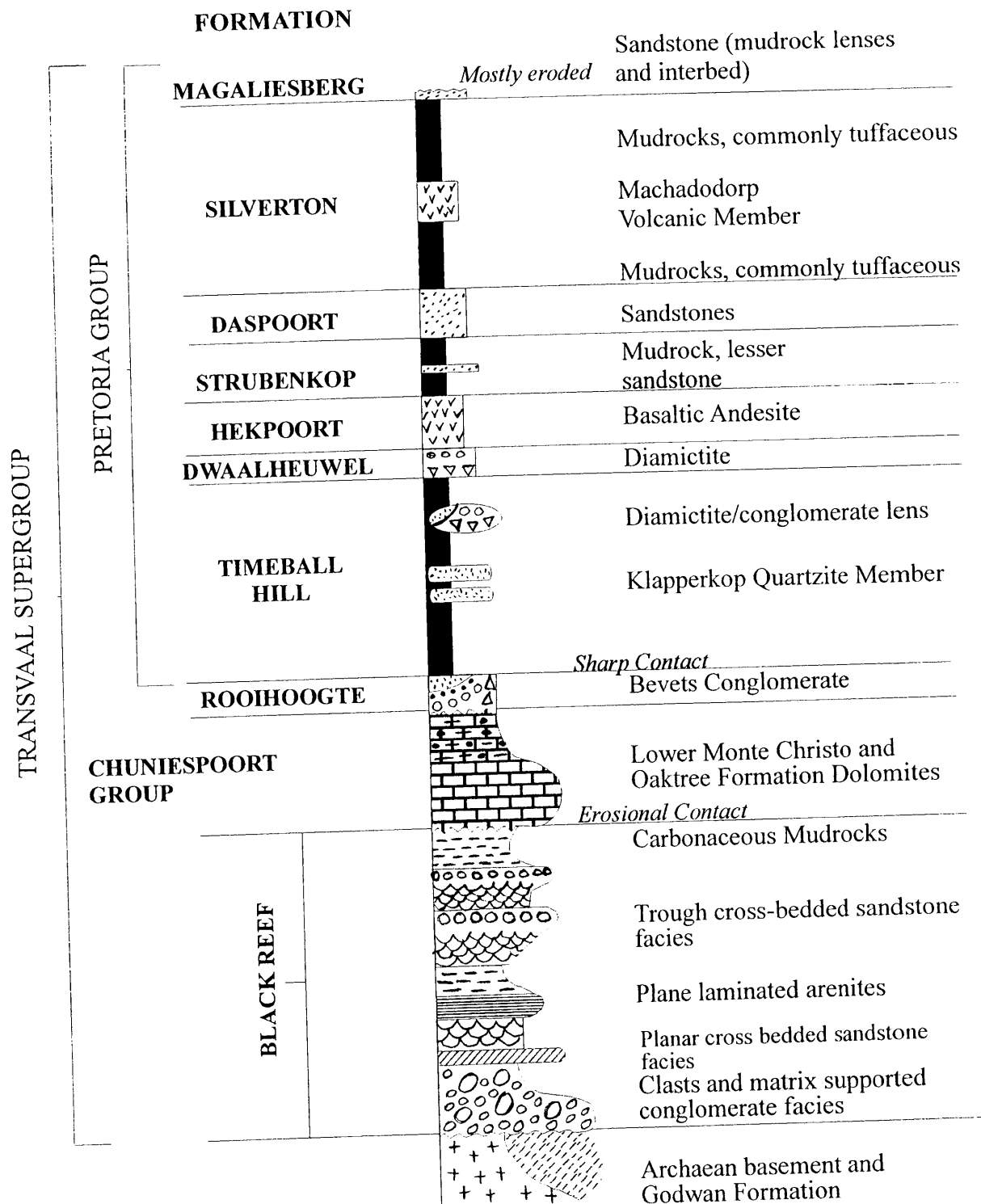
Fig.1.3. Simplified lithostratigraphy of the Eastern Transvaal basin. Vertical scale not proportional. Modified after Eriksson et al. , (1993).
