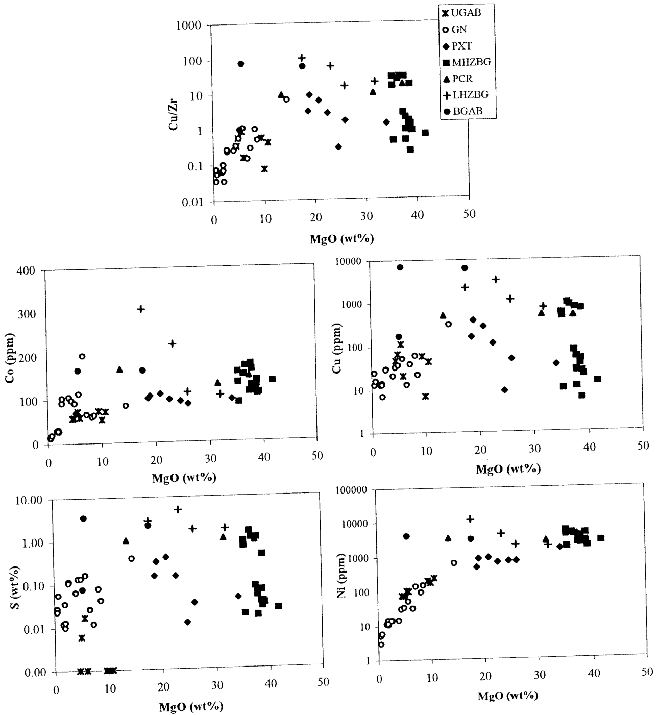
Fig.4.6. Variation diagrams for Cu/Zr and selected chalcophile trace elements plotted against MgO.
