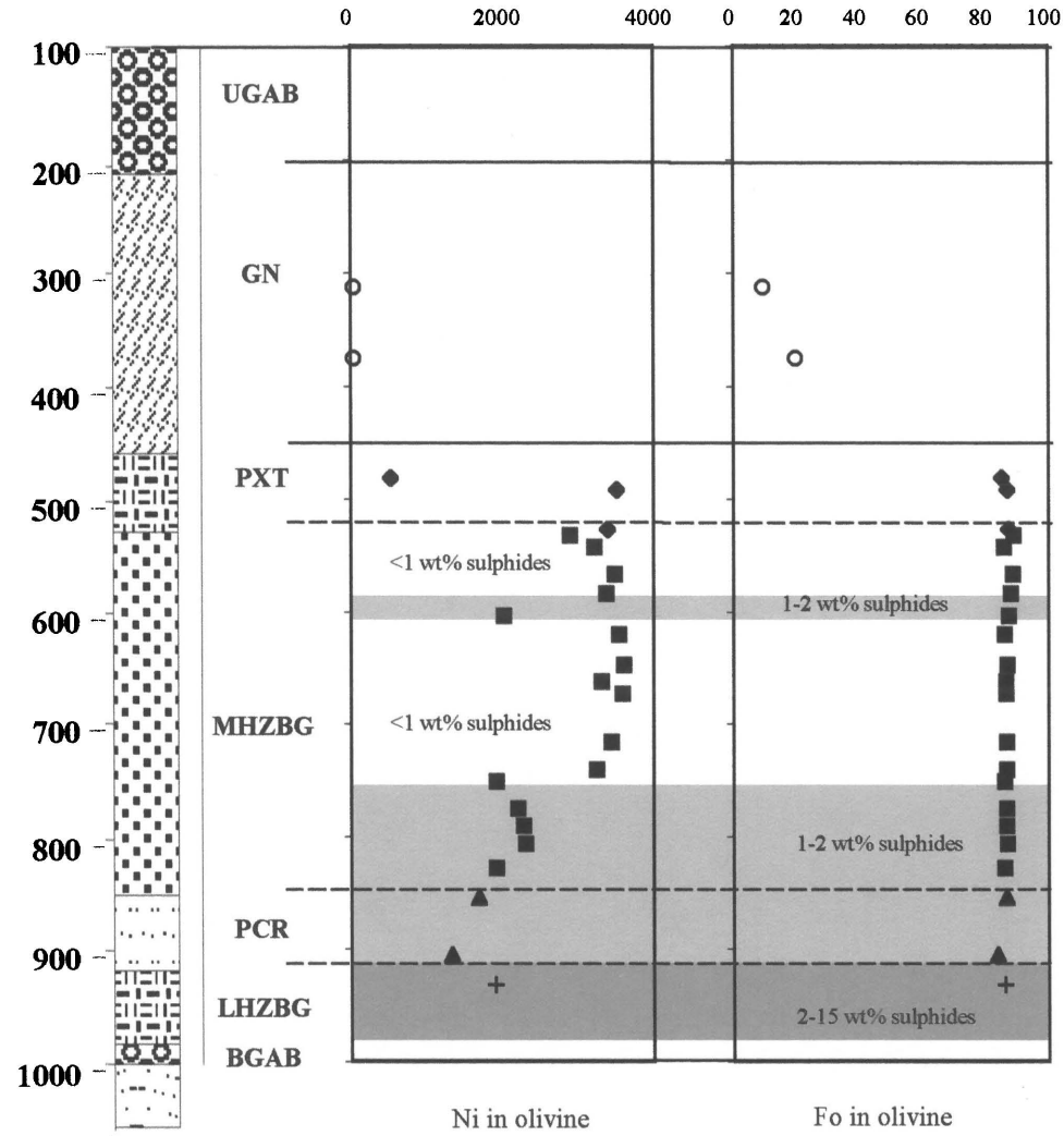
Fig.8.1. Olivine Ni (ppm) and Fo content (mol%) against stratigraphic height (m).
