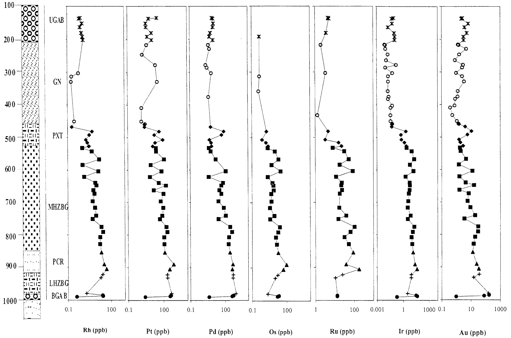
Fig. 5.1. Concentration of PGE and Au plotted versus stratigraphic height (m).
