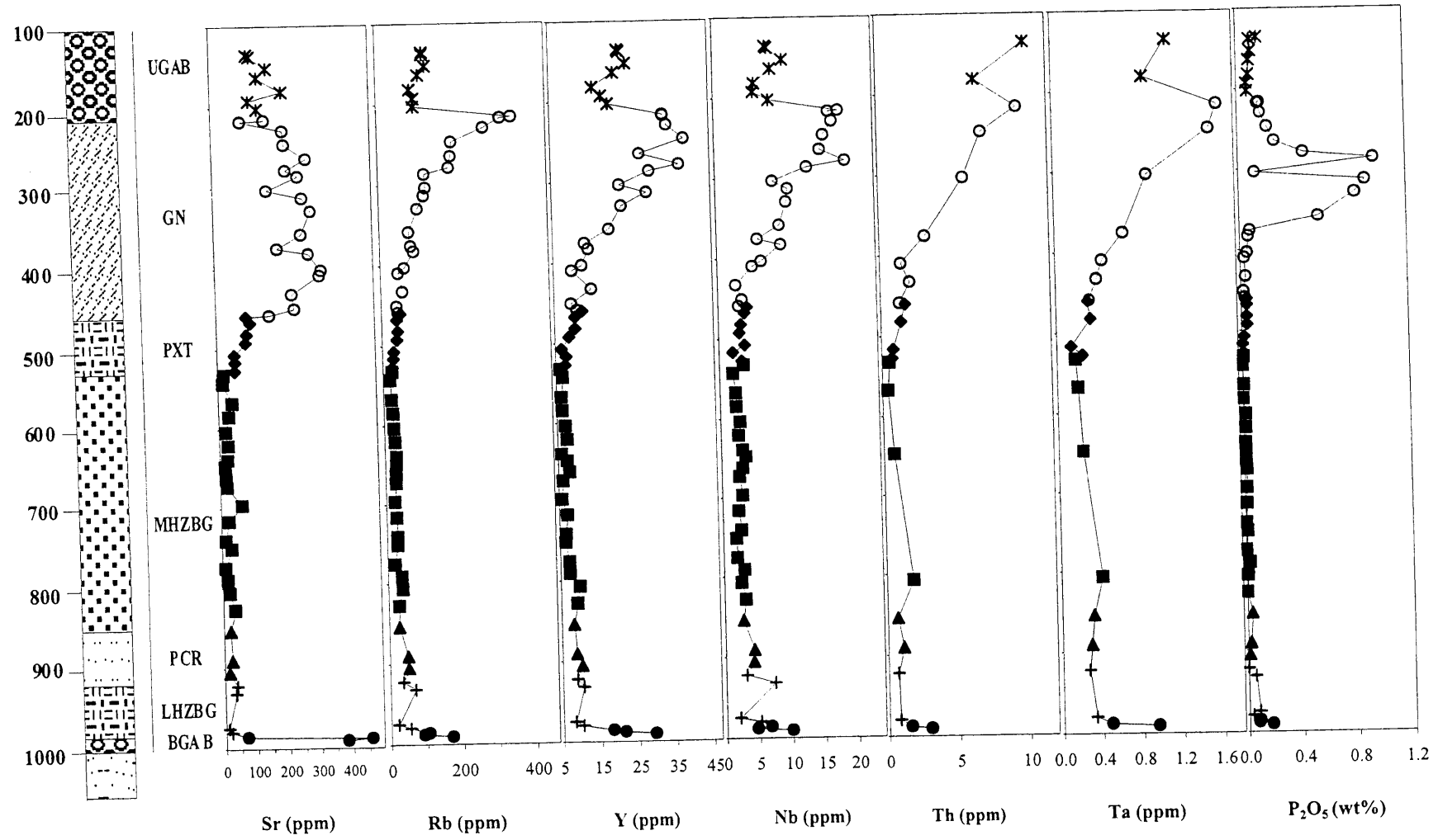
Fig.4.7. (a) Variation diagrams for selected trace elements versus stratigraphic height (m).
