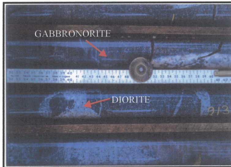
PLATE 1. Gabbronorite section near 123m showing diorite intrusion into gabbroic rock.
