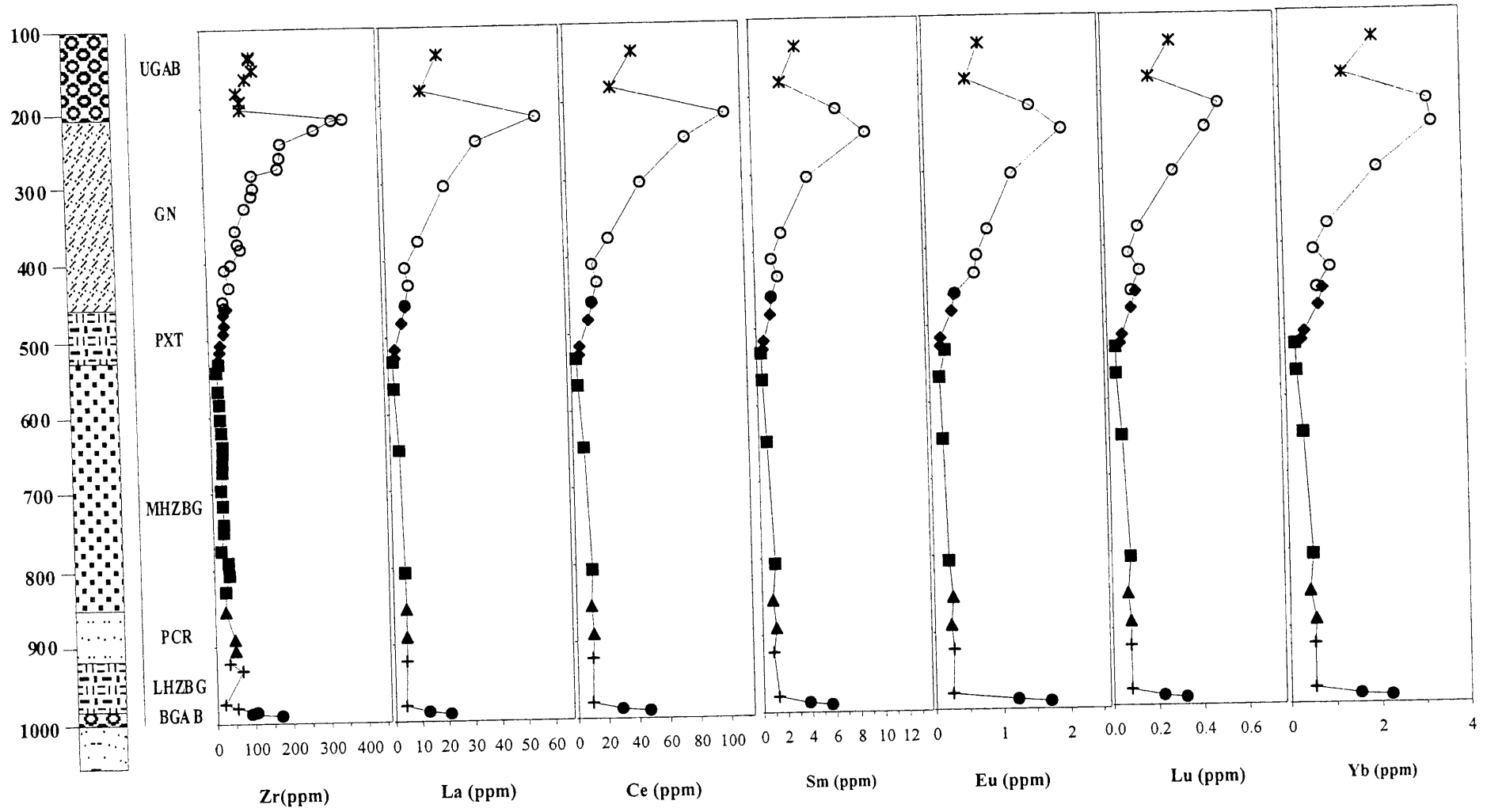
Fig.4.7. (b) Variation diagrams for selected trace elements versus stratigraphic height (m).
