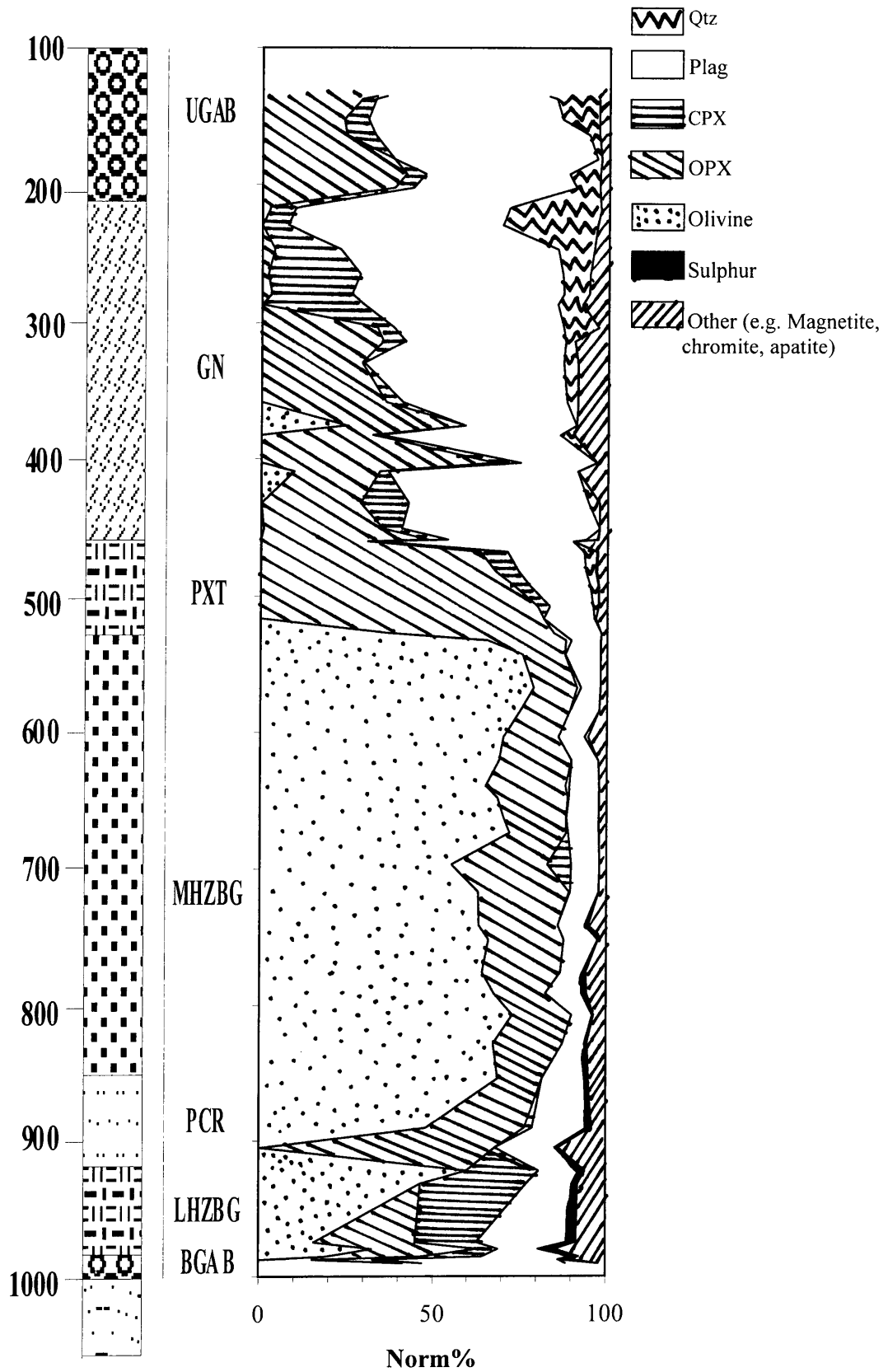
Fig. 4.10. Normalized data including sulphur concentrations Versus stratigraphic height (m)
