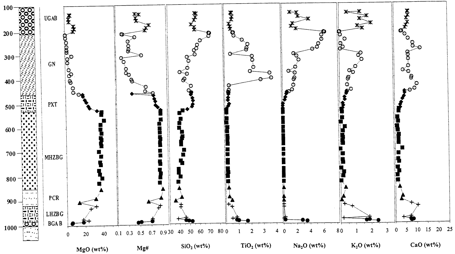
Fig.4.4. Variation of selected major element oxides and Mg# with stratigraphic height (m).
