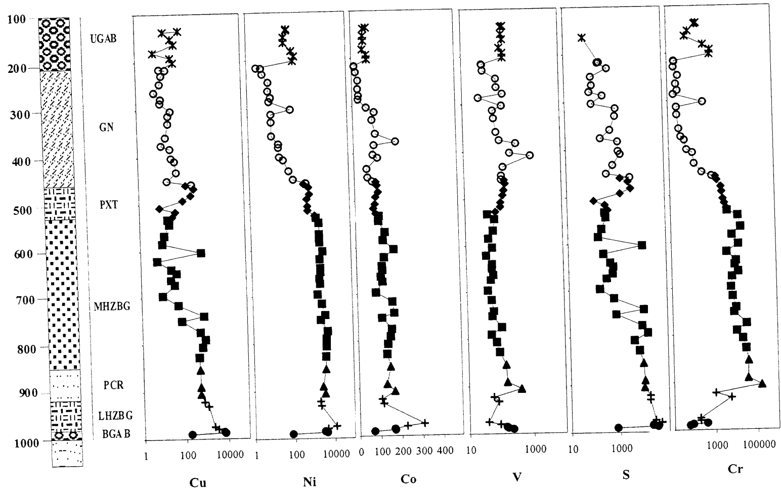
Fig.4.7(c) Variation diagrams for selected trace elements (ppm) versus stratigraphic height (m).
