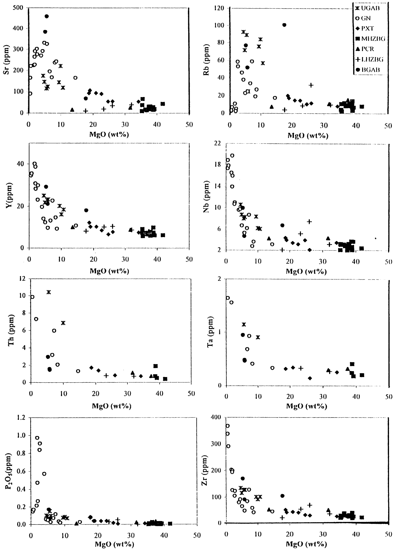
Fig.4.5.(a) Variation diagrams for selected trace elements versus MgO.
