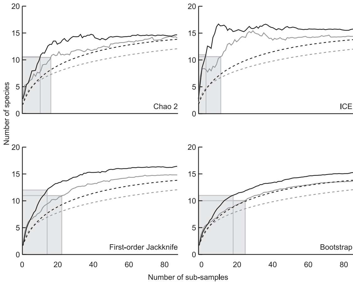
Figure 3. Estimator-based (solid line) and randomised (dashed line) species accumulation curves for near-natural (black) and managed (grey) beech forests obtained with incidence-based coverage (ICE), Chao 2, first-order Jackknife (Jack 1) and bootstrap richness estimators. Shadowed areas correspond to the 75% expected diversity cut-off. doi:10.1371/journal.pone.0023671.g003
