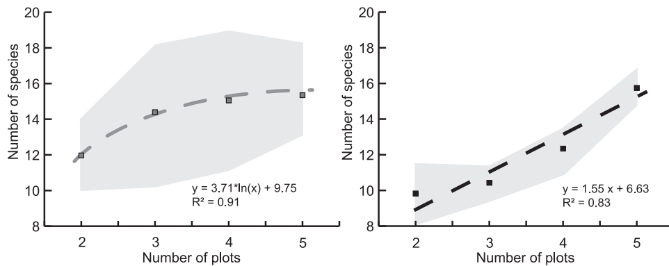
Figure 4. The average estimator based species accumulation curve for one to five plots of near-natural (black) and managed (grey) beech forests. Shadowed areas correspond to the standard deviation. doi:10.1371/journal.pone.0023671.g004
