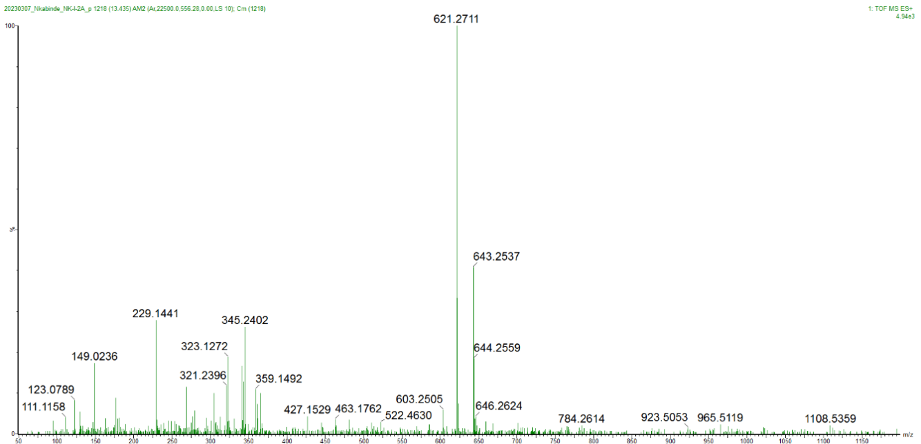
Supplementary Figure 1. Low energy MS spectra of yuanhuacine A (1), analysed in ESI positive ionisation mode.
