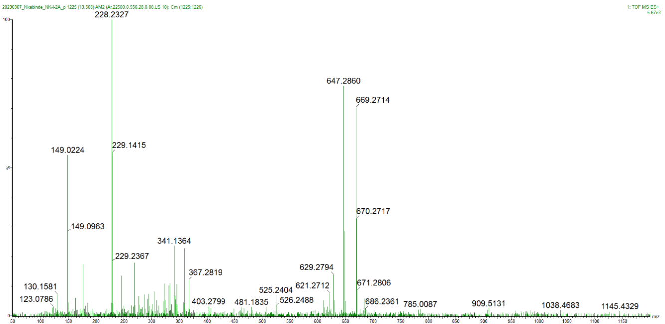
Supplementary Figure 2. Low energy MS spectra of gniditrin (2), analysed in ESI positive ionisation mode.
