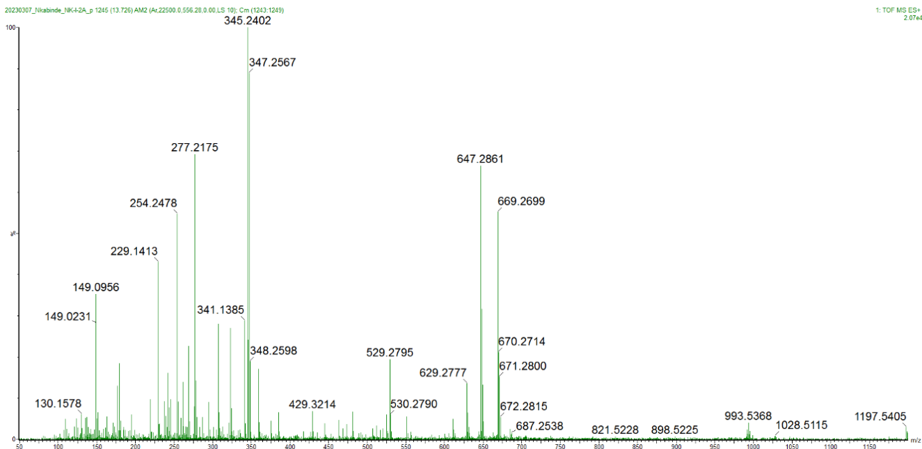
Supplementary Figure 3. Low energy MS spectra of yuanhuajine ( 3 ), analysed in ESI positive ionisation mode.
