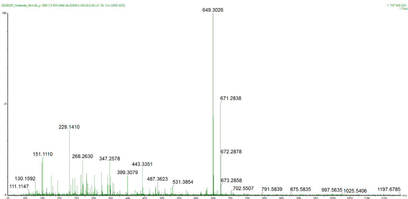
Supplementary Figure 4. Low energy MS spectra of yuanhuacine ( 4 ), analysed in ESI positive ionisation mode.
