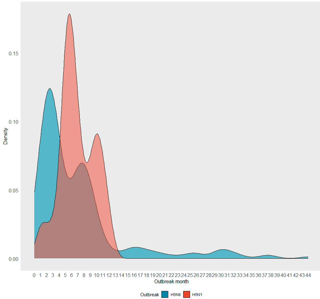
Figure S2. Density plot of HPAI outbreaks in South Africa by month.
