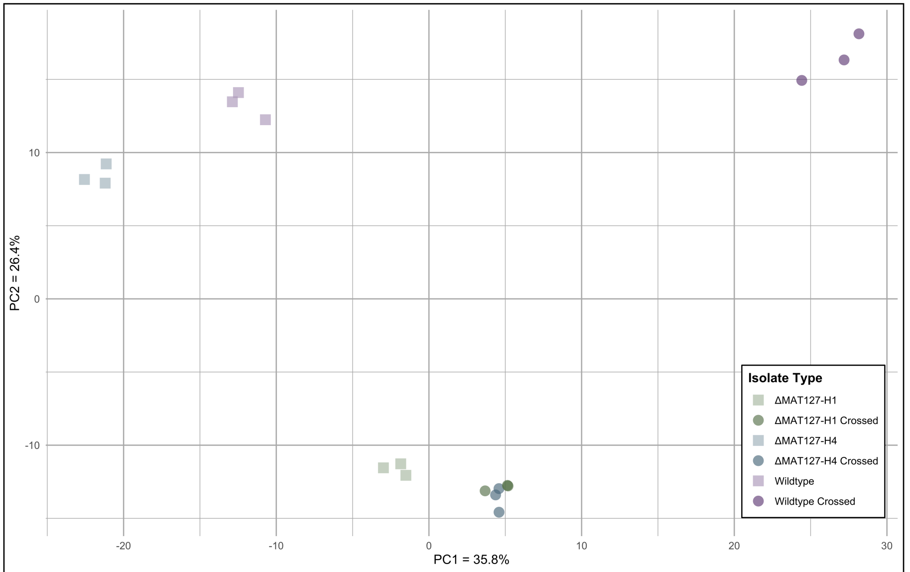
Figure S1: Principal component analysis (PCA) of the technical RNA-seq repeats. The technical repeats of each culture type clustered as expected and a total of 62% of the total variation was explained by the first two components. Square, light-coloured nodes represent the vegetative isolates, while circular, dark-coloured nodes represent the crossed culture types.
