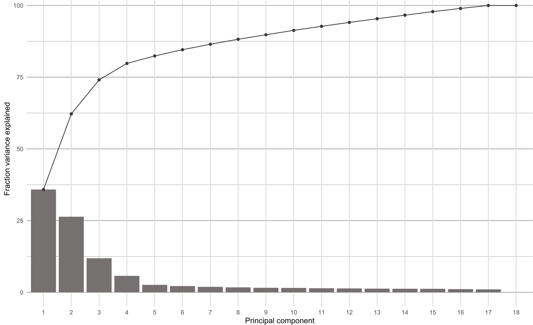
Figure S2. Screen plot from the principal component analysis (PCA). Almost 36% of the variance is explained by the first component and a further 26% is explained by the second component.
