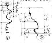
MOULDING DETAILS.
