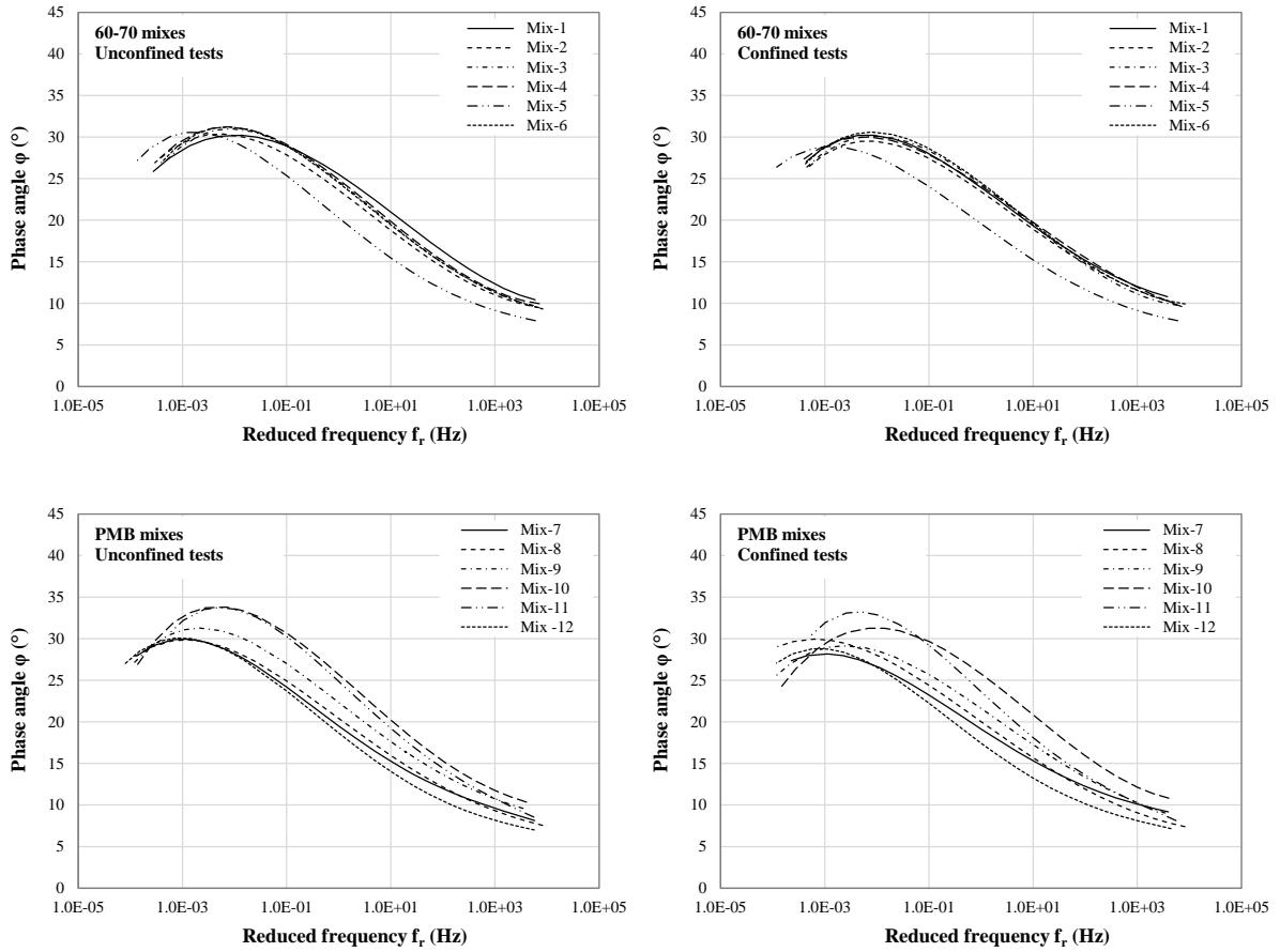
Figure 3. Phase angle master curves of the asphalt mixes (at 20 °C)
