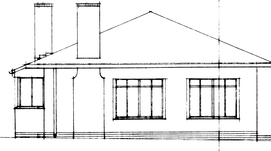
EAST ELEVATION
