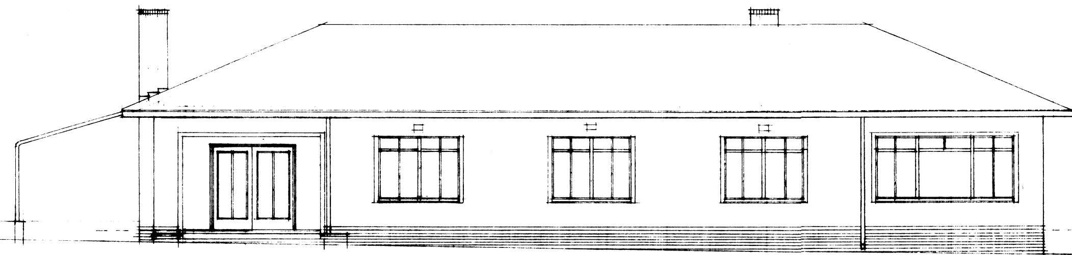
NORTH ELEVATION
