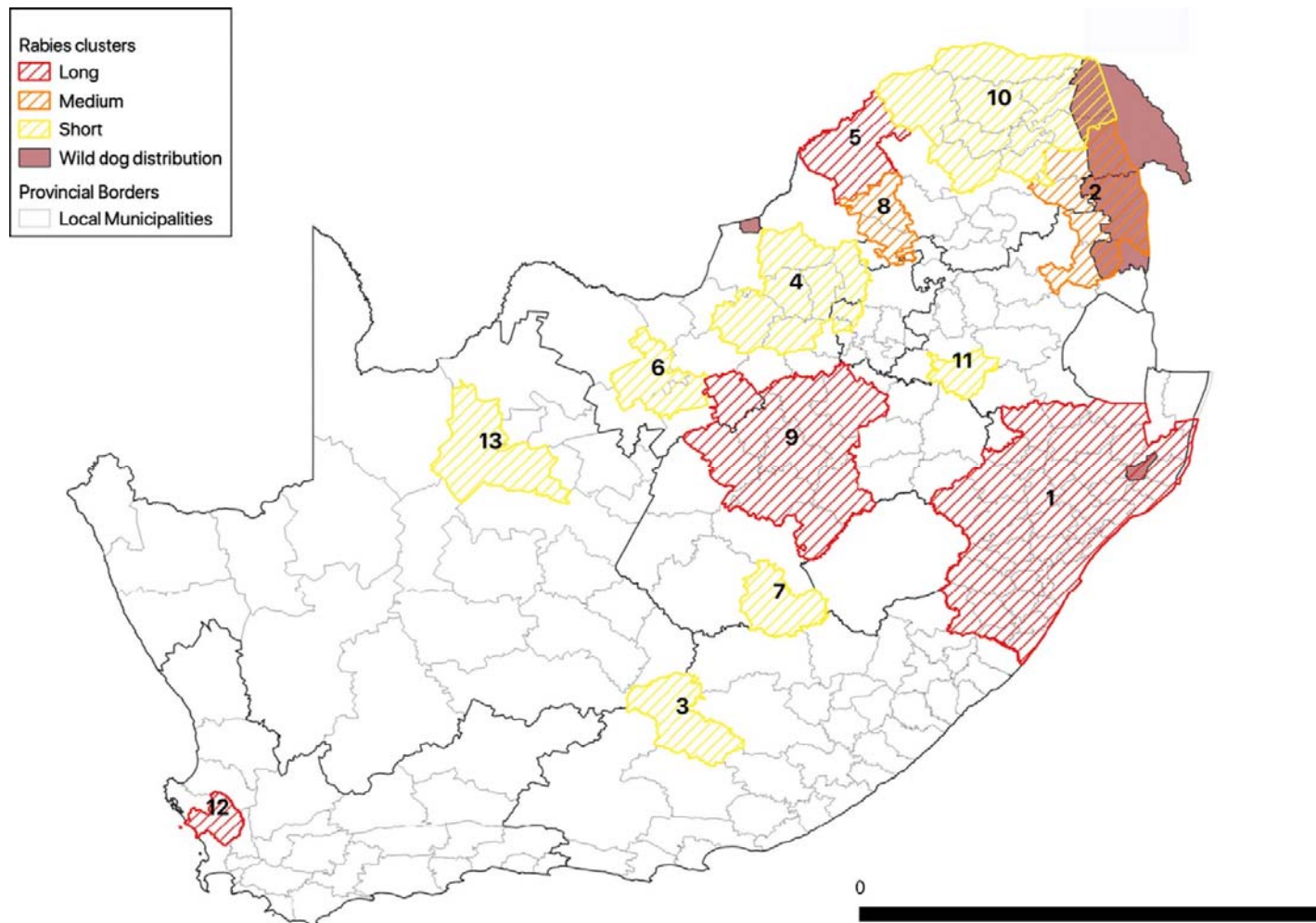
FIGURE 5. Spatio-temporal cluster analysis of rabies outbreaks in South Africa from 1993 to 2019 showing 13 significant clusters. The temporal length of the clusters is indicated by colour: yellow (short), orange (medium) and red (long). For details of each cluster refer to Table 2. (The map was constructed using QGIS 3.4 using country and municipal boundaries and wild dog distribution with permission from IUCN red data list https://www.iucnredlist.org (Woodroffe & Sillero-Zubiri, 2012))
