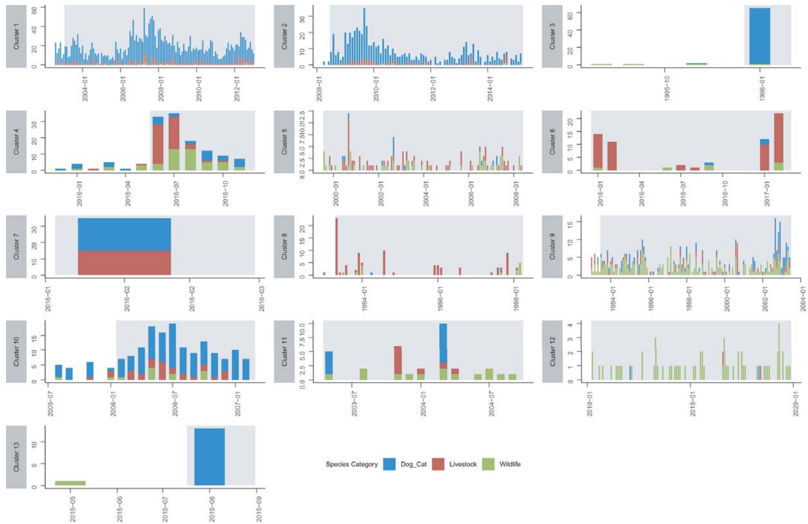
FIGURE 6. Analysis of rabies clusters in South Africa by species composition from 1993 to 2019. Clusters are shown in grey and any cases within six months prior to cluster in the same geographic area are also shown
