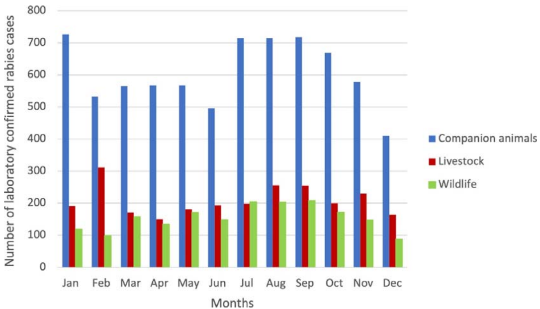
FIGURE 4. Monthly cumulative number of confirmed cases of rabies in companion animals, livestock and wildlife in South Africa from 1993 to 2019
