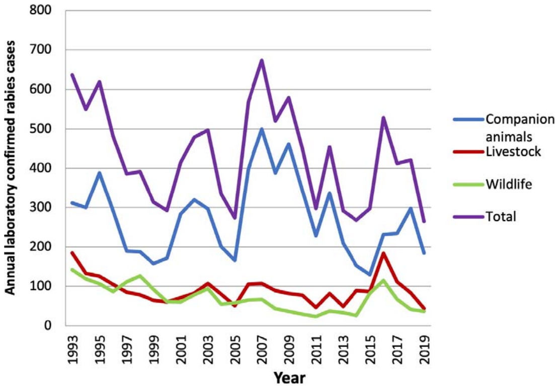
FIGURE 3. Annual confirmed rabies cases in companion animals, livestock and wildlife in South Africa from 1993 to 2019
