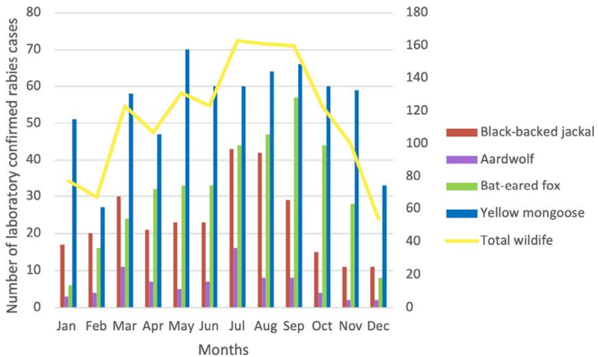
FIGURE 9. Number of confirmed cases of rabies in black-backed jackal, aardwolf, bat-eared fox and yellow mongoose in South Africa from 1993 to 2019, by month. Total wildlife case numbers are shown in right axis
