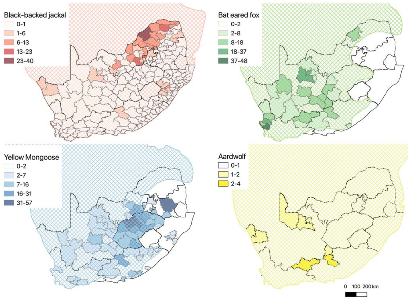
FIGURE 7. Distribution of number of rabies cases reported in wildlife in South Africa, 1993–2019, by local municipality showing the species distribution in chequered colour (Do Linh San et al., 2015; Green, 2015; Hoffmann, 2014a, 2014b) (The map was constructed using QGIS 3.4 using country and provincial boundaries and species distribution with permission from IUCN red data list https://www.iucnredlist.org )
