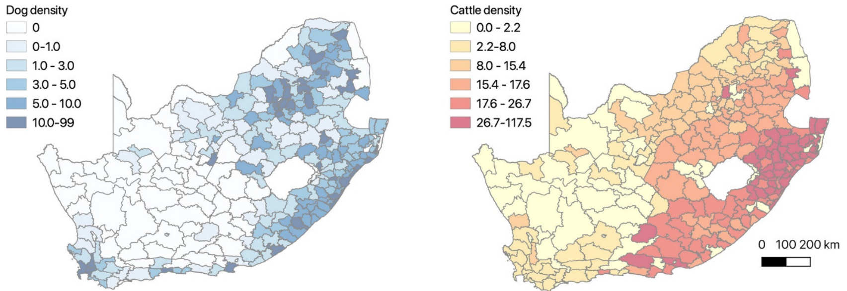
FIGURE 1. Estimated density of dogs and cattle per km 2 in South Africa based on the 2011 human population census and gridded livestock of the world 2010 (Gilbert et al., 2010; Statistics South Africa, 2012). (The map was constructed using QGIS 3.4 using country and municipal boundaries)
