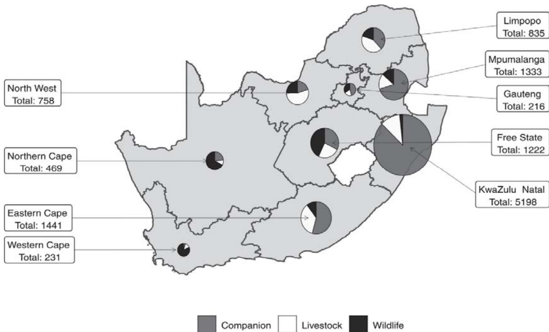
FIGURE 2. Map of rabies cases in South Africa 1993–2019 showing species categories involved by province. The diameter of the pie chart is proportional to the number of reported cases. (The map was constructed using RStudio version 1.0.153 using provincial boundaries)
