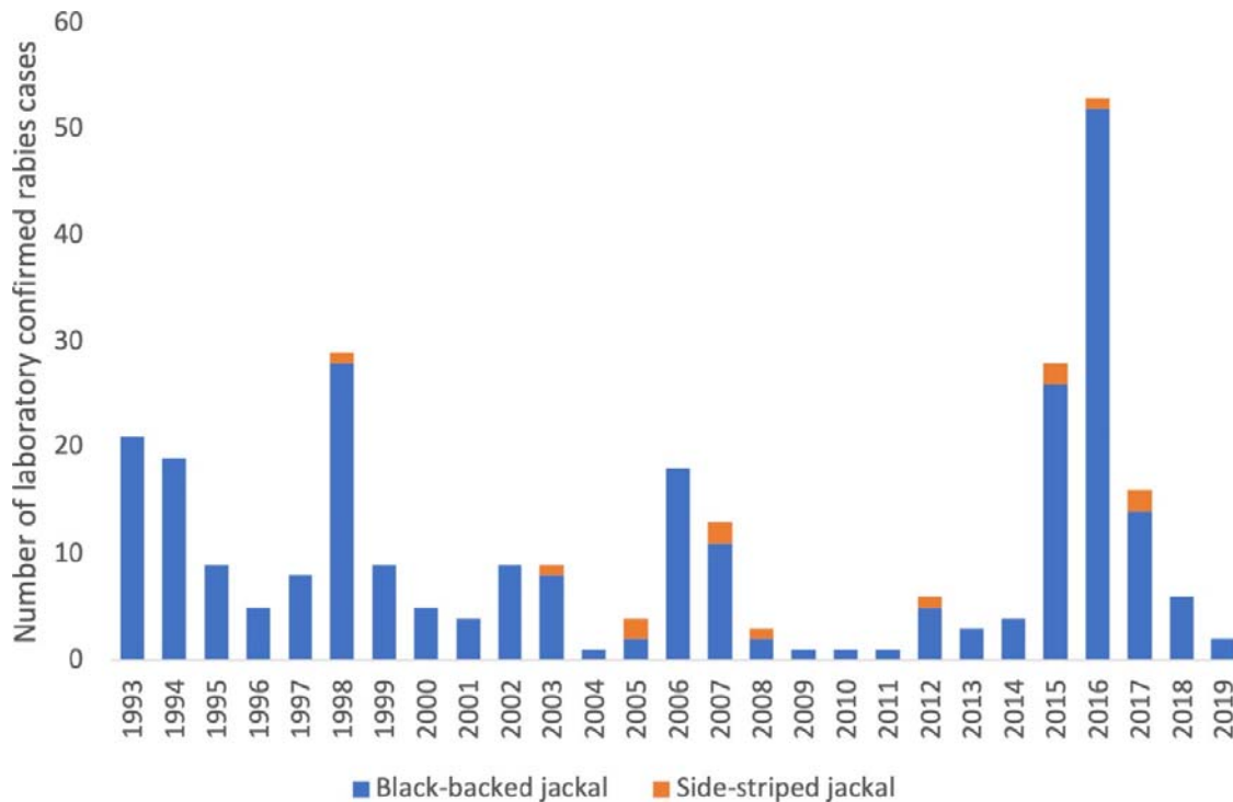
FIGURE 8. Number of rabies cases reported per year in jackals in South Africa from 1993 to 2019
