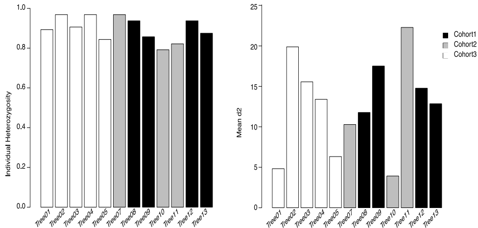
Figure SF4: Measure of individual heterozygosity, H , (left) and d^2 (right) by cohort assignment
