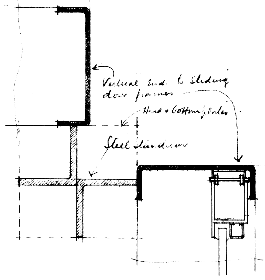
VERTICAL SECTION & CORNER PLAN DETAILS OF SLIDING DOORS TO 1/2 FULL SIZE SCALE
