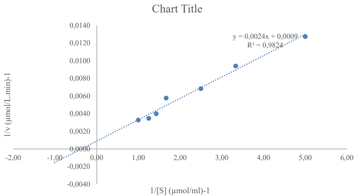
Figure S2: Kinetic plot showing the catalytic behaviour of HRJ16 laccase on ABTS
