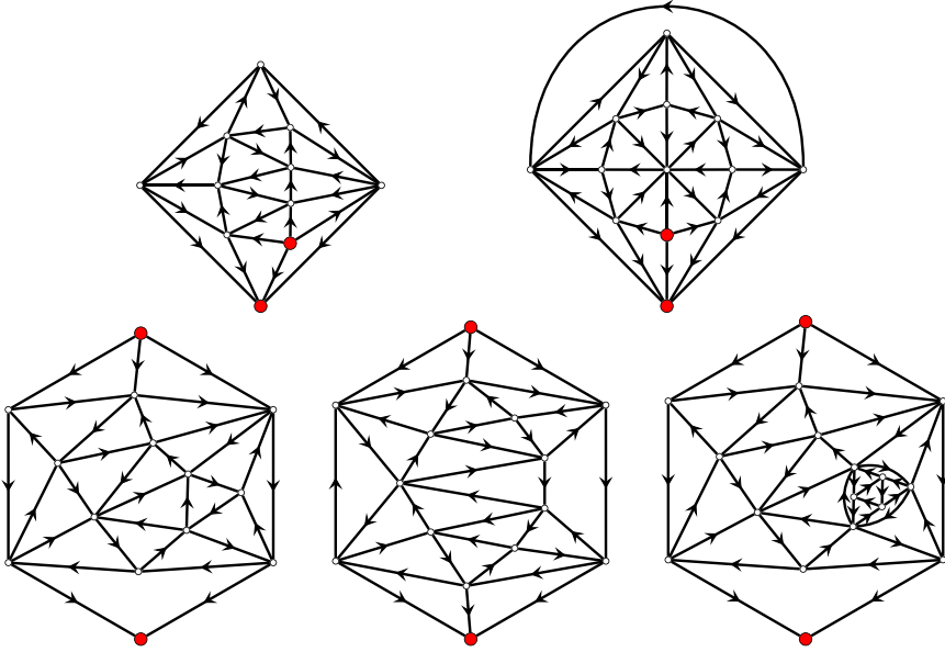
FIGURE 6 Planar hypotractable oriented graphs of order 11, 13, 14, 15 and 17 as required in the proof of Theorem 16. In each the sink and source are emphasised
