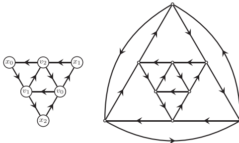
FIGURE 3 Left-hand side: The digraph Z_6 . Right-hand side: The smallest planar hypohamiltonian oriented graph
