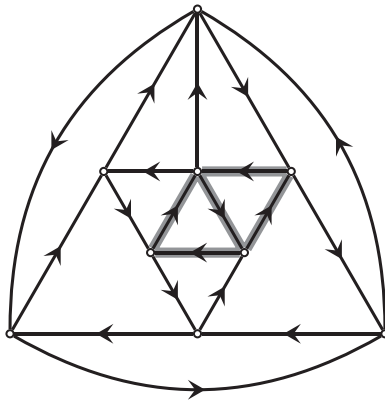
FIGURE 4 One of the two smallest almost arc-minimal planar hypohamiltonian oriented graphs. Together with the highlighted \theta -subdigraph this forms the basis for an infinite family of almost arc-minimal planar hypohamiltonian oriented graphs
