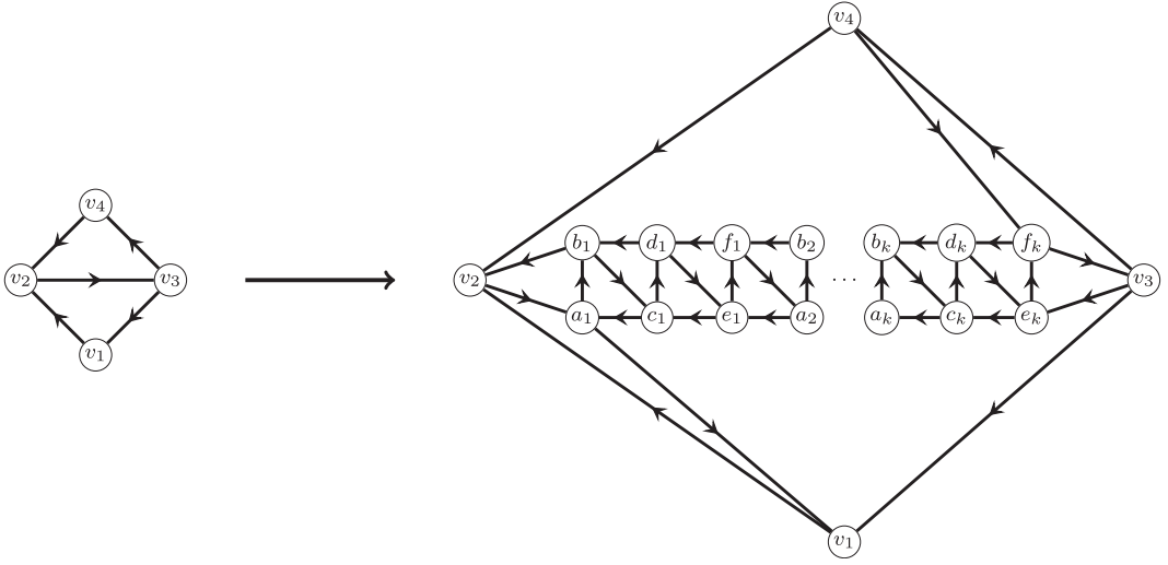
FIGURE 1 Replacing \theta with T_k(\theta)
