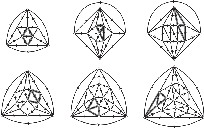
FIGURE 2 The planar hypohamiltonian oriented graphs of order 9, 11, 12, 13, 14 and 16 used in the proof of Theorem 8. The required \theta -subdigraphs are shown in bold
