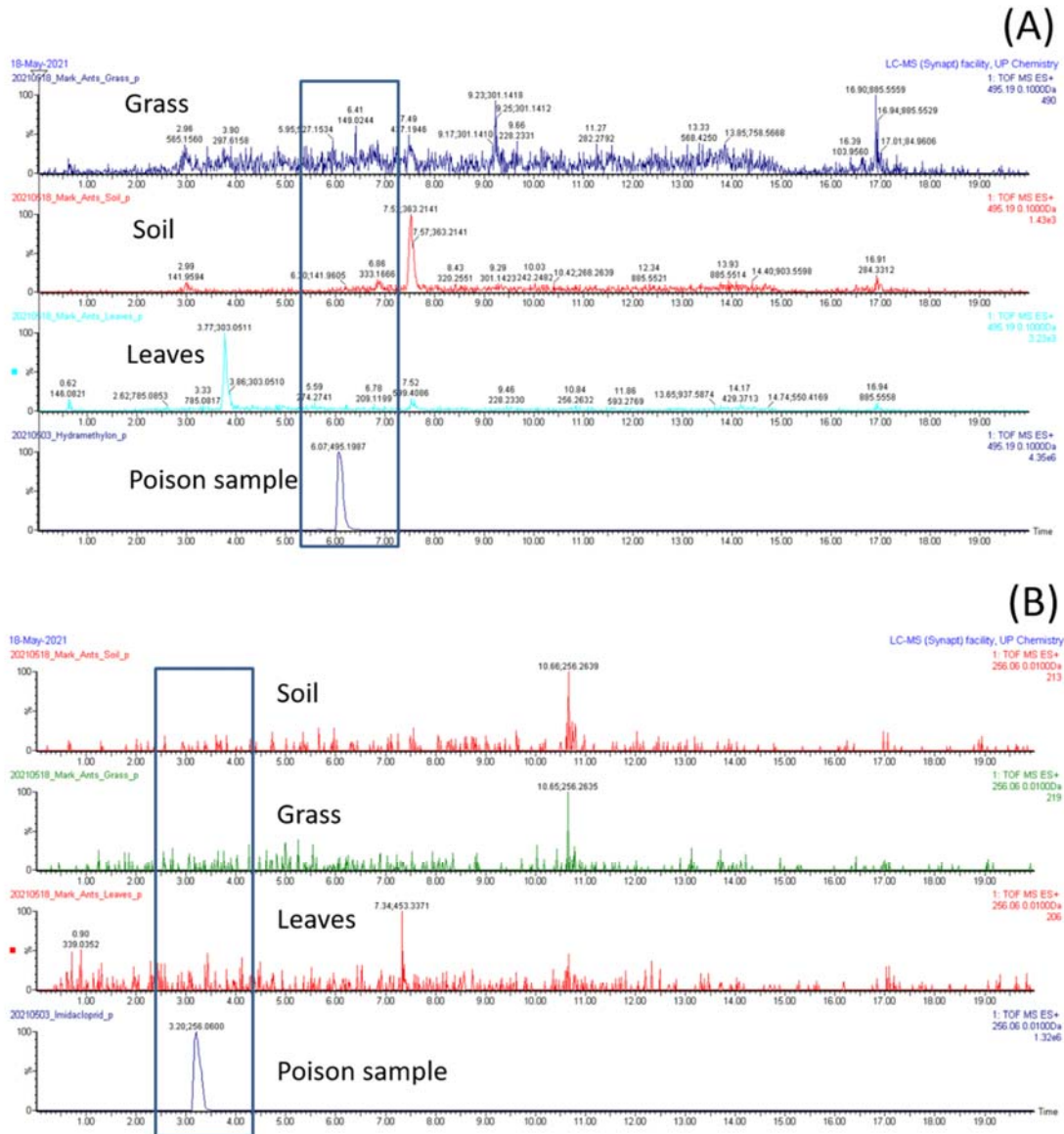
Figure S3. Results of liquid chromatography-mass spectrometry (LCMS) analysis of soil, grass and tree leaves ( Terminalia sericea ) demonstrating no detection of residual hydramethylnon (A) or imidacloprid (B) in the samples. The samples were collected between 8 – 14 th March 2021, 2.5 years into the suppression experiment.
