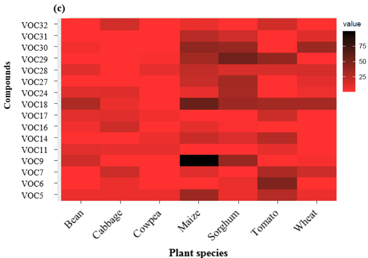
Figure 8. Random Forest (RF) analysis of volatile profiles from different host plants. (a) The most discriminant plant volatiles are listed based on mean decrease in accuracy (MDA) following RF analysis. (b) sPLS-DA biplot showing the correlation of the most discriminant volatiles in the plant species. (d) Heatmap clustering showing the mean abundance of the most discriminant volatile compounds from crop species.
