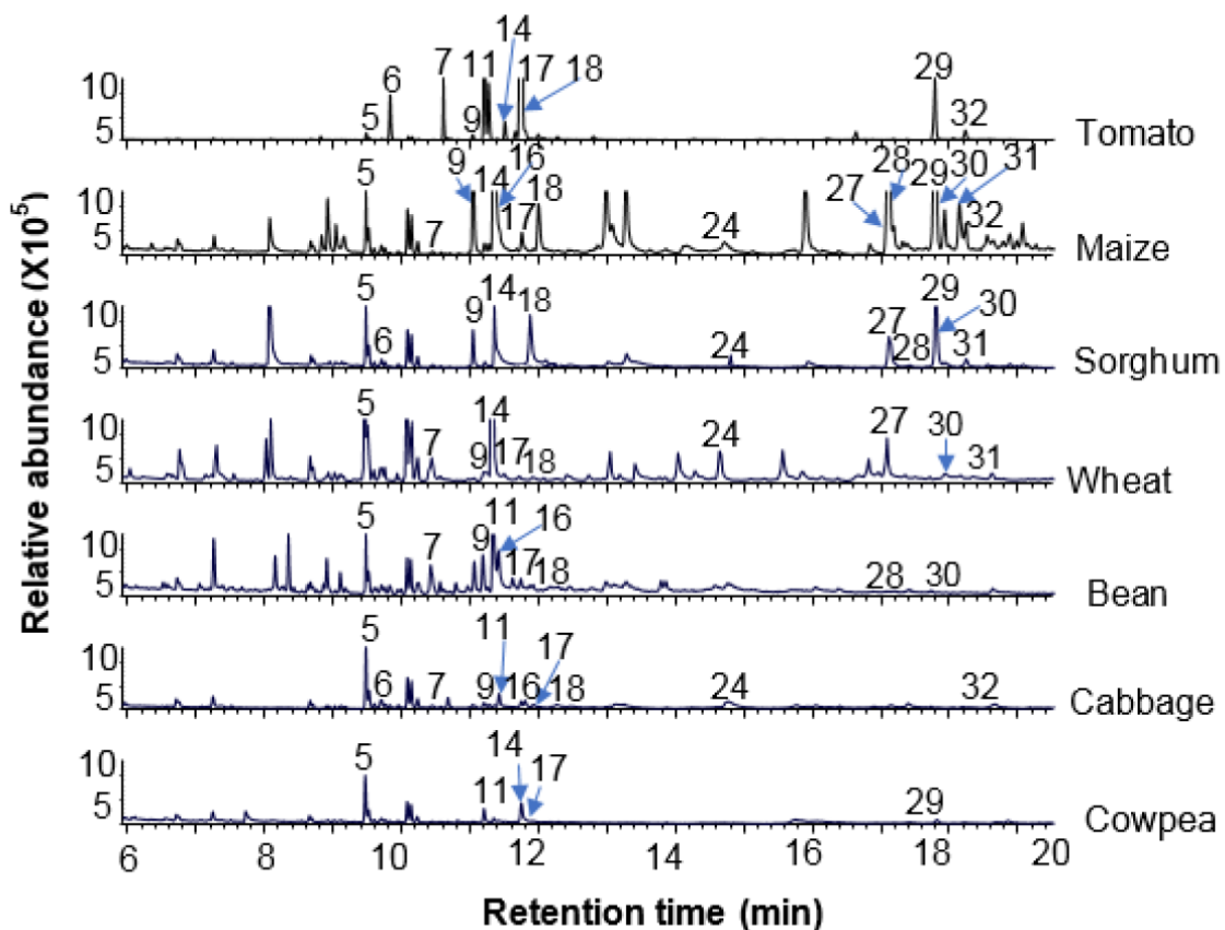
Figure 7. Gas chromatography mass spectrometry (GC-MS) chromatograms of plant volatiles. The peaks of the most discriminant plant compounds are indicated in numbers. Numbers corresponding to volatile compounds are indicated in Table 2.
