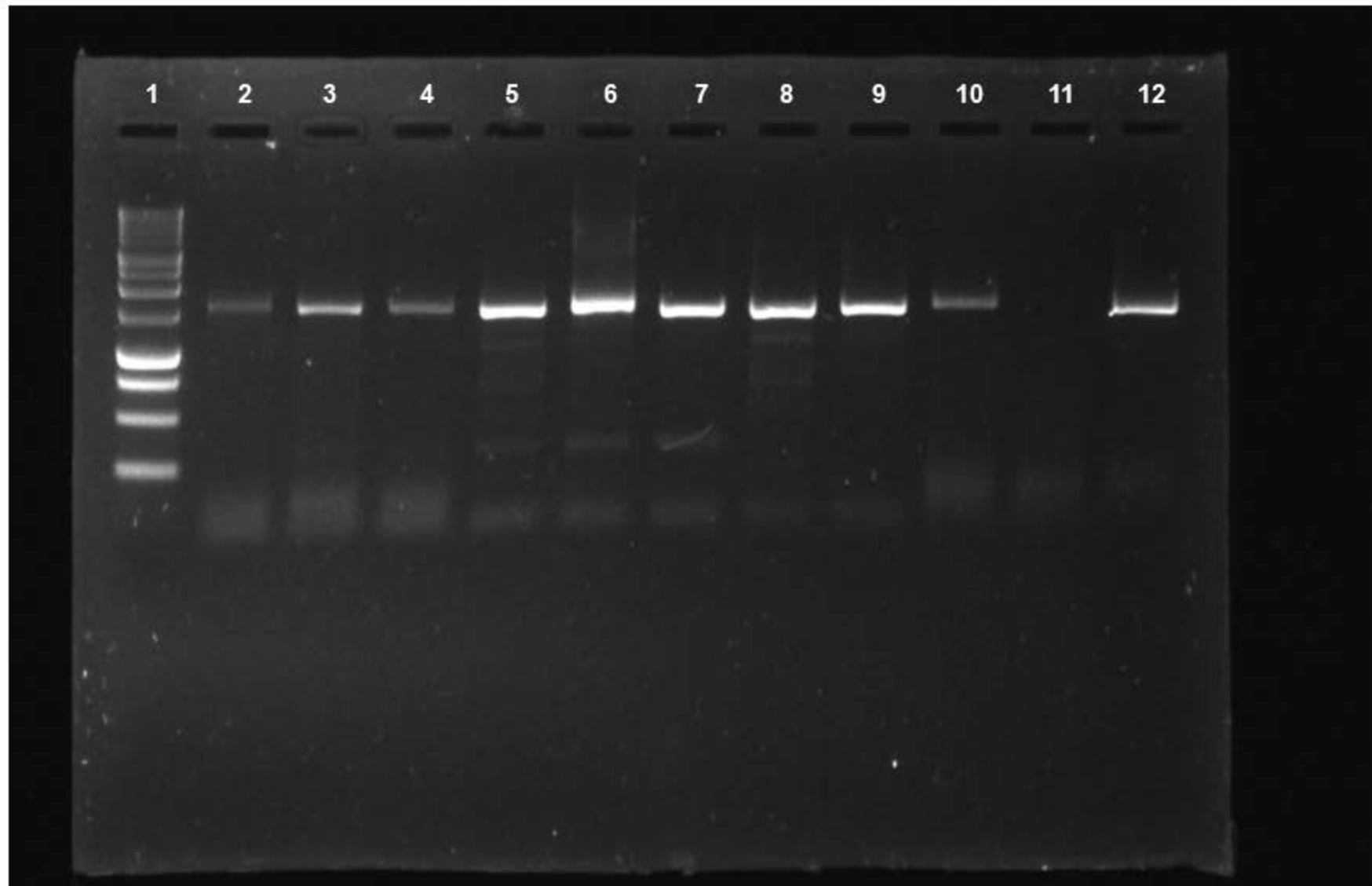
Fig 6: Gel electrophoresis image of Anaplasma PCR targeting the 16S rRNA gene from blood samples. Image taken under UV transillumination using Enduro™ GDS gel documentation system. Lane 1 = 1 kb DNA ladder; 2 - 10 = Anaplasma positive samples; 11 = nuclease free H 2 O (-ve); 12 = A. marginale (+ve).
