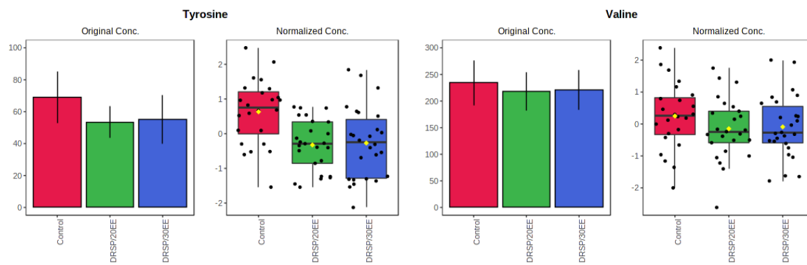
Fig S3: Boxplots representing the compounds detected via the amino acid method
