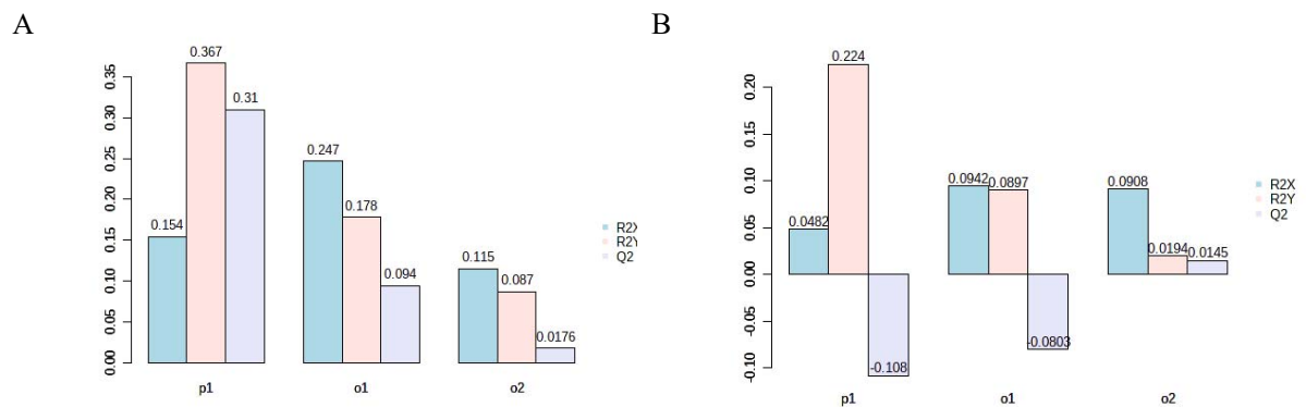
Fig S2: OPLS-DA classification performance. A = Amino acid data; B = Acylcarnitine data
