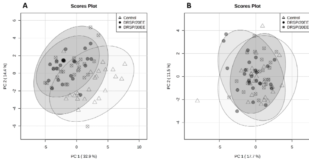
Fig S1: PCA scores plots for the two datasets investigated, with the variation explained indicated in parentheses. A = Amino acid data; B = Acylcarnitine data
