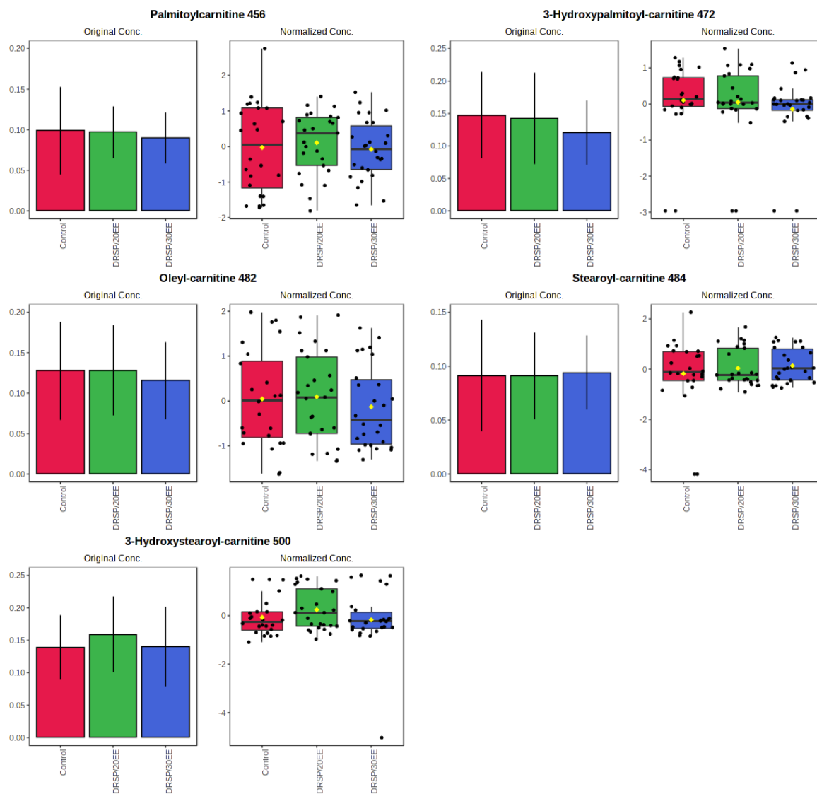
Fig S4: Boxplots representing the compounds detected via the acylcarnitine method
