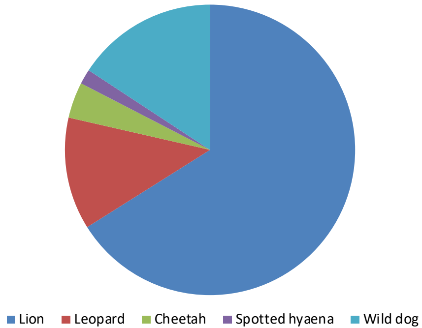
Figure S1: Proportion of herbivore carcasses (of the herbivore species included in this analysis) attributed to each of the five large predators in HIP between 1983 and 2010. All five predator species have remained present in the park since 2010, but the leopard population has reduced considerably, the spotted hyena population has decreased by two thirds, and the lion and wild dog populations have increased, suggesting that the proportion of kills made by leopards and spotted hyena during our study in 2014 would likely be substantially lower than the proportion represented here. Cheetah have remained present at low densities (estimated at six individuals in 2014). Data were sourced from Somers et al. (2017).
