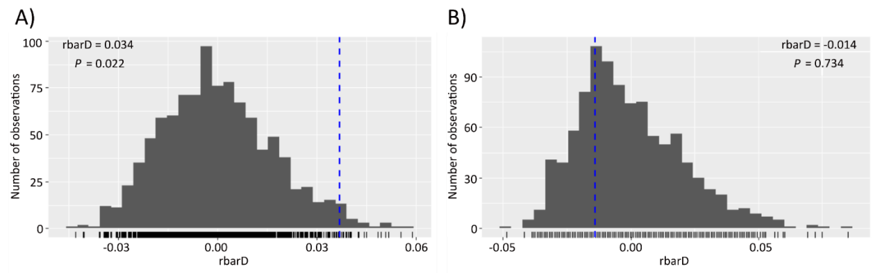
FIGURE S2. Histograms of the linkage disequilibrium tests (rBarD, P-values > 0.01) for the full (A) and clone-corrected dataset (B) of Teratosphaeria destructans isolates from Malaysia. The blue dashed line represents the value of rBarD and provides evidence of random mating.
