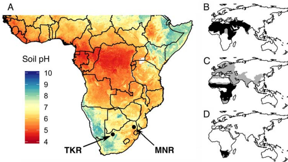
Figure 2. A) Map of sub-Saharan Africa showing the location of Tswalu Kalahari Reserve (TKR) and Manyeleti Nature Reserve (MNR). Underlying map is surface soil (0-5cm) pH measured in H 2 O from Hengl et al. (2017). Note: the inorganic fraction of hyaena faeces will only become bioavailable where soil pH <7. Present (black) and present-natural (grey) species range for B) Hyaena spp, C) Crocuta spp and D) Parahyaena spp adapted from PHYLACINE v1.2 (Faurby et al., 2018).
