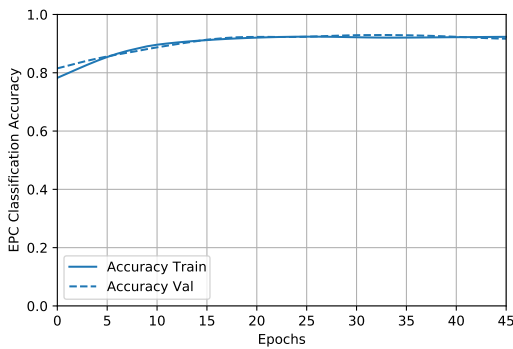
Figure 3: EPC classification accuracy during the ANN model training for Italy's Lombardy region pre-2015.
