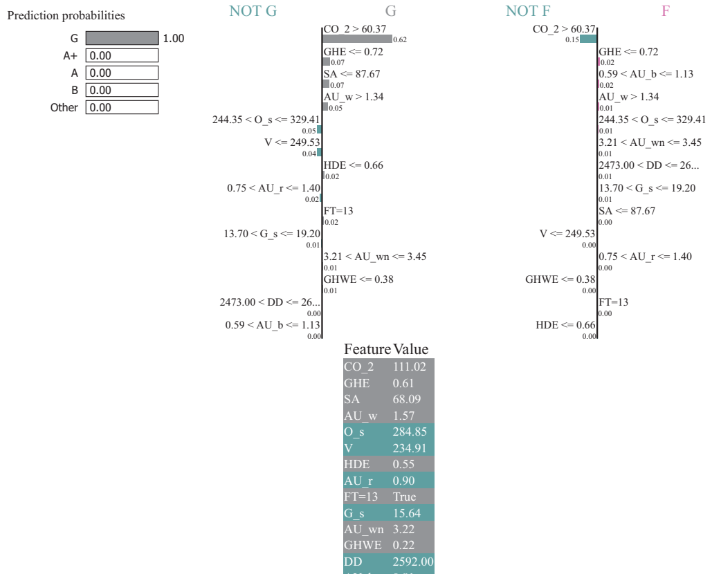
Figure 5: LIME explanations for a building EPC label 'G' classification.
