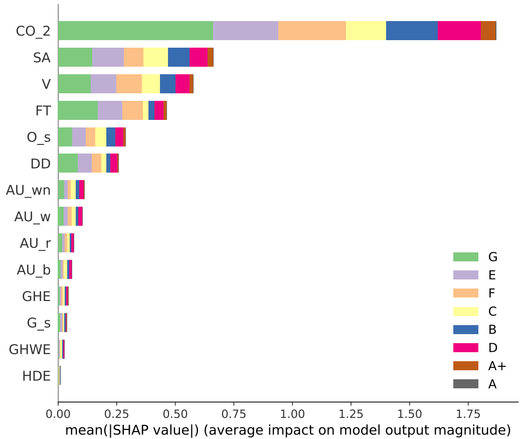
Figure 7: Input feature importance ranking via SHAP global explanations for building EPC classification.
