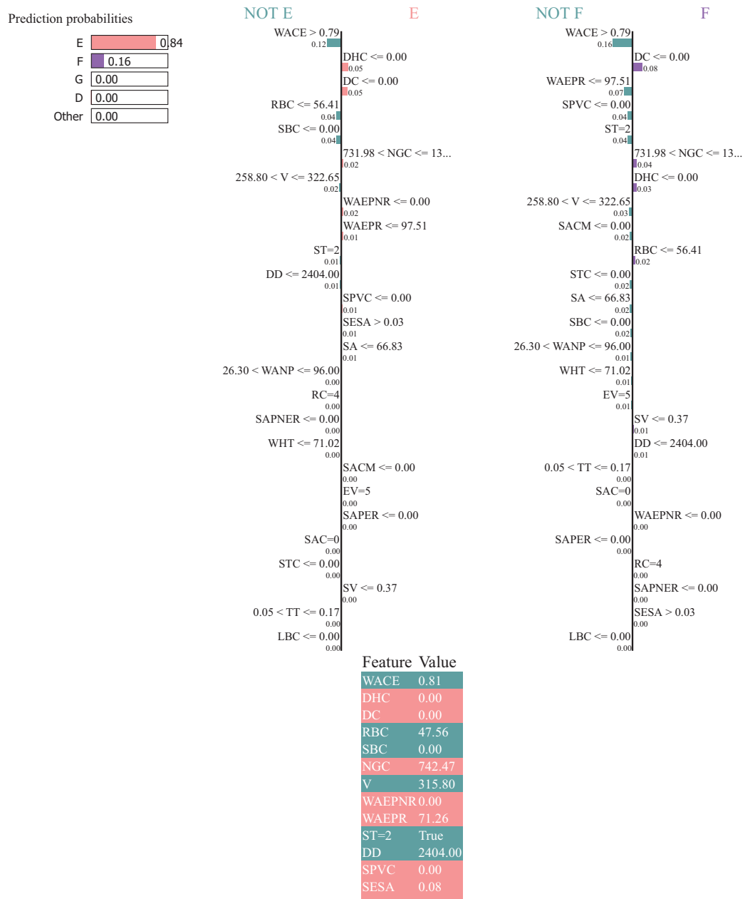
Figure 12: LIME explanations for a building EPC 'E' label classification.
