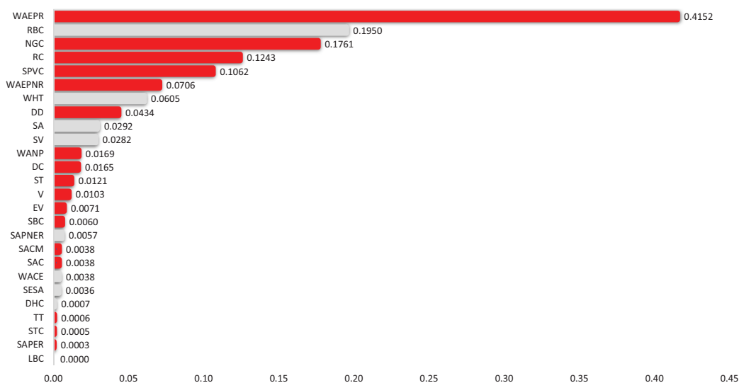
Figure 15: Input feature importance ranking via SHAP explanations for a building EPC E classification.
