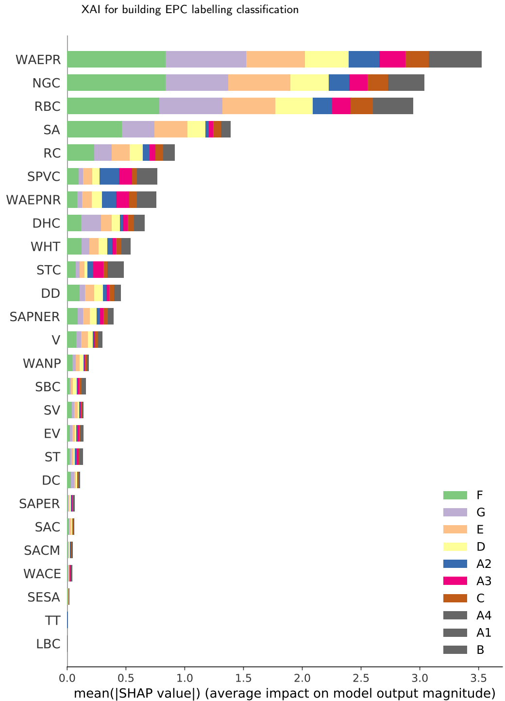
Figure 14: Input feature importance ranking via SHAP global explanations for the building EPC classification.
