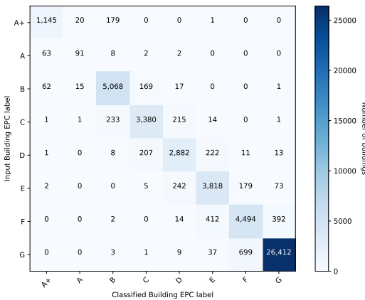
Figure 4: A confusion matrix: input building EPC label vs. classified EPC labels (Case study 1).
