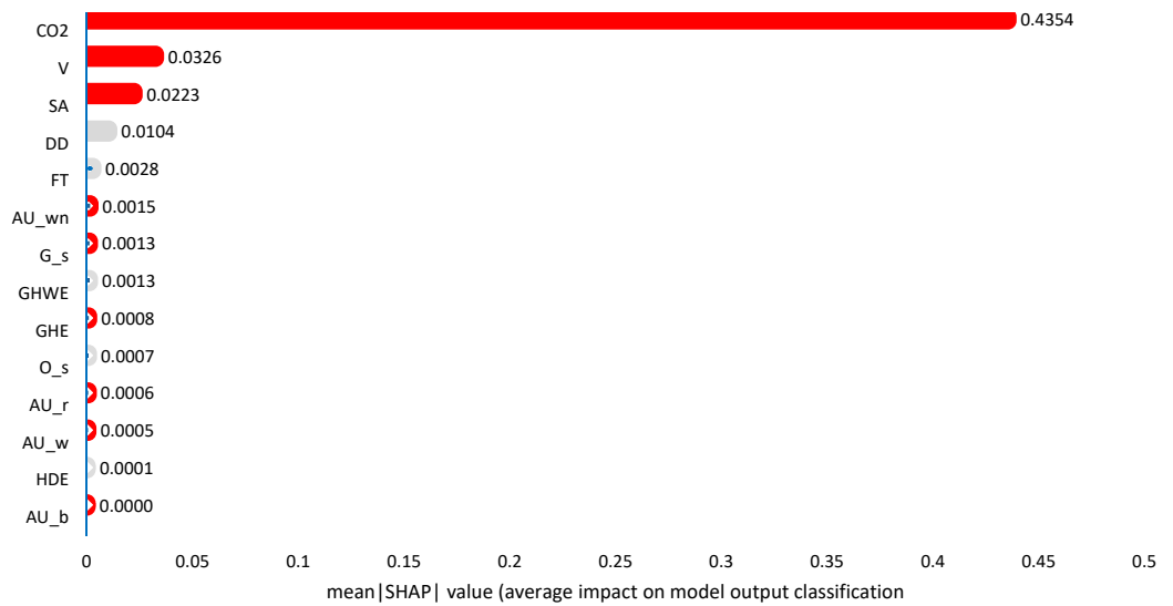
Figure 8: Input feature importance ranking via SHAP explanations for a building EPC G classification.
