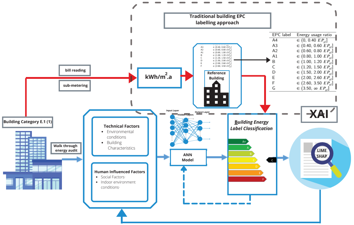
Figure 1: Building EPC ANN classification and explainable artificial intelligence.
