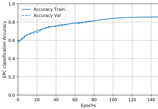
Figure 10: EPC classification accuracy during the ANN model training for Italy’s Lombardy region post-2015.
