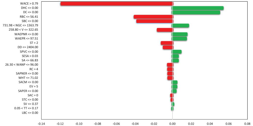
Figure 13: Input feature importance ranking via LIME explanations for a building EPC E classification.
