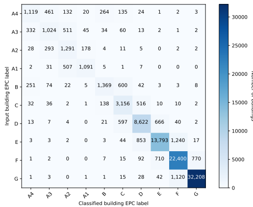
Figure 11: A confusion matrix: input building EPC label vs. classified EPC labels (Case study 2).
