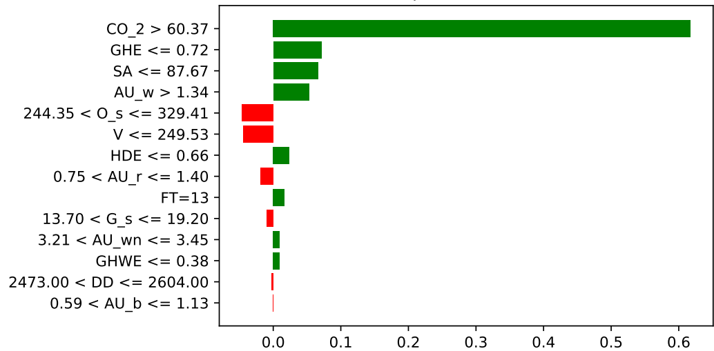
Figure 6: Input feature importance ranking via LIME explanations for a building EPC 'G' classification.
