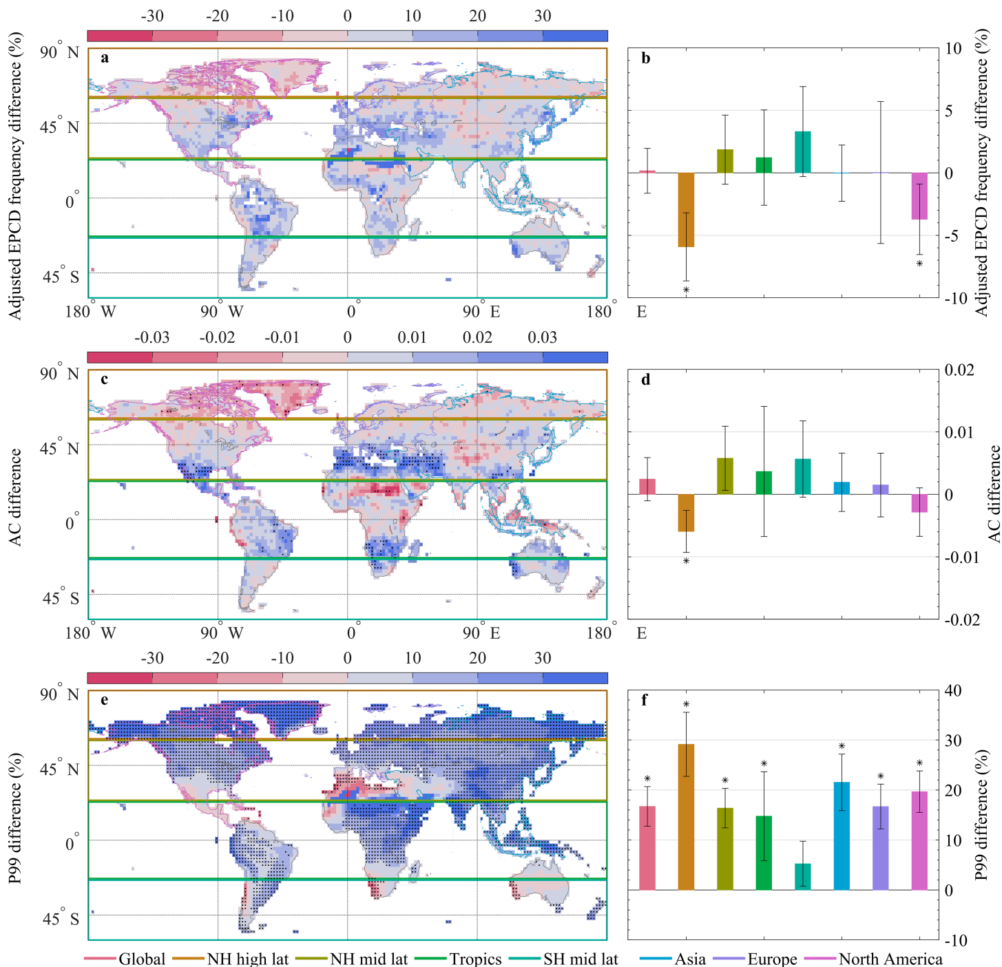
Fig. 4. Changes in adjusted frequency of extreme precipitation on consecutive days, autocorrelation, and precipitation intensity between 1961–2010 and 2071–2100 for historical + RCP8.5 scenario simulations. (a),(b) EPCD frequency changes (%) after removing the effects of possible intensity changes. (c),(d) Changes in autocorrelation in the daily extreme precipitation time series. (e),(f) Changes (%) in daily intensity of precipitation for the 99th percentile of all-day precipitation. Stippling in (a) and asterisks in (b), (d), and (f) indicate “robust change” across all models (see “Materials and methods” section). Stippling in (c) and (e) represents that at least 80% of models agree on the change sign. Error bars in (b), (d), and (f) represent plus and minus one ensemble standard deviation.
