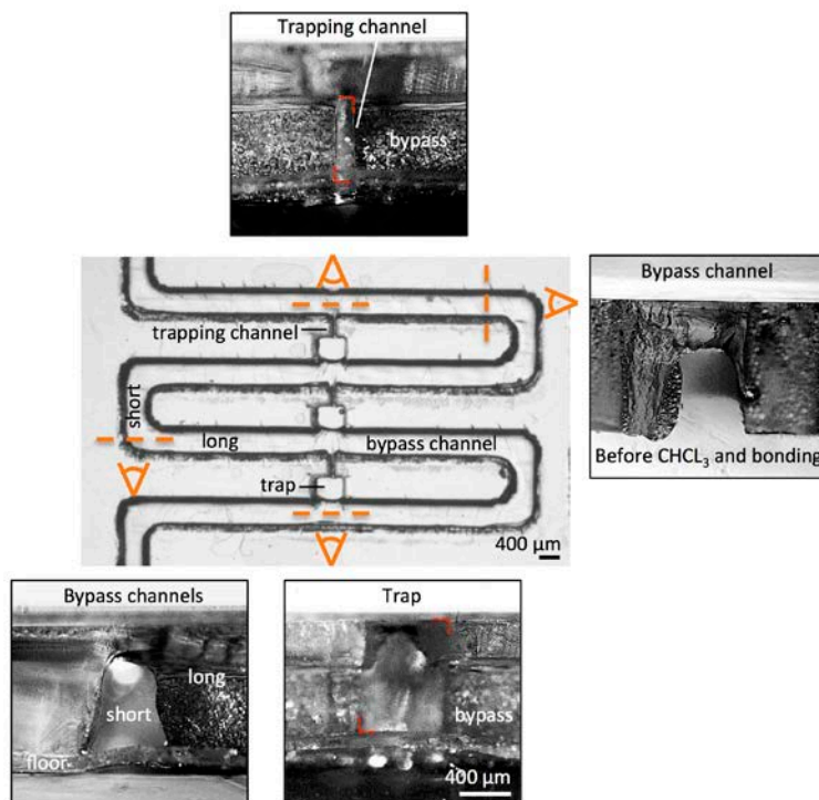
Suppl. Fig. 6. Microfluidic device geometry. Top-view and cross-sectional views of the device after making various breaks to expose the features. Representative locations of the breaks (dotted lines) and point-of-view (eye symbol) are shown. Cross-section of the long portion of the bypass is shown before chloroform ( \text{CHCl}_3 ) treatment and bonding. Other cross-sections are shown after \text{CHCl}_3 treatment and bonding to the floor. Red brackets delineate feature borders for the trap channel and for the trap (transition to trap channel visible inside).
