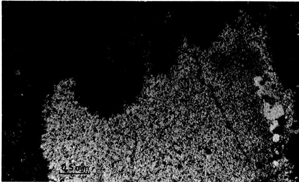
Figure 4: Hornblende (dark) matrix partly replacing a chert pebble (light) in a conglomerate (AK319, RC, Bevet's Conglomerate Member, southeast of Dinokana, polarized light).
