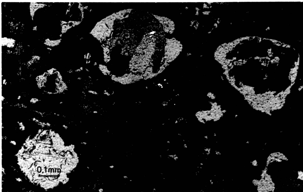
Figure 12: Nodular structures containing biotite, muscovite (m) and a clear rim of quartz in a groundmass of sericite and quartz (AK92, SS, Strubenkop Shale Formation, Rietgat 91JP, polarized light).
