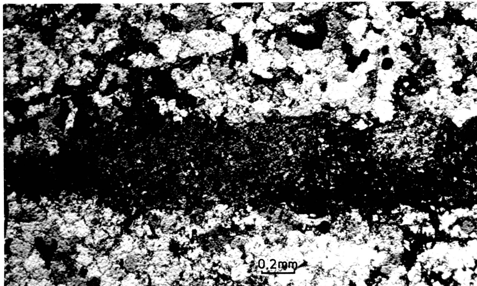
Figure 19 : Aggregate pseudomorphs of andalusite (A) after chloritoid (dark) in a hornfels lamina in quartzite (AK29, TL, Timeball Hill Formation, Buffelfontein 94JP, polarized light).
