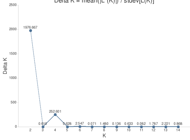
Delta K = \text{mean}(|L''(K)|) / \text{stdev}[L(K)]
