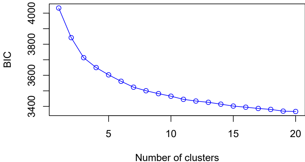
Value of BIC versus number of clusters
