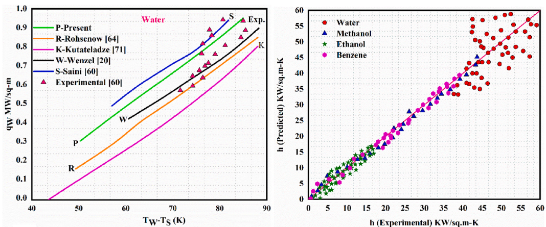
Fig. 3. Comparison of (a) heat transfer correlations; (b) experimental and predicted 'h' values.
