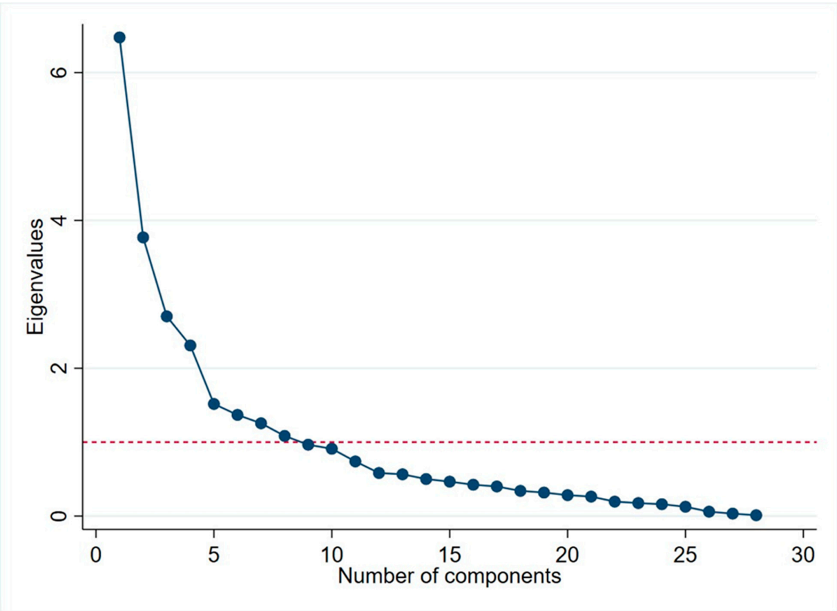
Figure S1. Screeplot for the principal component analysis of nutrients.
