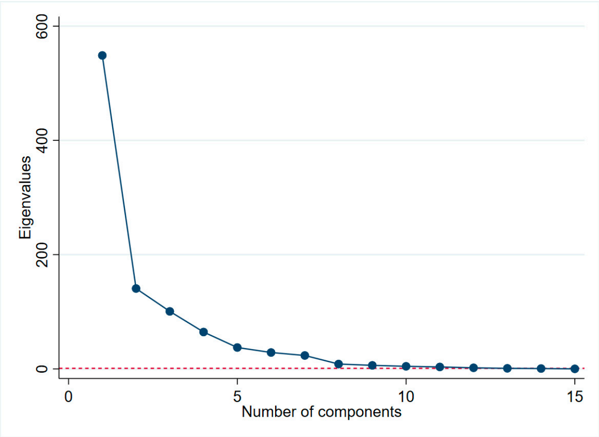
Figure S2. Screeplot for the principal component analysis of food items.
