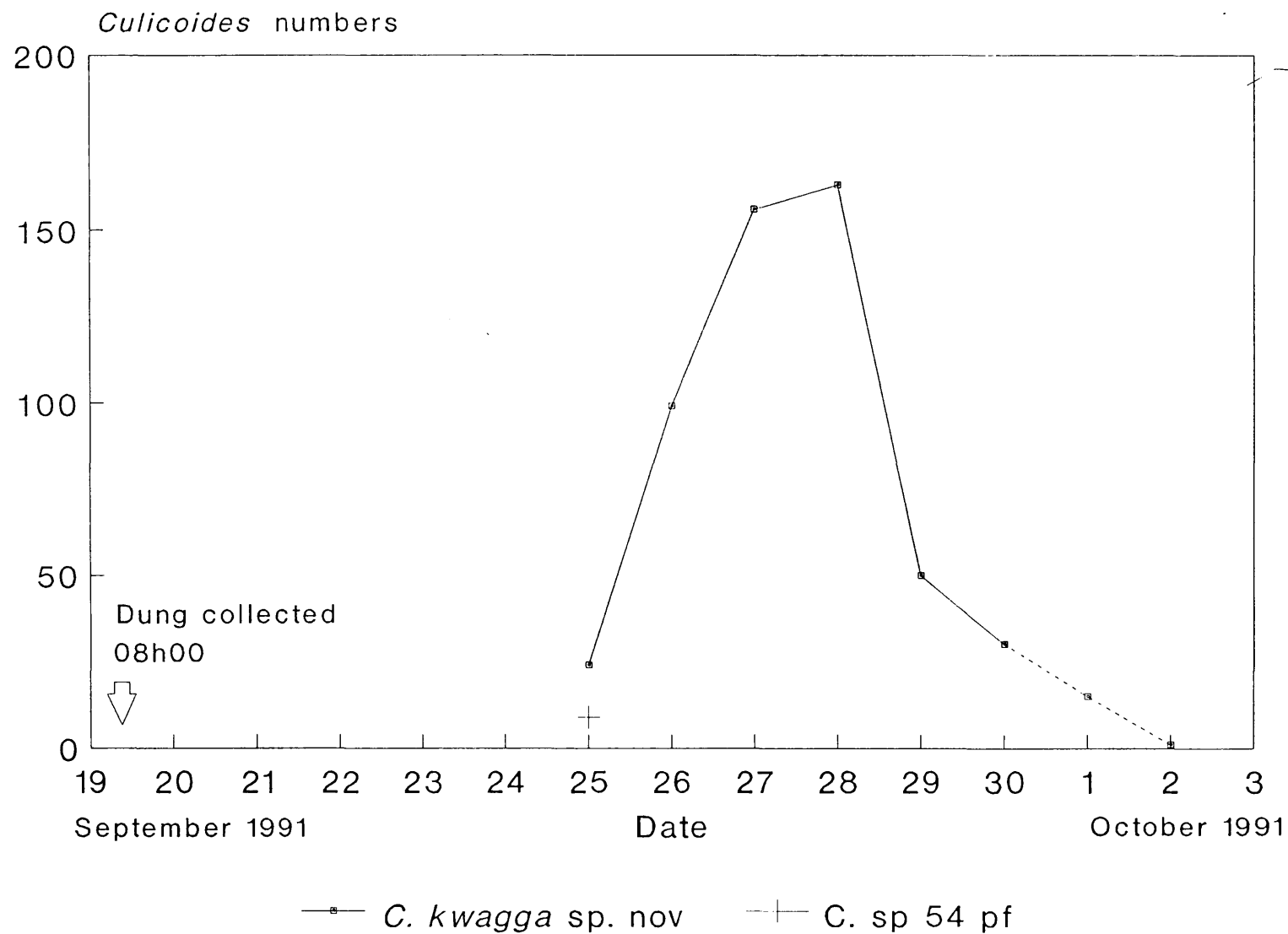
FIG. 7.6 Numbers of two Culicoides spp. reared from 4,5 kg of zebra dung collected on 19/9/1991 at Ngirivane 12 km w. of Satara (central KNP); dung a few hours to 1,5 days old. Collection no. KNP 91.27.
