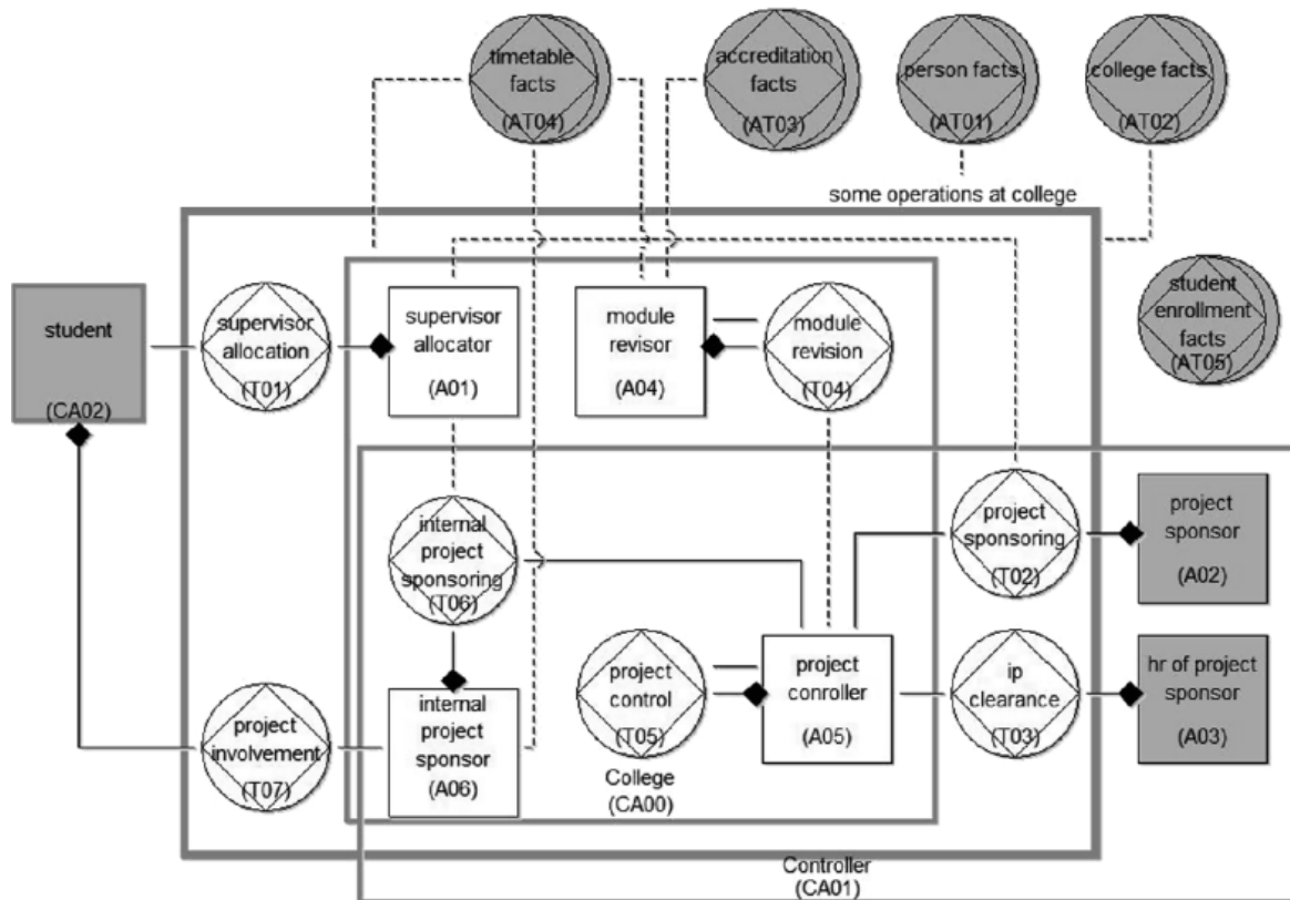
Fig. 4. The OCD for a college, based on [19]
