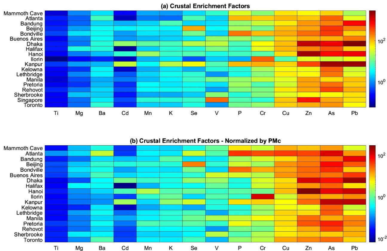
Figure 2. (a) Crustal enrichment factors (EF) for PM 2.5 relative to crustal ratios of the given element and iron (Eq. 1), and (b) replacing measured iron with measured PM c (Eq. 2). Elements are sorted by mean enrichment factor across all sites; sites are listed alphabetically. Singapore is not shown in the bottom plot due to unavailable PM c data.
