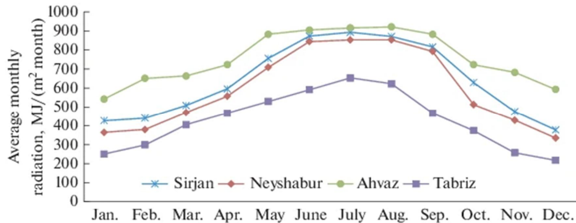
Fig. 2. Average monthly radiation for four cities.
