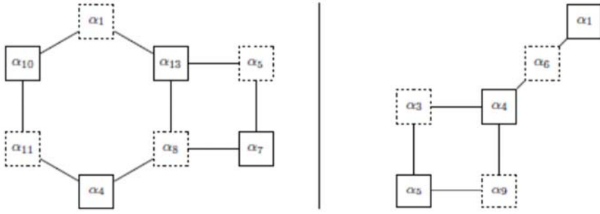
FIGURE 1. Two examples of graphs as described above in the case G = F_4(2^f) . On the left, \mathcal{S} and \mathcal{Z} correspond to the [4, 12, 9] -core associated to \mathcal{F}_{7,1} . On the right, \mathcal{S} and \mathcal{Z} are taken with respect to the only [5, 11, 6] -core; here |\mathcal{T}| = 1 , and \Delta \in \mathcal{T} is the graph with edges \{\alpha_4, \alpha_6\} and \{\alpha_6, \alpha_1\} . The vertices in \mathcal{J} (resp., \mathcal{I} ) are those surrounded by a straight (resp., dotted) box.
