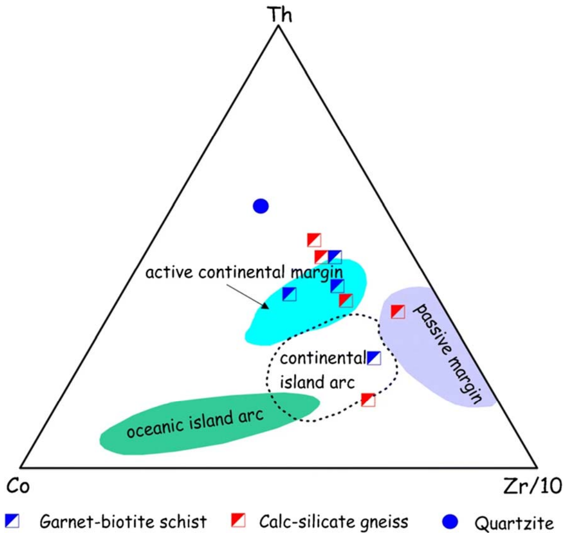
Fig. 11. Th – Co – Zr/10 tectonic setting discrimination ternary diagram (Bhatia and Crook 1986) for Okpella metasedimentary rocks
