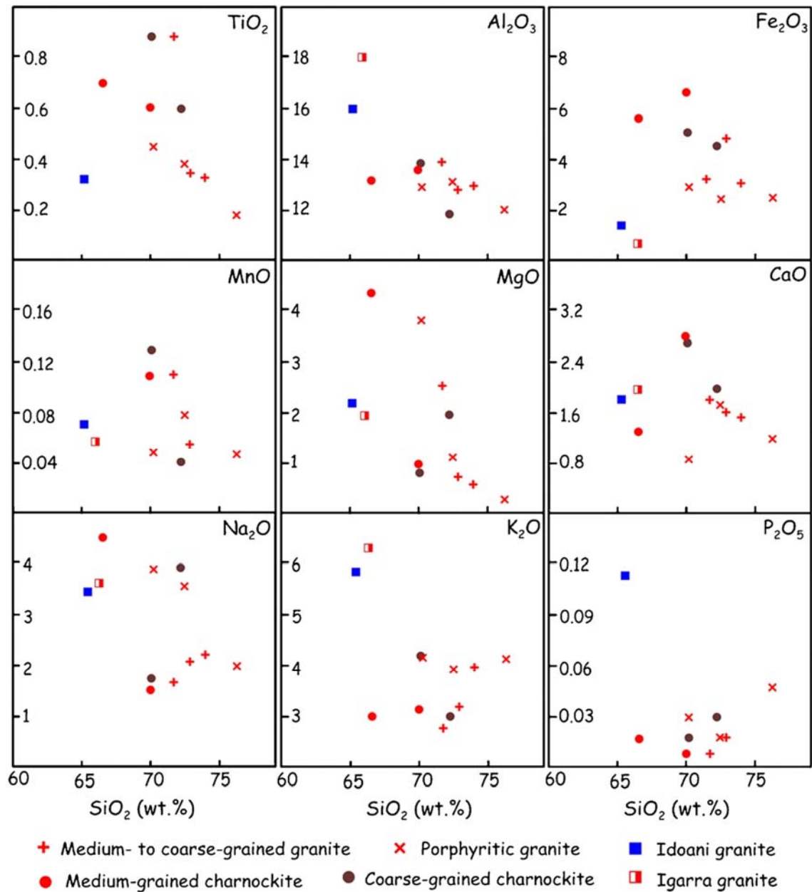
Fig. 7. Harker plots of some major elements against \text{SiO}_2 for Okpella granitoids and the Idoani and Igarra granites
