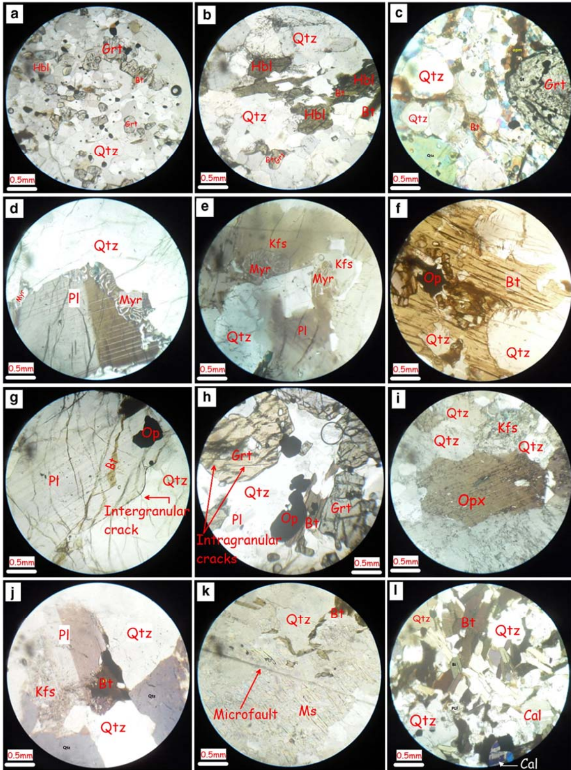
Fig 5. Representative photomicrographs of the studied rocks, mineral abbreviations used are according to Kretz (1983): a garnet-biotite schist composed of mafic bands (garnet + biotite + hornblende + opaques) and felsic bands (quartz + feldspar); b detailed view of the association quartz + garnet + biotite + hornblende, oriented along the foliation in garnet-biotite schist;
