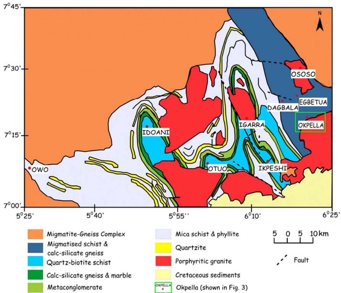
Fig 2. Geological map of Igarra Schist Belt showing Okpella area (modified after Odeyemi 1988)
