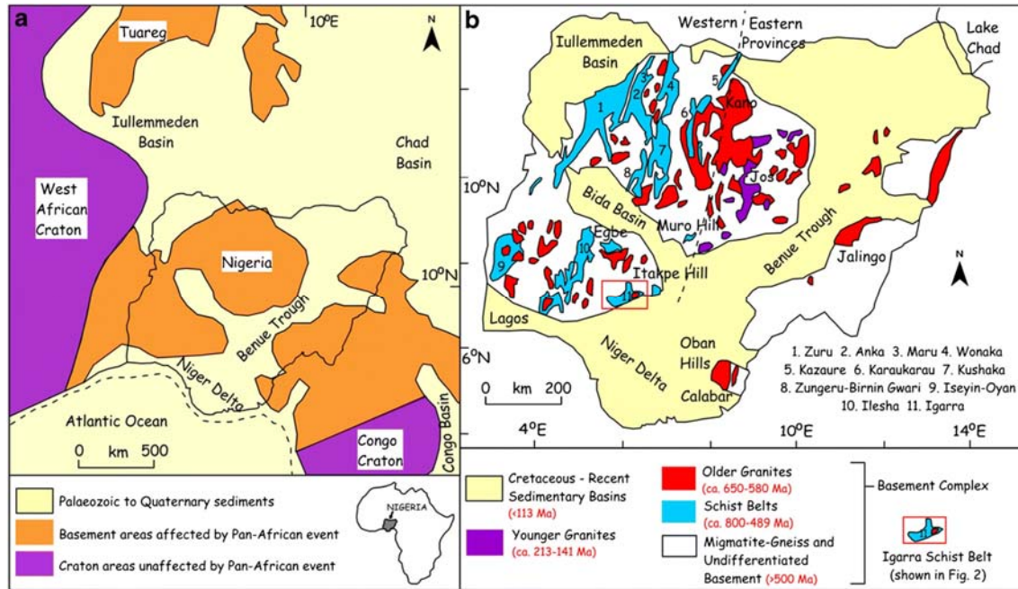
Fig. 1. a Regional geological map of Nigeria within the Pan-African Trans-Saharan mobile belt between the West African and Congo Cratons. b Outline geological map of Nigeria showing the Basement Complex, Younger Granites and Sedimentary Basins (modified after Woakes et al. 1987)
