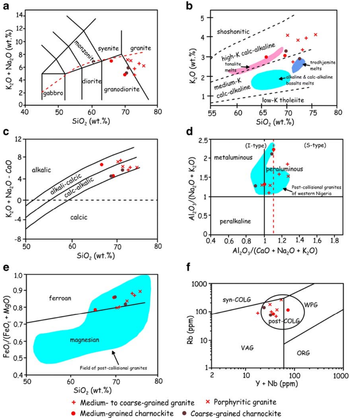
Fig 8. Petrochemical diagrams for discriminating Okpella charnockites and granites. a Total alkalis versus silica (after Gillespie and Styles 1999), red dashed line represents boundary between alkalic rocks above and sub-alkalic rocks below. b K 2 O versus SiO 2 plot (after Le Maitre 2002) with fields of compositions of tonalitic, trondhjemitic and basaltic melts from Roberts and Clemens (1993); (c) K 2 O + Na 2 O - CaO versus SiO 2 plot (after Frost et al. 2001). d Shand's Al 2 O 3 /(Na 2 O + K 2 O) versus Al 2 O 3 /(CaO + Na 2 O + K 2 O) molecular plot (after Maniar and Piccoli 1989), with field for post-collisional granites of western Nigeria (Goodenough et al. 2014) given for comparison. e FeO total /(FeO total + MgO) versus SiO 2 , with field for post-collisional granites from Frost et al. (2001). f Rb versus Nb + Y tectonic discrimination diagram (after Pearce et al. 1984)
