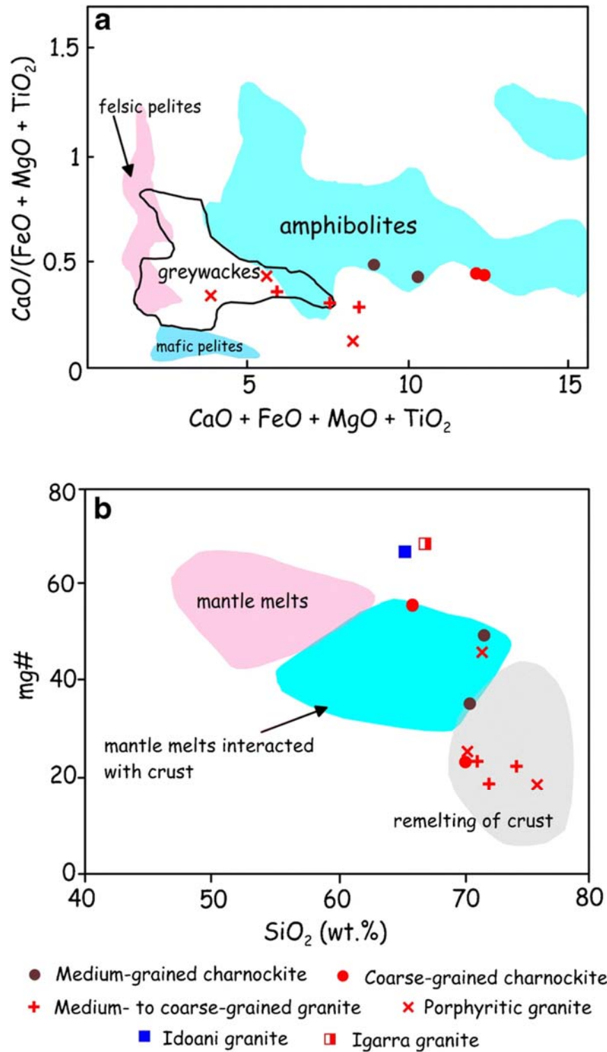
Fig. 9. a \text{CaO}/(\text{FeO} + \text{MgO} + \text{TiO}_2) versus \text{CaO} + \text{FeO} + \text{MgO} + \text{TiO}_2 discrimination plot of Patiño Douce (1999) for determining the source rock compositions of Okpella granitoids. The fields show the compositions of melts produced by experimental dehydration-melting of various lithologies. All values are in wt%. b mg# versus \text{SiO}_2 plot for Okpella granitoids and the Idoani and Igarra granites (after Peng et al. 2019)
