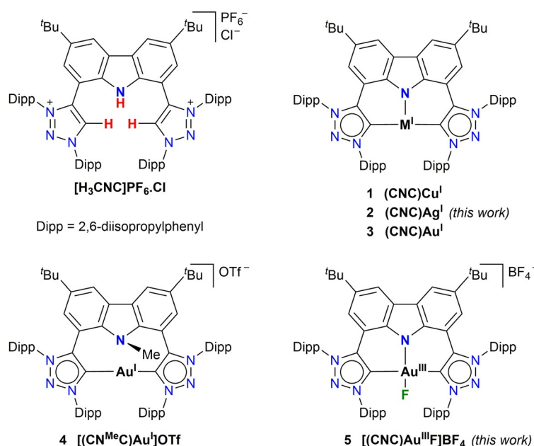
Figure 1. Precursor bis(triazolium)carbazole ligand salt [H_3CNC]PF_6 \cdot Cl and neutral (1–3) and cationic (4, 5) metal complexes employed in this study.
