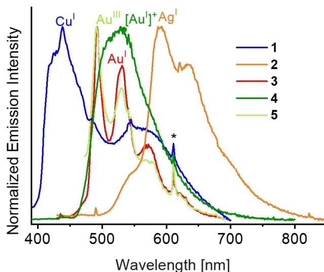
Figure 6. Normalized emission spectra of 1–5 in butyronitrile glass at 77 K; the asterisk represents an instrumental artifact.
