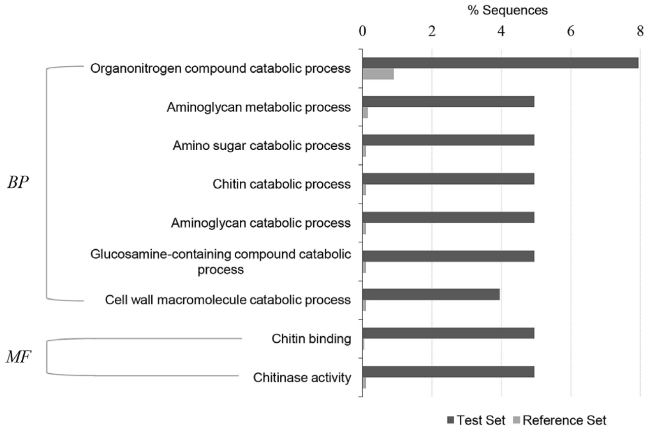
S2 Fig. Gene Ontology (GO) enrichment analysis of group 3 obtained in the hierarchical clustering analysis of Fig 4.
