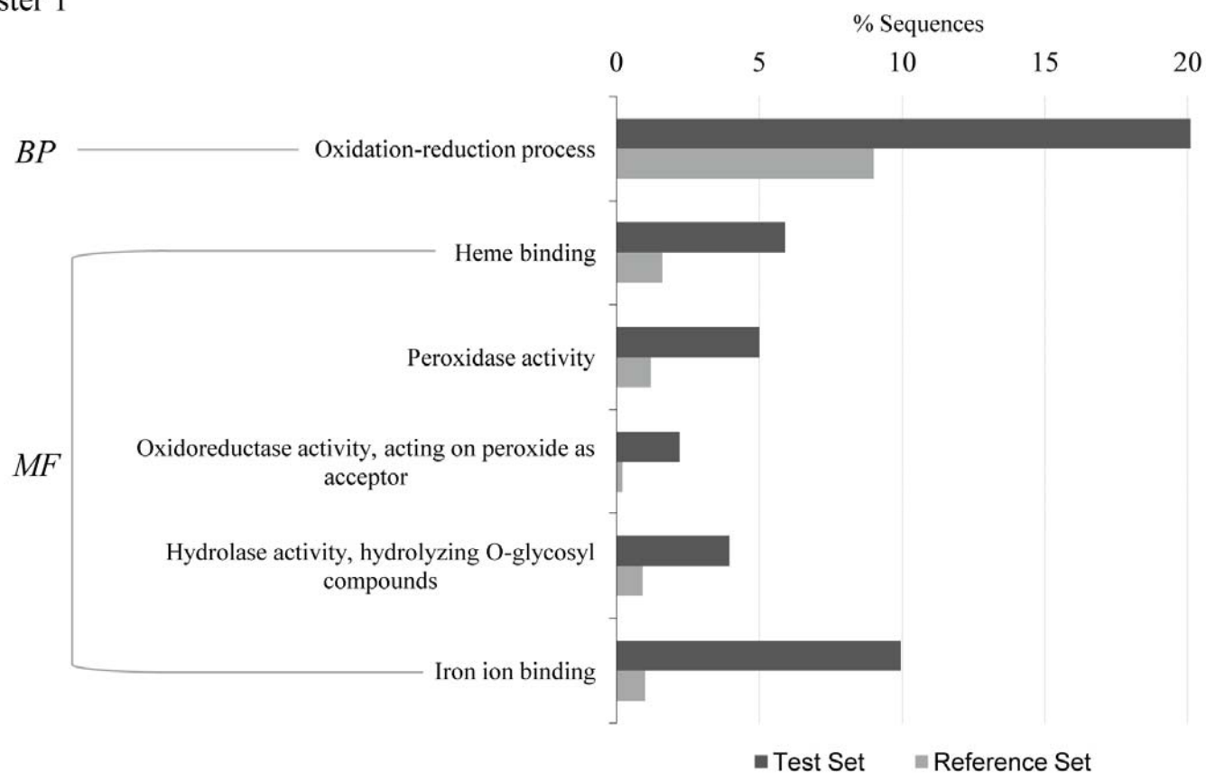
S1 Fig. Gene Ontology (GO) enrichment analysis of group 1 obtained in the hierarchical clustering analysis of Fig 4.
