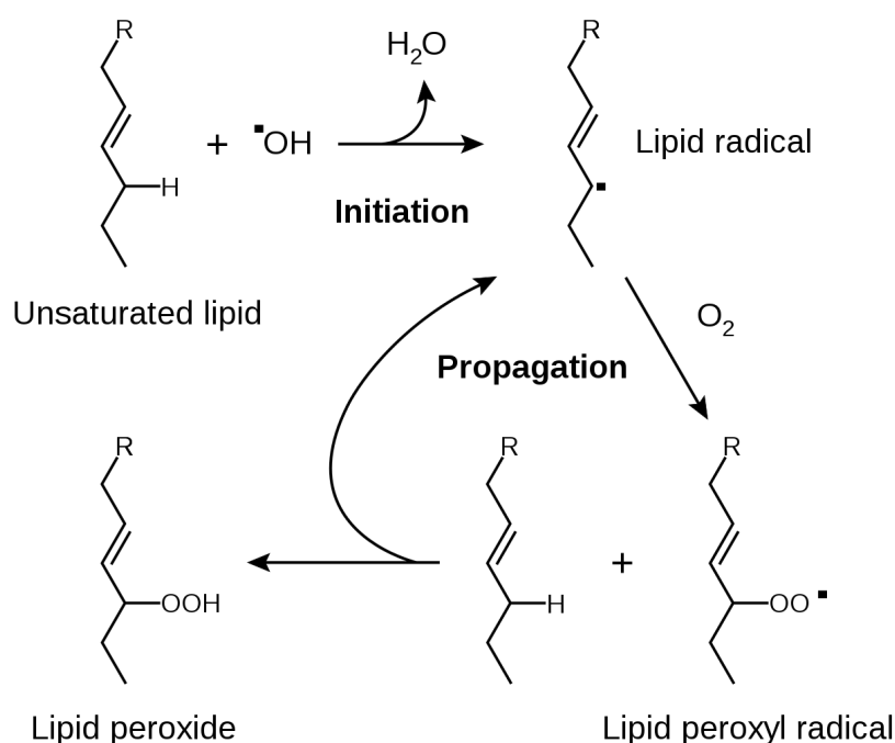
FIGURE 3.3: The peroxidation of lipids. By Tim Vickers, after (Young and McEneny 2001). Public Domain, https://commons.wikimedia.org/w/index.php?curid=1728531
