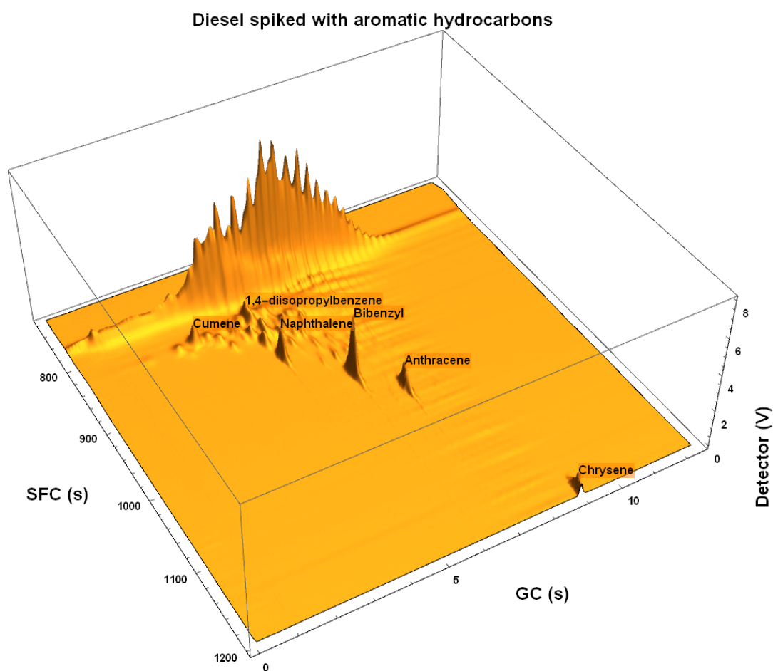
FIGURE 7.6: A 2D chromatogram of a commercial diesel sample spiked with selected aromatic compounds. Tentative peak assignments were made using knowledge of the boiling points and relative masses of the spike compounds.
