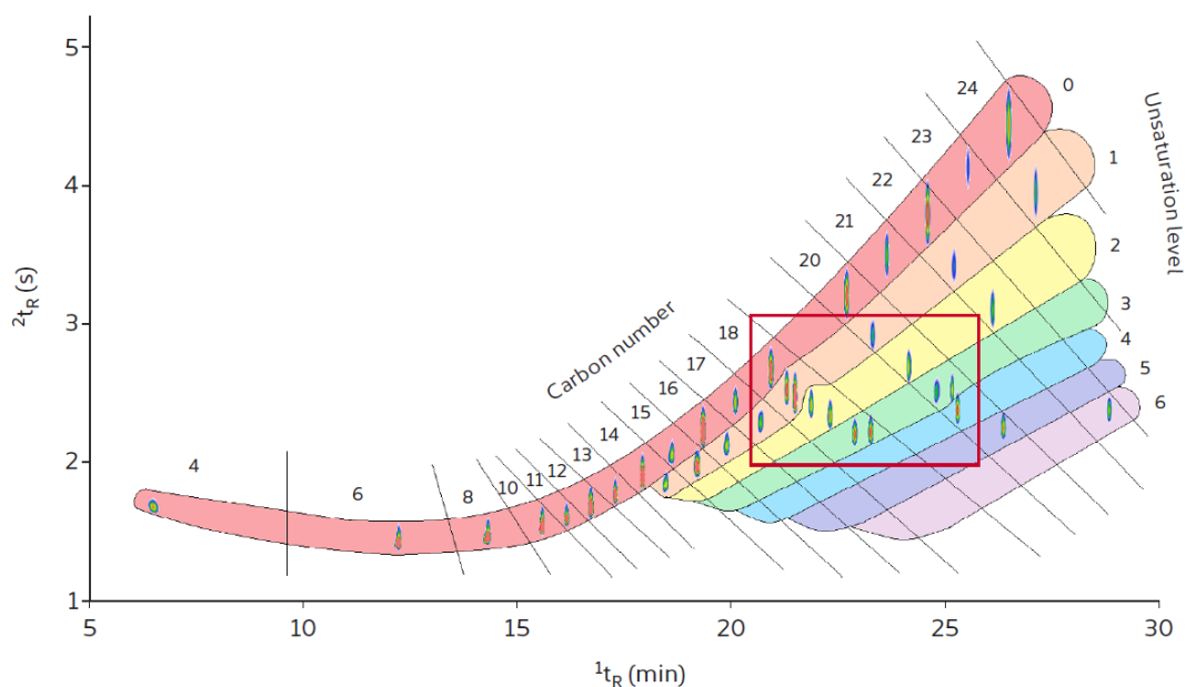
FIGURE 6.9: GC×GC-FID colour plot of a 37-component FAME standard. The coloured bands indicate successively higher levels of unsaturation, from 0 (red, no double bonds) to 6 (violet, with 6 double bonds) (SepSolve Analytical 2018).
