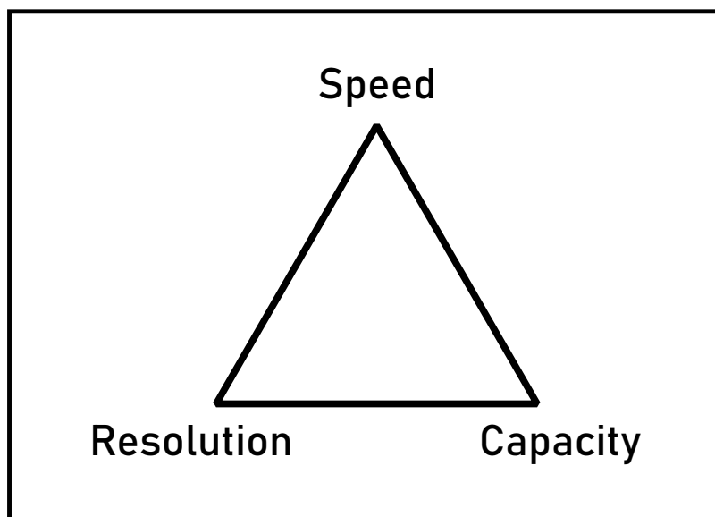
FIGURE 5.1: The chromatographer's trilemma.
