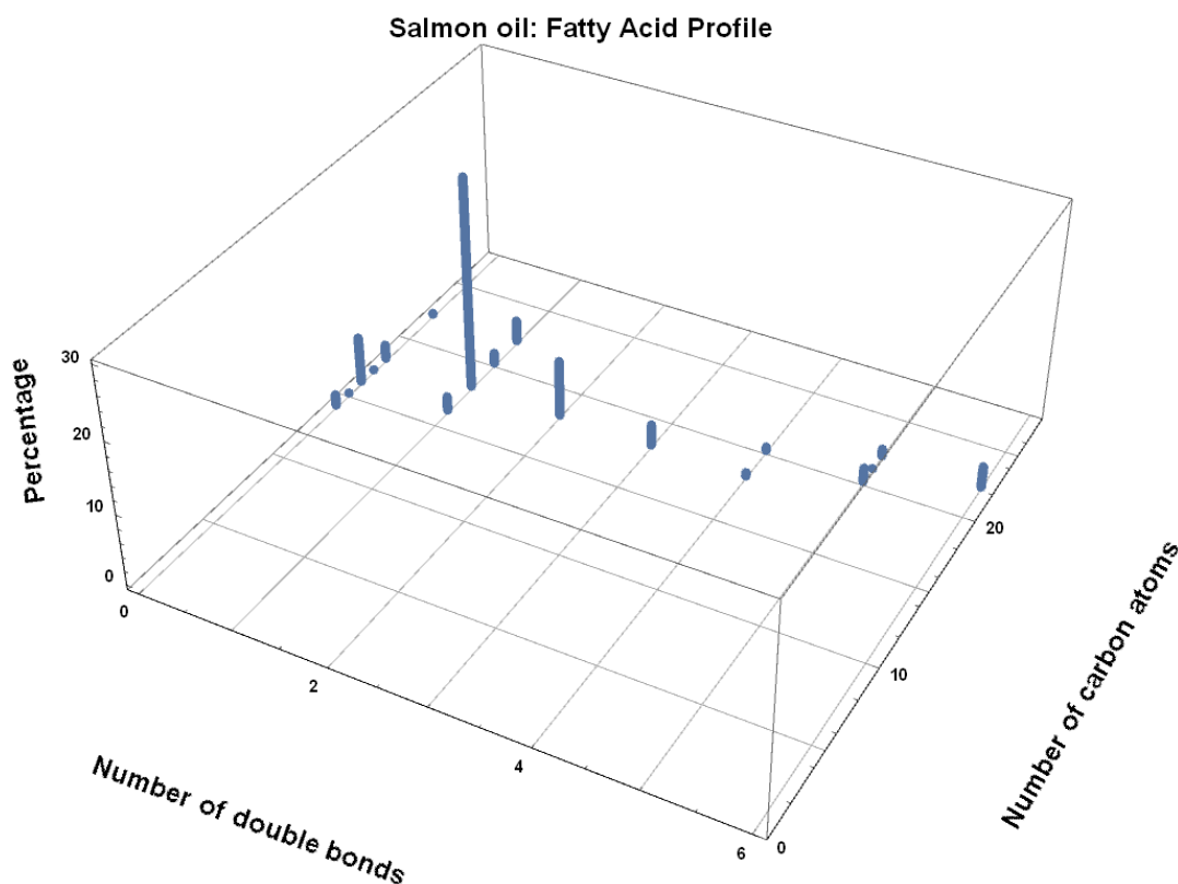
FIGURE 6.8: The fatty acid profile of salmon oil, when plotted on a suitably-scaled bar chart, shows how well the SFC×GC chromatogram of the same oil (Figure 6.7) represents the same data without any processing.
