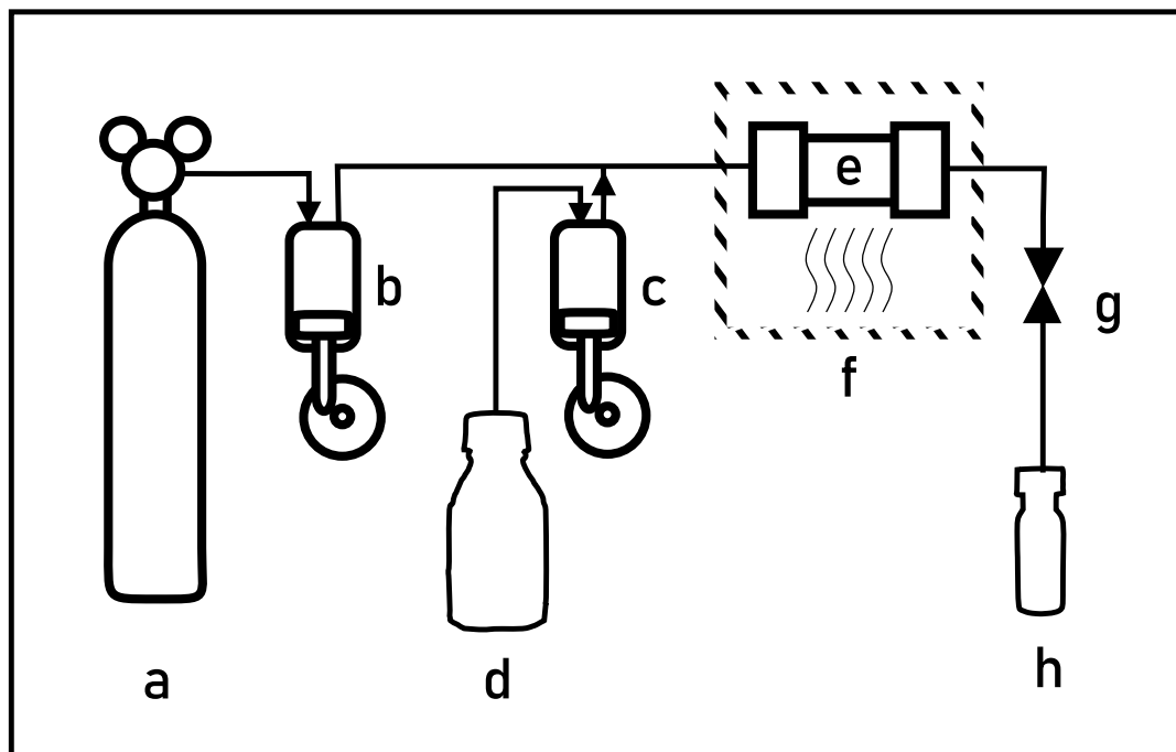
FIGURE 2.3: A diagram of an SFE system. (a) CO 2 supply (b) High-pressure SF pump (c) High-pressure modifier pump (d) Modifier reservoir (e) Extraction cell (f) Temperature control (g) Pressure control (h) Collection vessel
