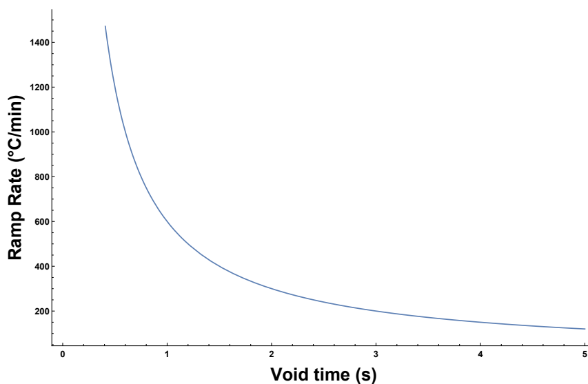
FIGURE 5.4: The ramp rate for temperature-programmed gas chromatography as a function of void time ( 10^{\circ}\text{C} per void time ( t_m )).
