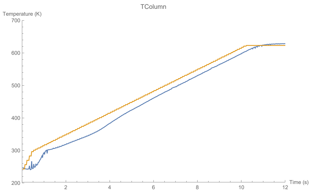
FIGURE 7.1: A comparison of the temperature set point and the indicated coaxial heater temperature during a fast GC run. The orange line shows the intended temperature program and the blue line shows the actual indicated temperature, as recorded. The “steps” in the orange line are caused by the 100 ms period of the control loop.
