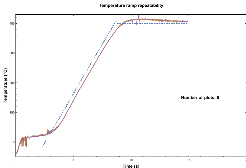
FIGURE 5.15: A graph of 9 identical, consecutive temperature ramps overlaid. The heating rate is 4000\text{ }^{\circ}\text{C min}^{-1} . The temperature follows (with some lag) the set point up to 350\text{ }^{\circ}\text{C} before deviating noticeably.
