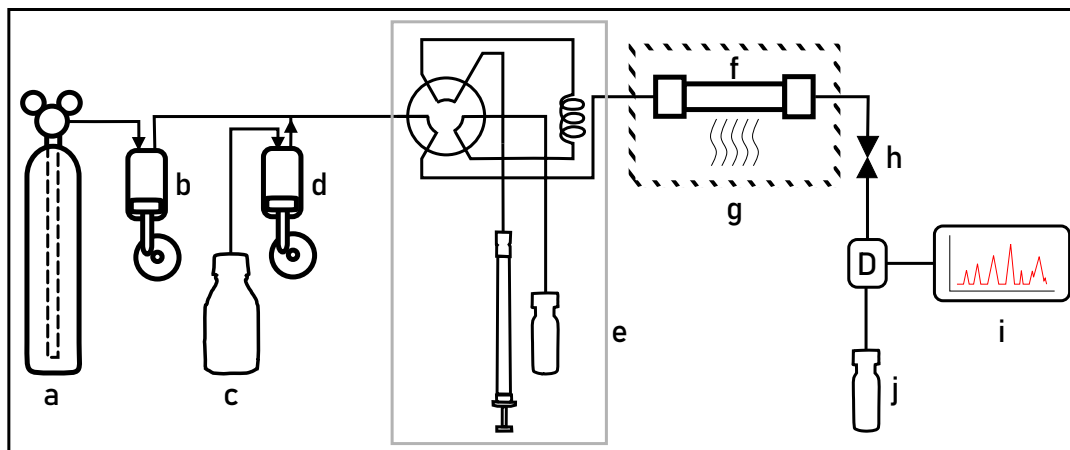
FIGURE 2.5: A diagram of an SFC system. (a) CO 2 supply (b) High-pressure SF pump (c) Modifier reservoir (d) High-pressure modifier pump (e) Injection system (f) Column (g) Optional heating (h) Back-pressure control (D) Detector (i) Data system (j) Optional fraction collection.
