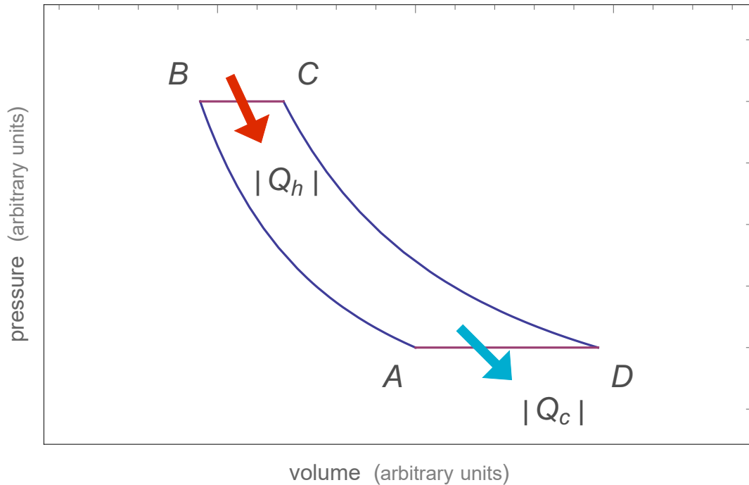
FIGURE 1.3: The pV diagram of the thermodynamic Brayton cycle. In the gas turbine the continuous combustion of the injected fuel and free expansion of the air through a turbine means that the heat addition (BC) is isobaric. Work is extracted during the adiabatic expansion process CD (Wolfram | Alpha 2019c).
