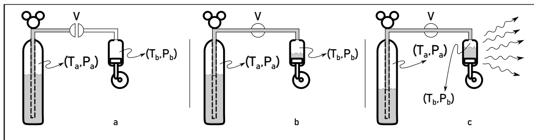
FIGURE 4.1: A schematic diagram of the process of the filling of the carbon dioxide pump. (a) The pressure in the reservoir P_a is much higher than the pressure in the receptacle P_b . The valve is closed, so there is no flow. (b) The valve is open and some carbon dioxide has flowed from the reservoir to the receptacle. But P_b = P_a , so there is no flow. (c) When the temperature in the receptacle T_b < T_a , then P_b < P_a , following Gay-Lussac's law. Flow will continue until all the vapour in the receptacle has condensed.
