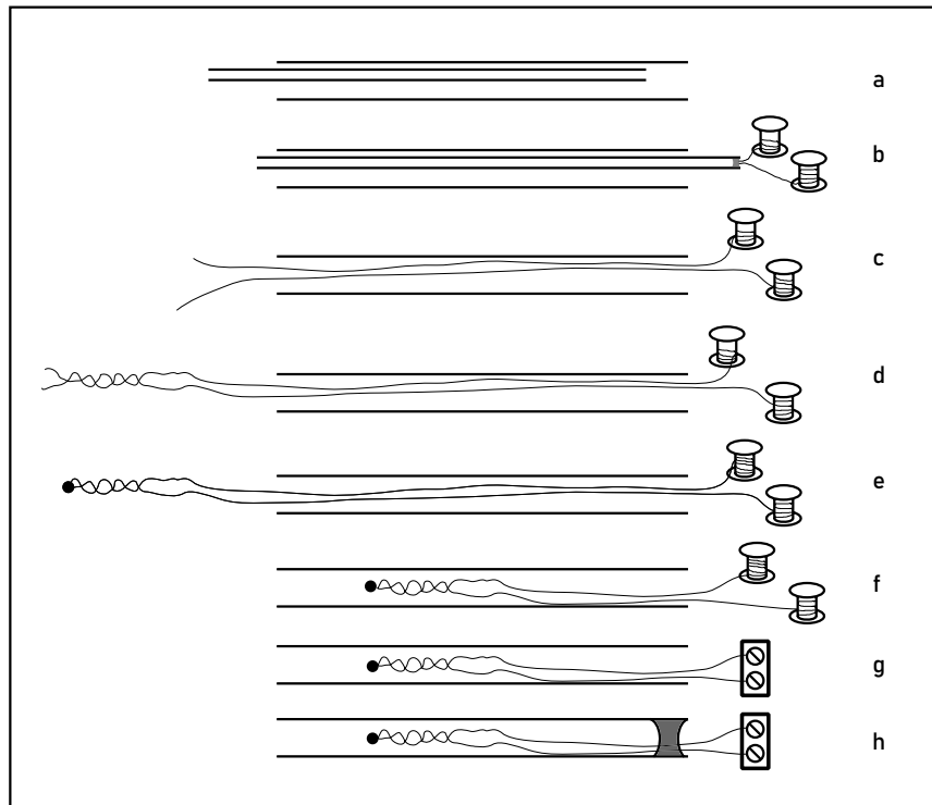
FIGURE 5.11: (a) A narrow capillary is threaded inside a wider one (b) The ends of a pair of thermocouple wires are fitted inside the end of the narrow capillary and anchored with cyanoacrylate adhesive. (c) The wires are pulled through the wider capillary using the narrow capillary. (d) The ends of the wires are twisted together, creating a mutual mechanical anchor. (e) The ends of the wires are welded together. (f) The wires are pulled back into the thick capillary, locating the junction at the desired position in the capillary. (g) The wires are trimmed and connected to a terminal block. (h) A drop of cyanoacrylate adhesive is used to anchor the wires permanently in the capillary.
