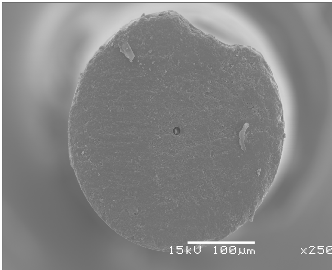
FIGURE 4.7: An electron micrograph of a restrictor tip, showing the size of the orifice.
