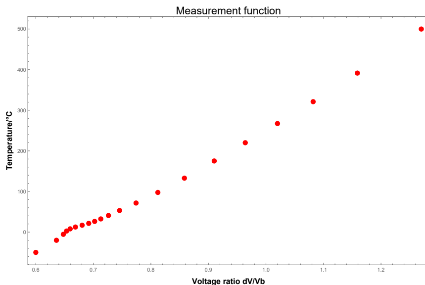
FIGURE 5.13: Measurement curve for the coaxial heater.
