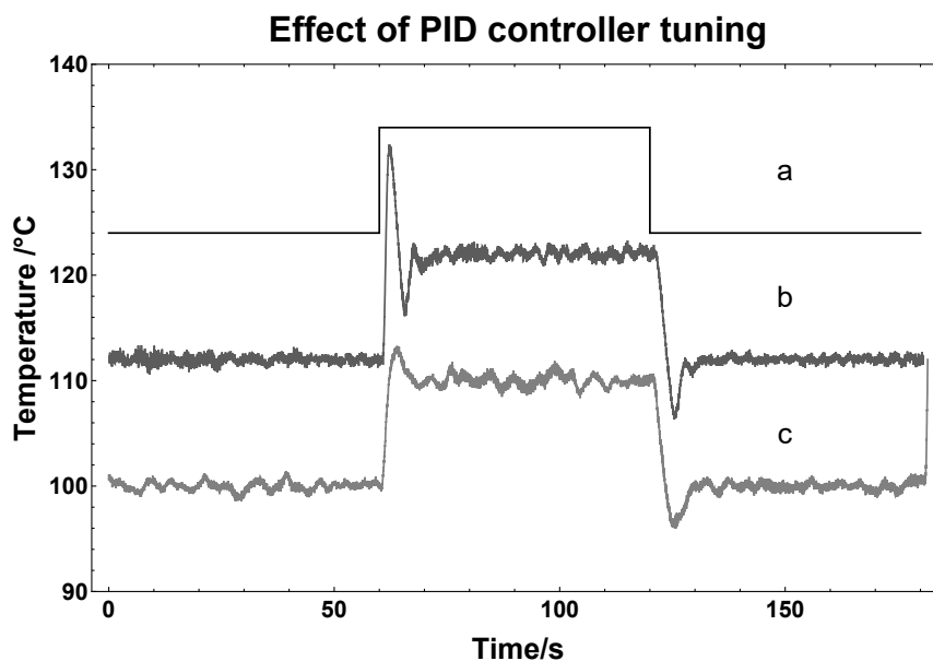
FIGURE 5.14: An illustration of effective PID controller tuning. The trace (a) represents the set point change over time and includes a step change. (b) Before tuning the temperature overshoots and then undershoots the step change in the set point. (c) After the controller has been tuned the overshoot in response to a step change in the set point is minimized.
