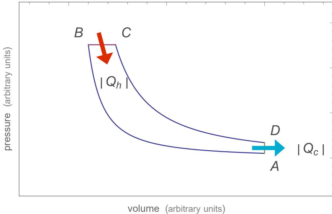
FIGURE 1.2: The pV diagram of the thermodynamic Diesel cycle. The isobaric process BC corresponds to the combustion of the finely divided fuel particles in air. Work is extracted from the engine both during this process and during the adiabatic process CD . (Wolfram | Alpha 2019b)
