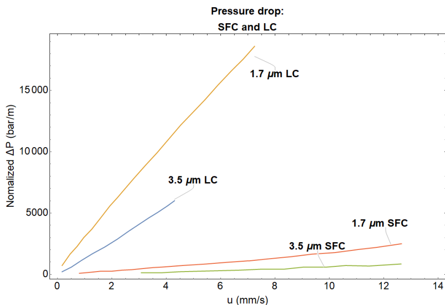
FIGURE 2.7: Normalized generated pressure drop as a function of linear velocity for 1.7 \mu\text{m} and 3.5 \mu\text{m} particles in LC and SFC. Each curve represents the pressure drop required to generate the linear velocity of the corresponding curve in Figure 2.6, normalized to 1 m of column to avoid influence of column geometry variations. Adapted from (Perrenoud, Veuthey, and Guillaume 2012).
