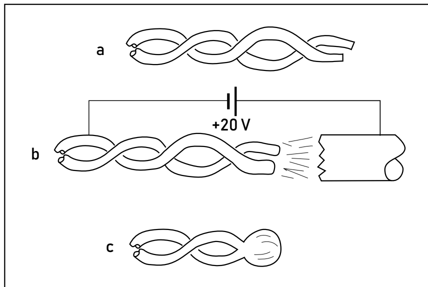
FIGURE 5.8: The process of welding fine wires to make thermocouples (a) Wires twisted together (b) Electric arc heating up the wires (c) Wires welded with a well-formed bead.
