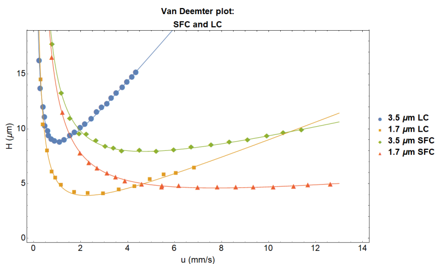
FIGURE 2.6: Kinetic performance as a function of linear velocity for different particle sizes in LC and SFC. Van Deemter curves for butylparaben on 2 systems equipped with 1.7 \mu\text{m} or 3.5 \mu\text{m} particles columns. LC conditions: \text{H}_2\text{O}/\text{ACN} (60/40, v/v), 30 ^\circ\text{C} , 1 \mu\text{l} injected. SFC conditions: \text{CO}_2/\text{MeOH} (96/4, v/v), 40 ^\circ\text{C} , 150 bar backpressure, 1 \mu\text{l} injected. Adapted from (Perrenoud, Veuthey, and Guillaume 2012).
