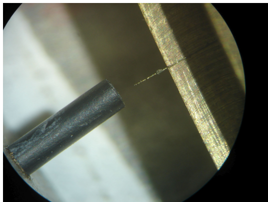
FIGURE 5.10: A microphoto of a pair of twisted thermocouple wires ready to be welded. The black carbon electrode is 2 mm in diameter.
