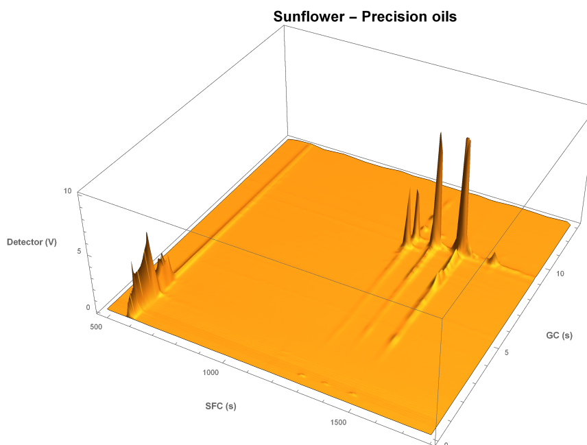
FIGURE 5.18: A 2D SFC×GC chromatogram of fatty acid methyl esters of sunflower oil
