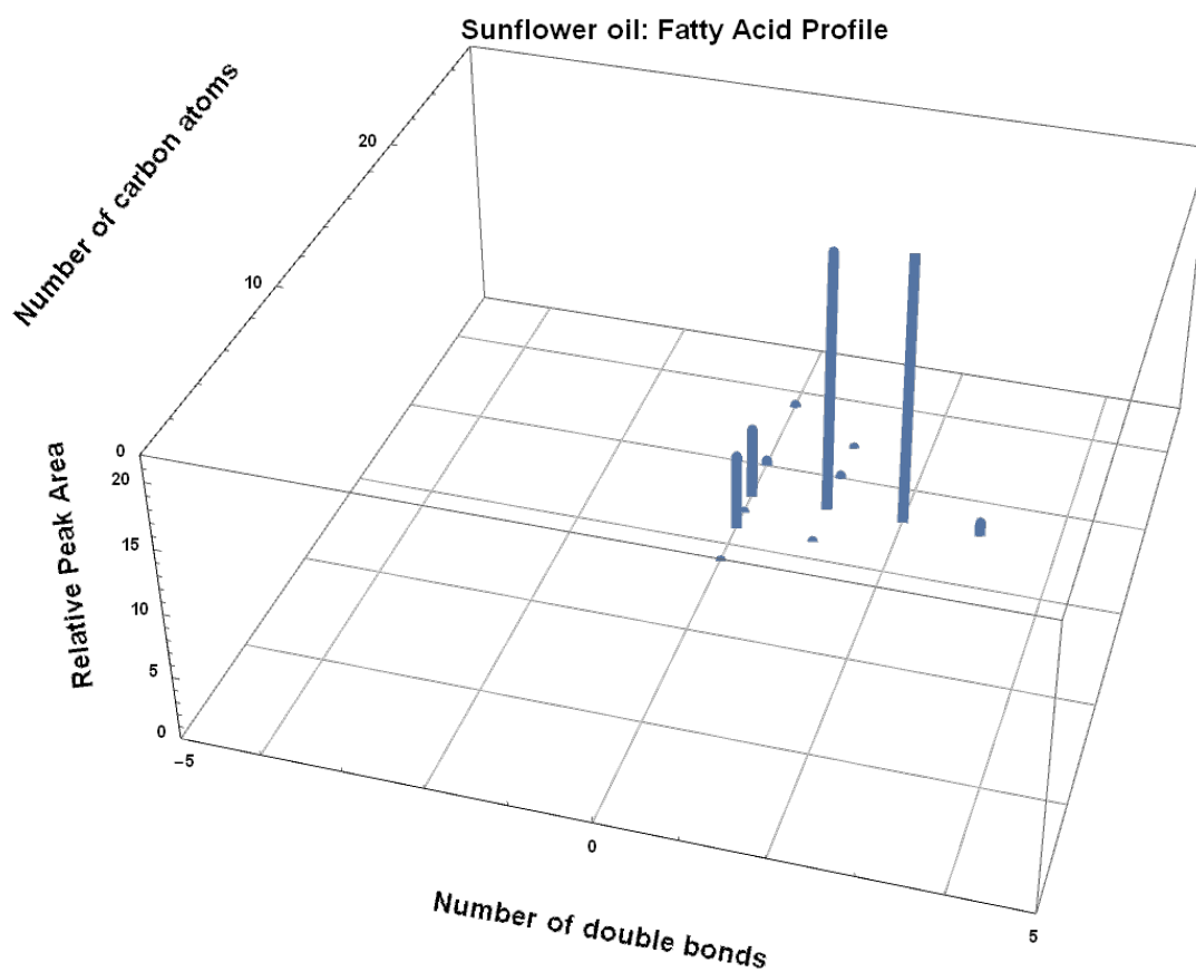
FIGURE 6.4: The fatty acid profile of a sunflower oil, when plotted on a suitably-scaled bar chart, shows how well the SFC×GC chromatogram of the same oil (Figure 6.3) represents the same data without any processing.
