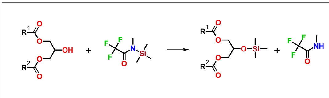
FIGURE 3.4: The derivitization of a diglyceride with N-methyl-N-(trimethylsilyl)-trifluoroacetamide (MSTFA). During GC the inert trimethylsilyl group does not interact with the stationary support, and the volatile trifluoroacetamide elutes with the solvent front.
