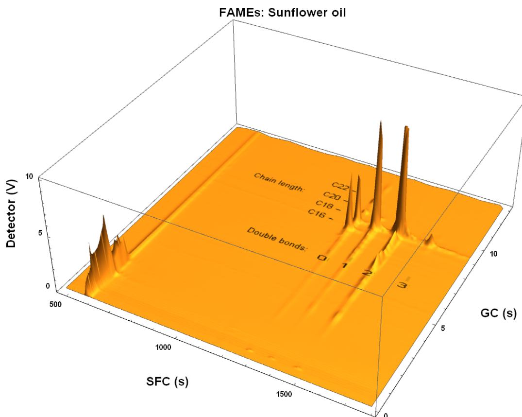
FIGURE 6.3: A 2D chromatogram of FAMES derived from sunflower oil. It is clear that the oil consists mostly of unsaturated fatty acids, with a high proportion of linoleic acid (C18:2).
