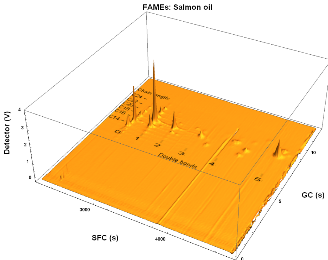
FIGURE 6.7: A 2D chromatogram of FAMES derived from salmon oil. It is clear that the oil contains significant quantities of polyunsaturated fatty acids.
