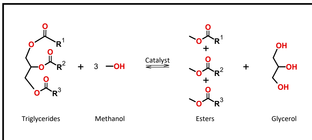
FIGURE 1.4: Transesterification: the chemical reaction that converts vegetable oils into biodiesel
