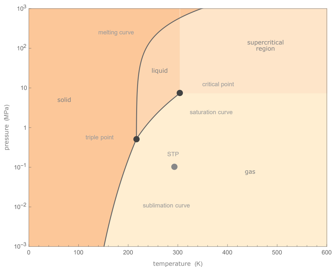
FIGURE 2.2: The phase diagram of carbon dioxide (Wolfram | Alpha 2019d).
