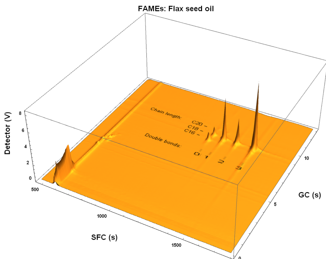
FIGURE 6.6: A 2D chromatogram of FAMES derived from flax seed oil. It is clear that the oil consists mostly of highly unsaturated fatty acids.
