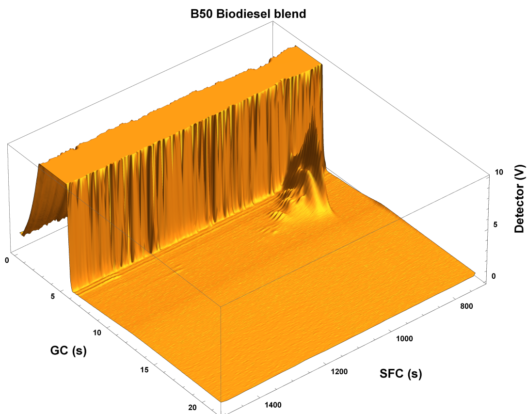
FIGURE 8.1: The modifier used in the SFC dimension elutes as a solvent front on the GC dimension, and does not otherwise affect the separation.
