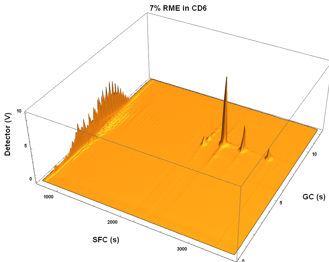
FIGURE 7.2: A 2D chromatogram of biodiesel and petrodiesel in a 7% blend. The hydrocarbons elute completely before the first FAME elutes, offering interference-free determination of both. The chromatogram was compiled from 368 1D fast temperature-programmed GC chromatograms.
