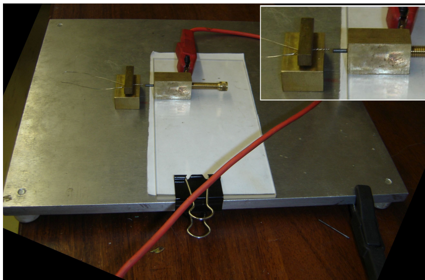
FIGURE 5.9: A view of the fine-wire thermocouple welder, as set up on a microscope base plate. The wire shown in the photograph is much thicker the one actually used. It is shown clamped between the clamping bar and the clamping weight. A thin sheet of acrylic serves to isolate the positive electrode from the negative base. The carbon electrode can be advanced towards the thermocouple twist using the screw. The black clamp at the bottom right-hand corner attached to the base plate and the red clamp attached to the screw housing provide a potential difference of approximately 20 V between the carbon electrode and the thermocouple. To do (??)
