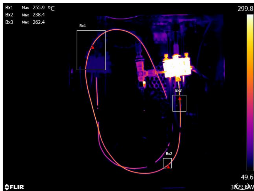
FIGURE 5.7: A thermograph of the coaxial heater at high temperature. It shows that there are no runaway hot spots.
