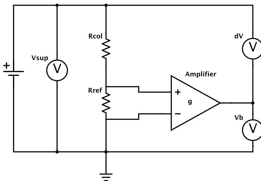
FIGURE 5.5: Electric circuit diagram of the coaxial heater.
