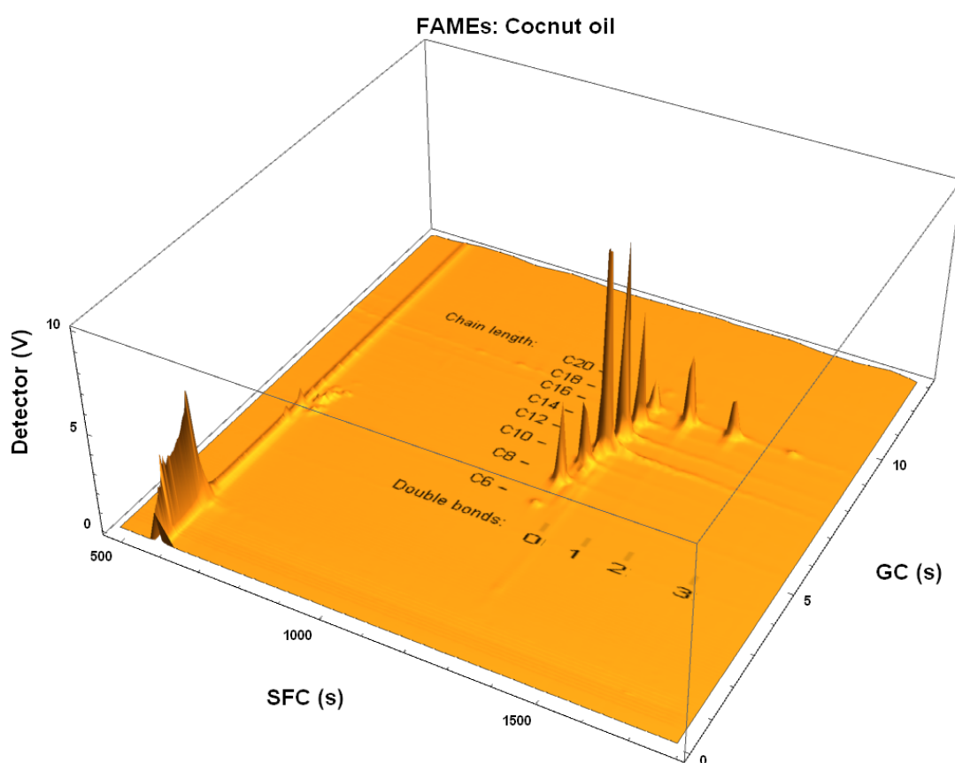
FIGURE 6.5: A 2D chromatogram of FAMES derived from coconut oil. It is clear that the oil consists mostly of saturated fatty acids.
