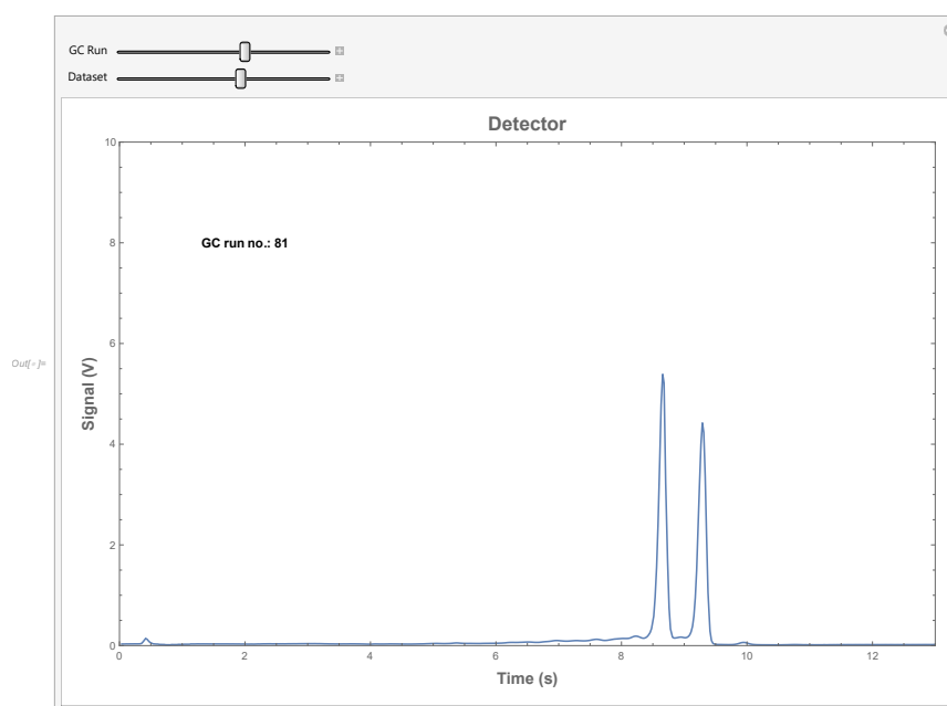
FIGURE 5.17: A single fast GC chromatogram, in a Mathematica Manipulate[] environment. The sliders can be used to select which GC run to view, and which data of that run.
