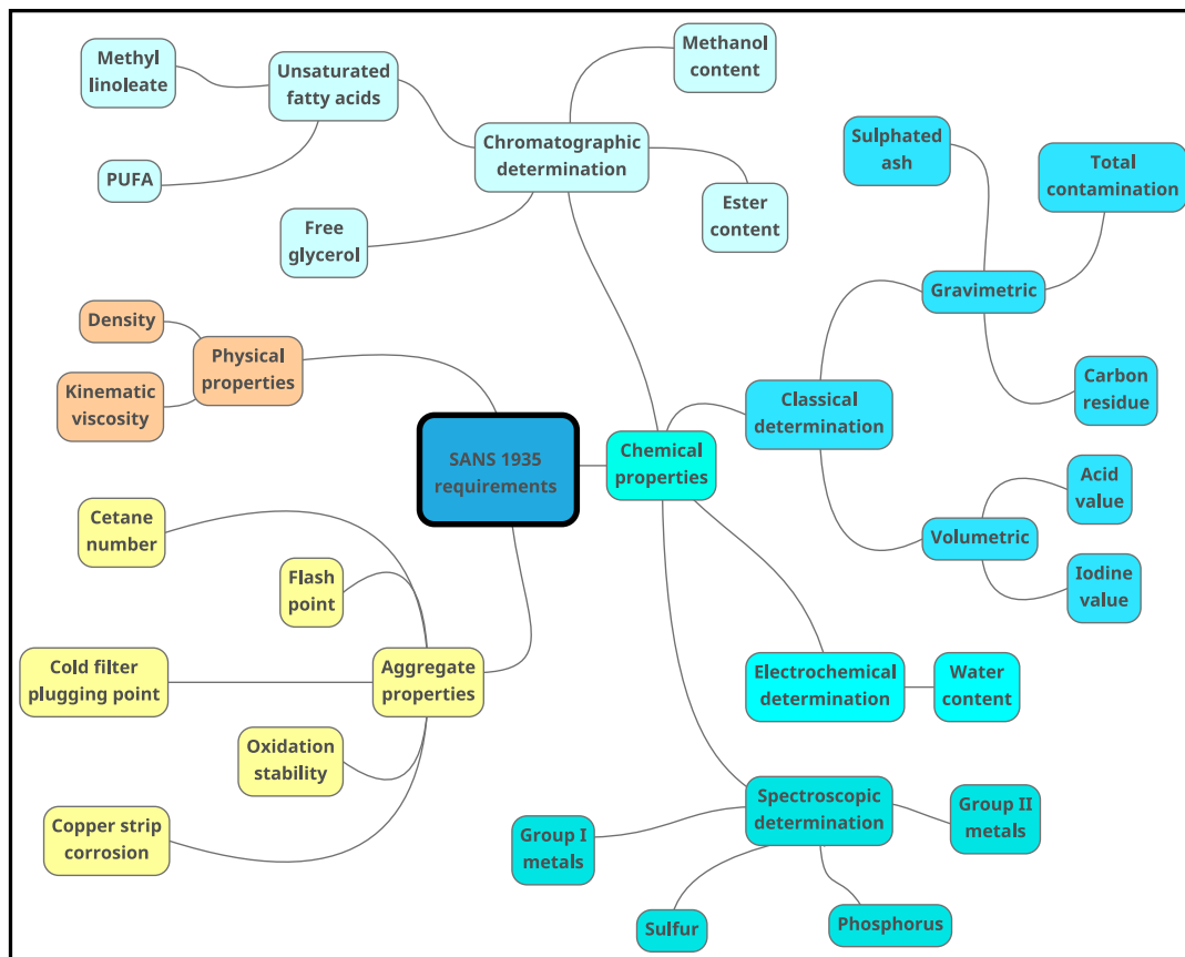
FIGURE 3.1: A mind map showing how the properties of biodiesel assessed by SANS 1935 is grouped for the purpose of discussion in this chapter.
