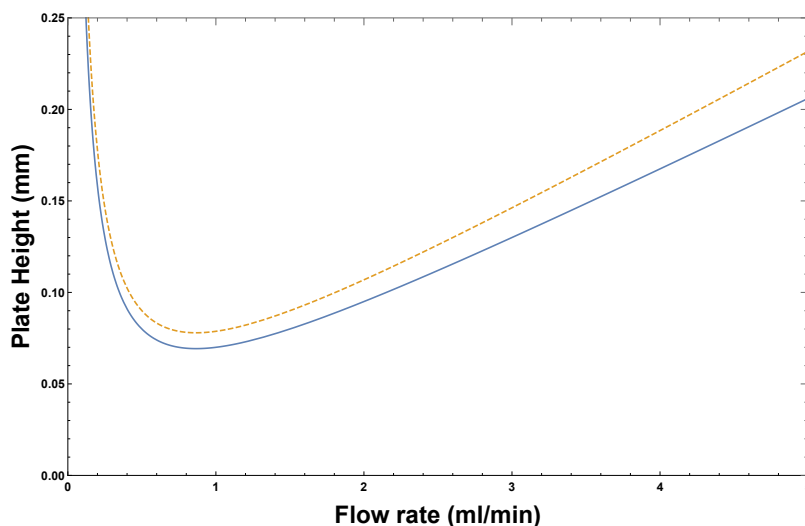
FIGURE 5.2: A plot of H vs. F . The solid line represents the low pressure drop case, and the dashed line the high pressure drop case.
