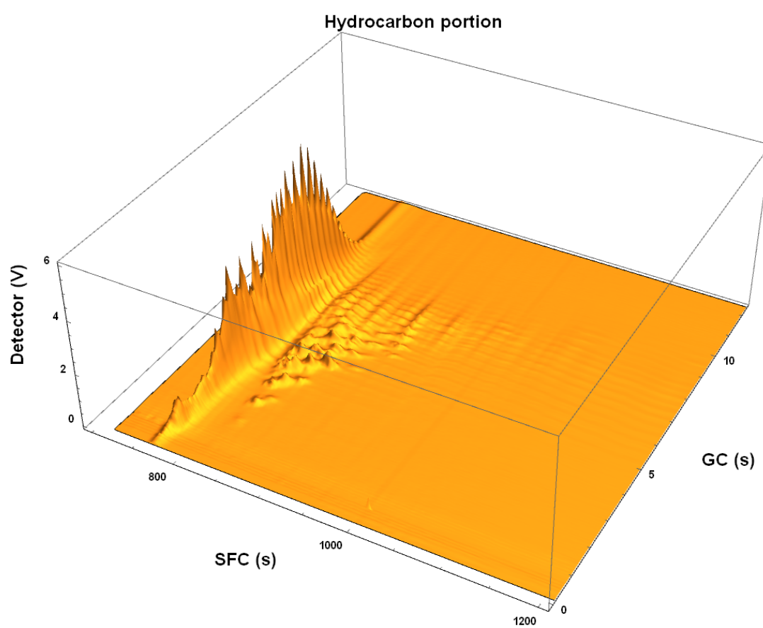
FIGURE 7.4: The portion of the chromatogram of the 7% biodiesel blend that contains the peaks attributed to the hydrocarbons.
