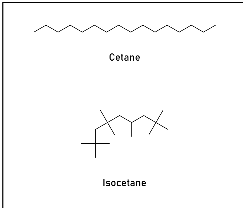
FIGURE 3.2: The chemical structures of the C16 hydrocarbon isomers cetane and isocetane.
