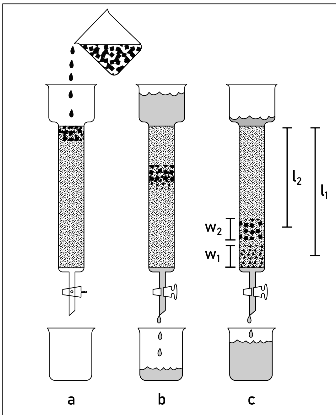
FIGURE 2.4: A conceptual diagram of basic chromatography. (a) A mixture of compounds (represented by squares and triangles) are introduced in a thin band on the head of a column (stippled area). (b) A solvent (grey) is run through the column. The different compounds migrate at different rates. (c) If conditions are optimal the compounds are separated fully (but not excessively) when they reach the end of the column. R_s = 2(l_1 - l_2) / (w_1 + w_2)
