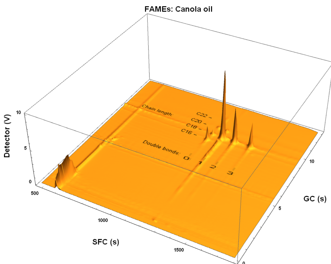
FIGURE 6.2: A 2D chromatogram of FAMES derived from canola oil. It is clear that the oil consists mostly of unsaturated fatty acids.
