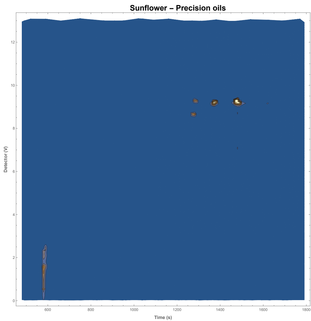
FIGURE 5.19: The SFC×GC contour plot representation of the 2D chromatogram shown in Figure 5.18.
