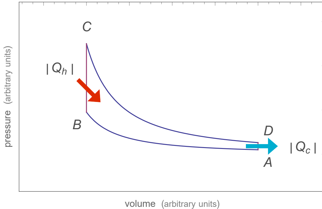
FIGURE 1.1: The pV diagram of the thermodynamic Otto cycle. The isochoric heat addition step (BC) corresponds to the burning of the homogeneous air-fuel mixture. Work is extracted from the engine during the adiabatic expansion CD (Wolfram | Alpha 2019a).
