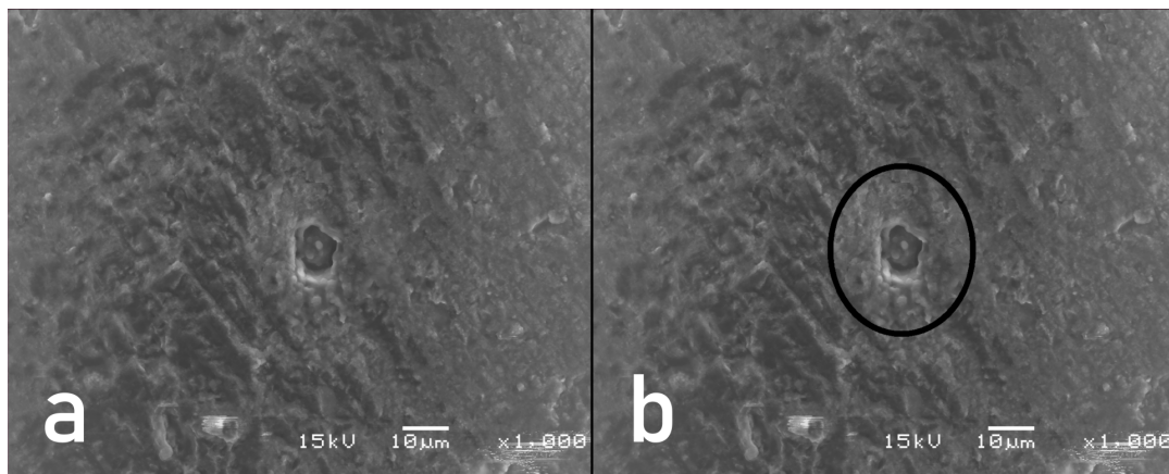
FIGURE 4.8: An electron micrograph of a blocked restrictor orifice. (a) Original image (b) Image with black circle showing estimated original orifice location
