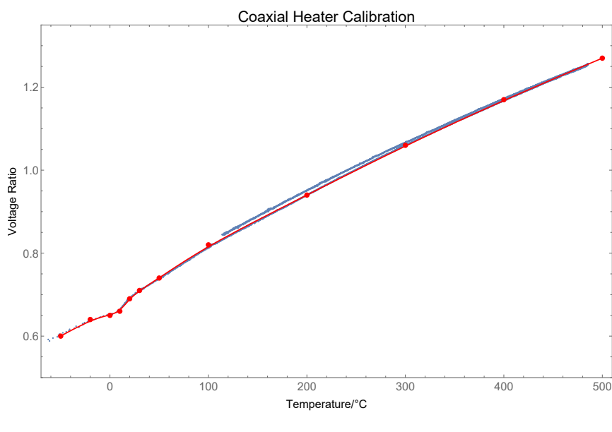
FIGURE 5.12: Calibration curve for the coaxial heater.
