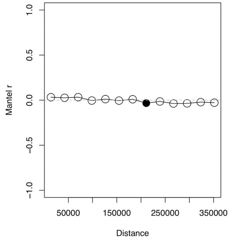
Figure S3: Mantel tests for the full generalized linear mixed model with negative binomial distribution
