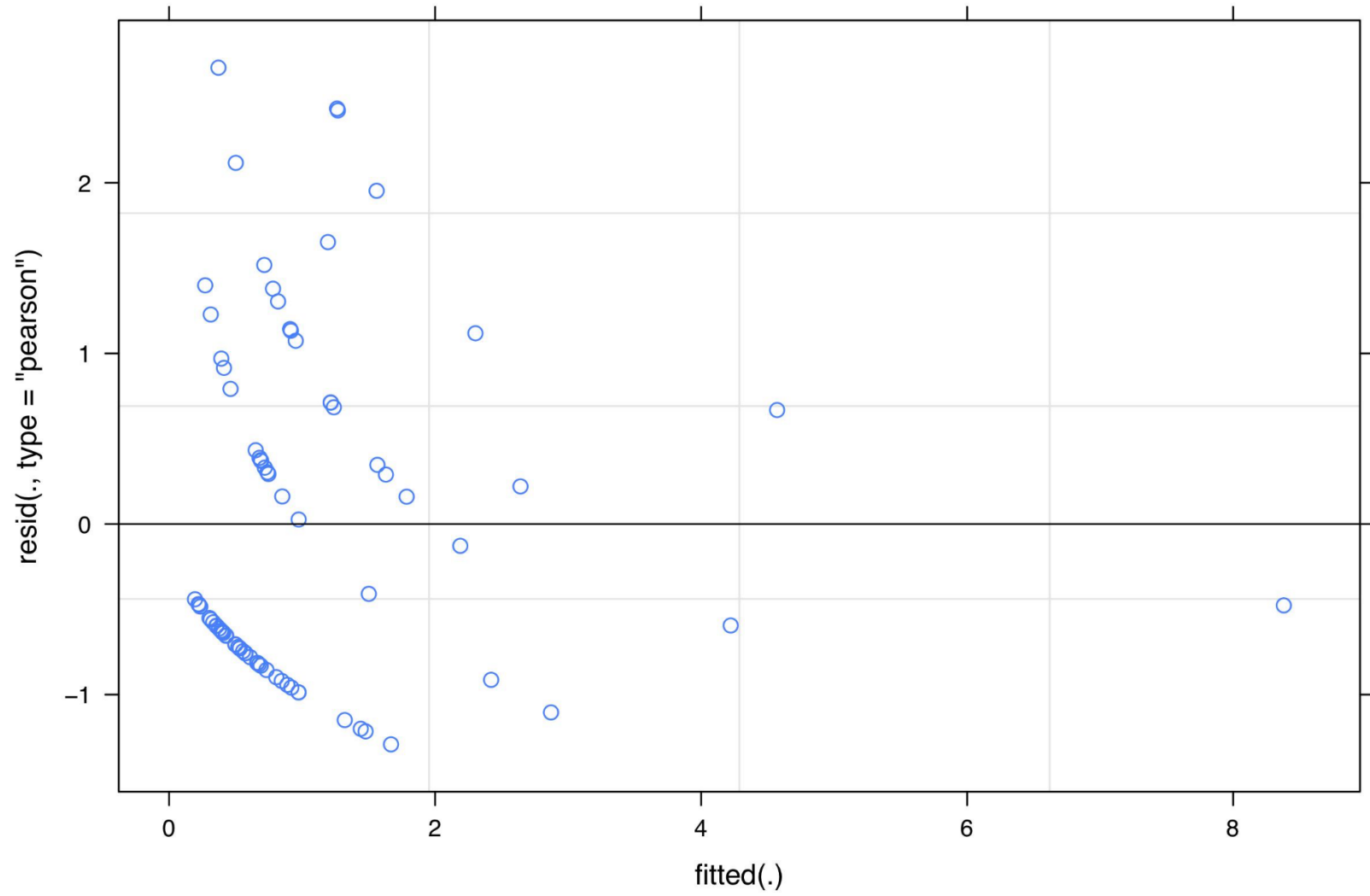
Figure S2: Scatter plot of fitted vs residual values for the full generalized linear mixed model with negative binomial distribution
