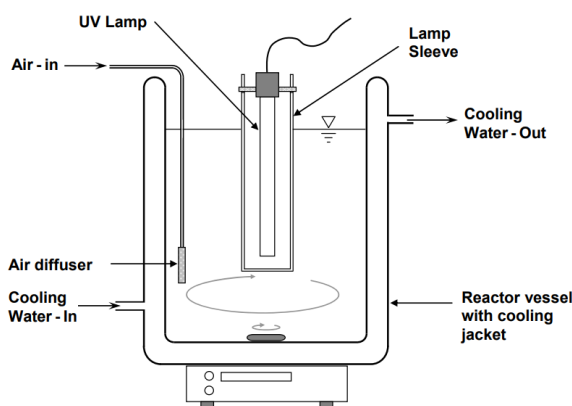
Figure 3: Photocatalytic reactor set-up (Adopted from Bamuza-Pemu and Chirwa).
