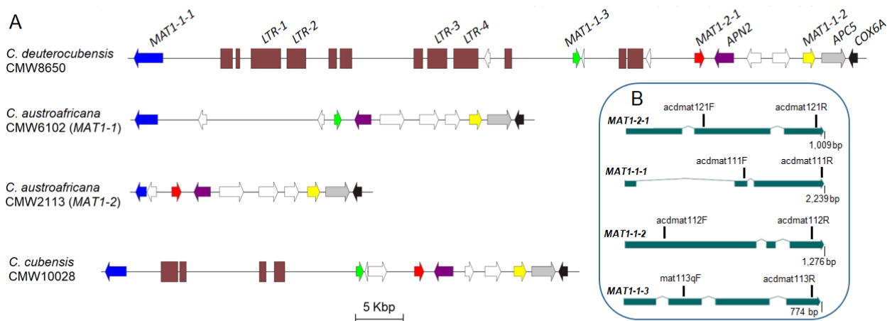
Fig. 1. (A) MAT loci of C. austroafricana CMW6102 ( MAT1-1 ), C. austroafricana CMW2113 ( MAT1-2 ), C. deuterocubensis and C. cubensis showing genes and repeat regions. (B) Annotation of the diagnostic MAT primers on the MAT genes of C. cubensis . The location of the MAT gene primers was the same in C. austroafricana , and C. deuterocubensis .
