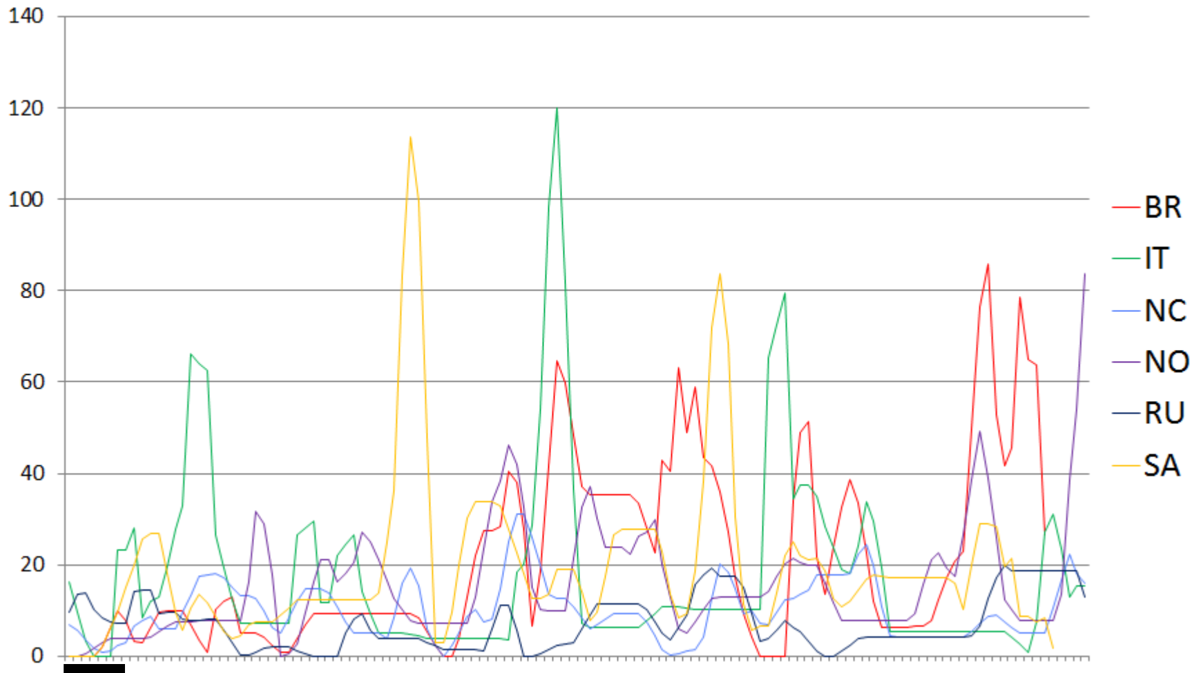
Chromosome 10
