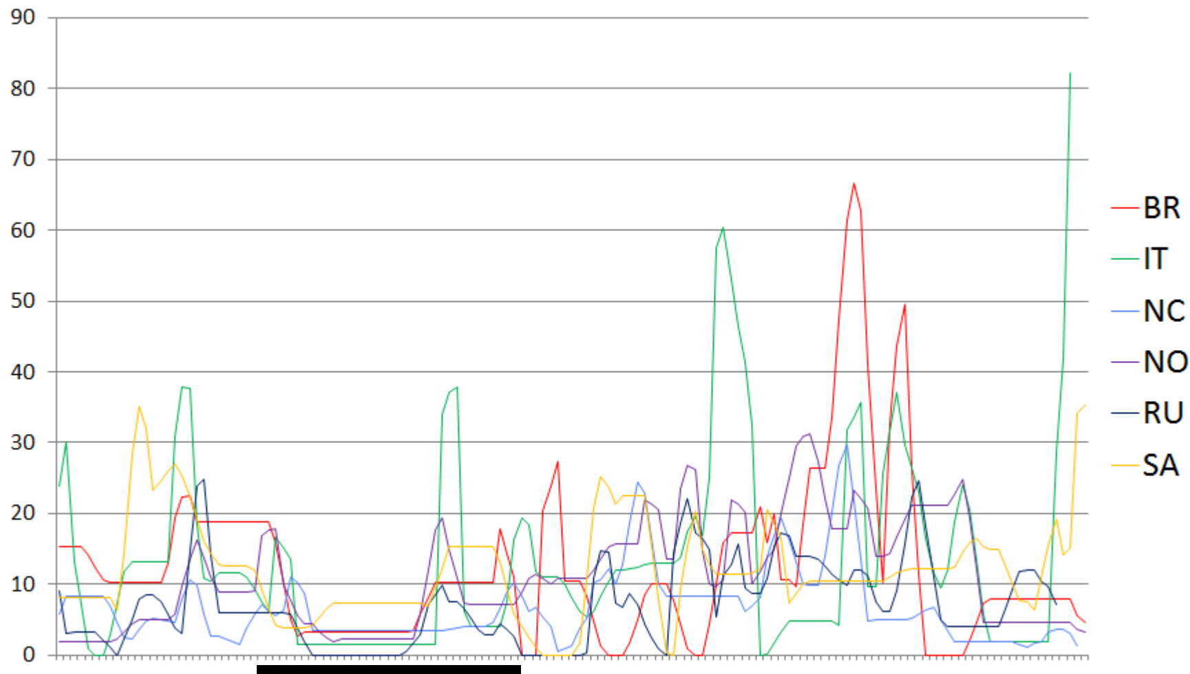
Chromosome 11
