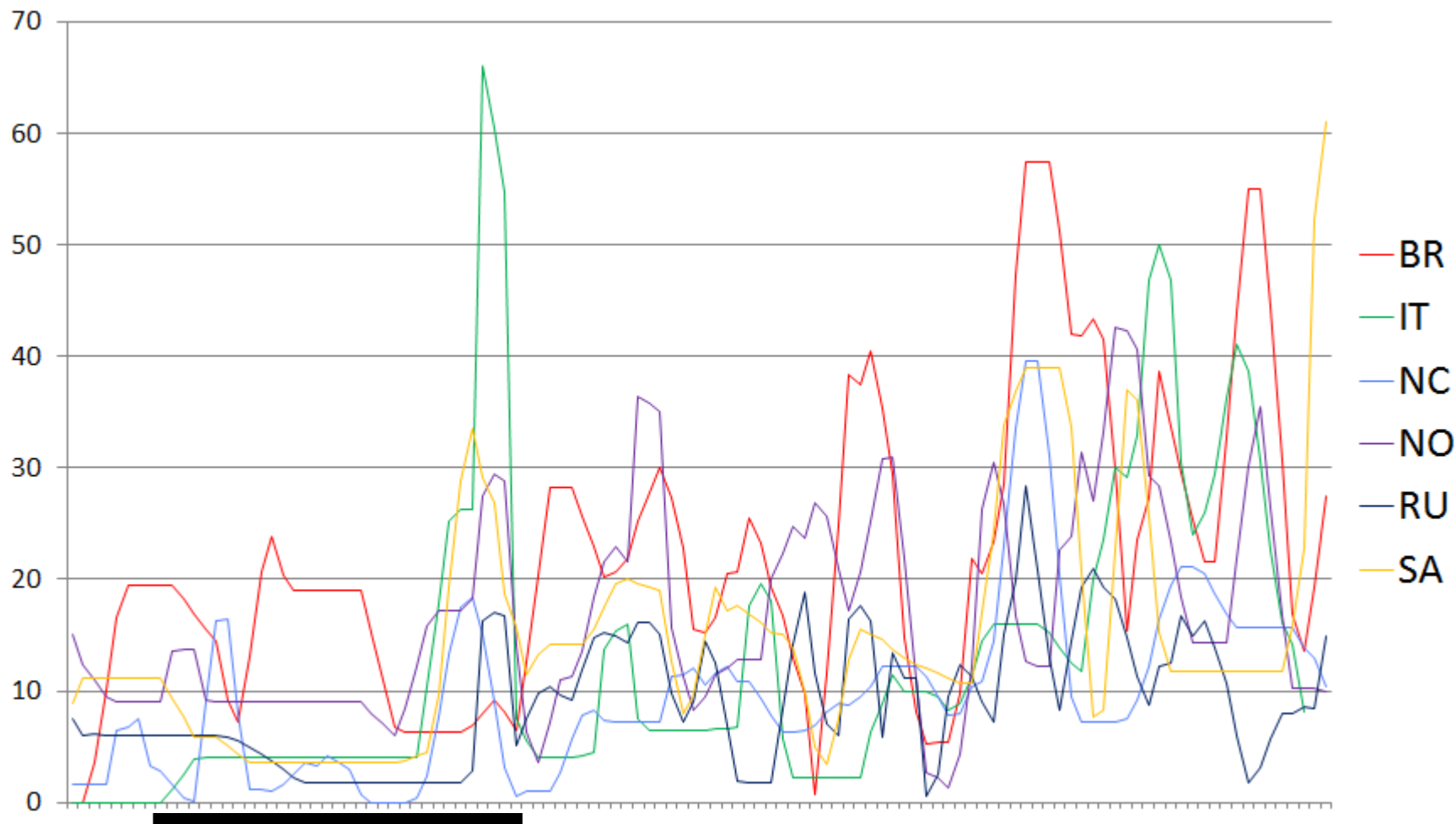
Chromosome 12
