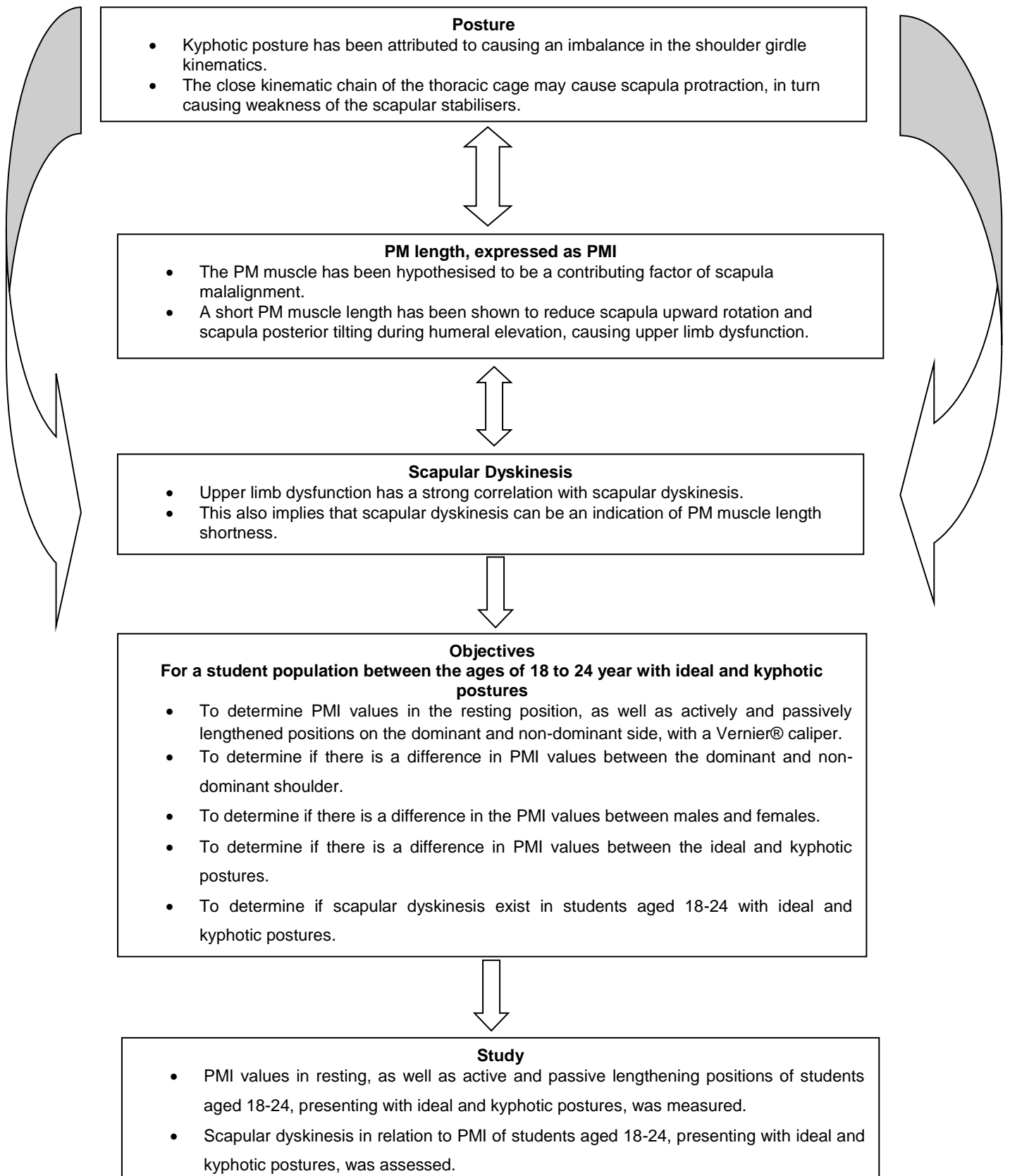
Figure 1. 1 Conceptual Framework
