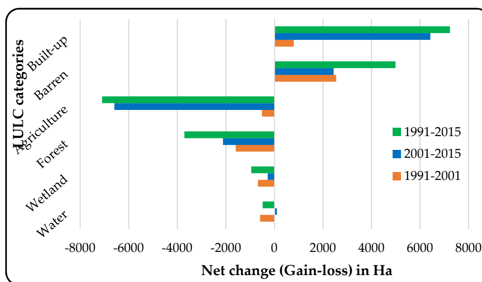
Figure 3. Net change in LULC classes between 1991 and 2015.
