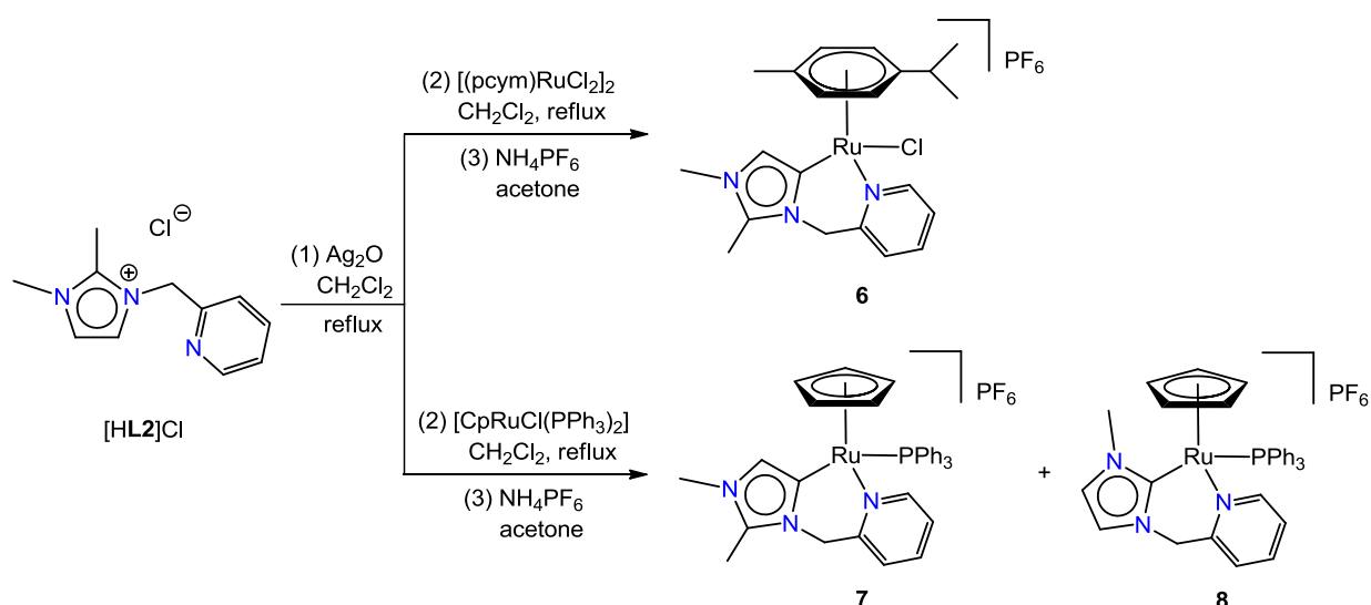
Scheme 3: Synthesis of picolyl-functionalized aNHC half-sandwich Ru(II) complexes.
