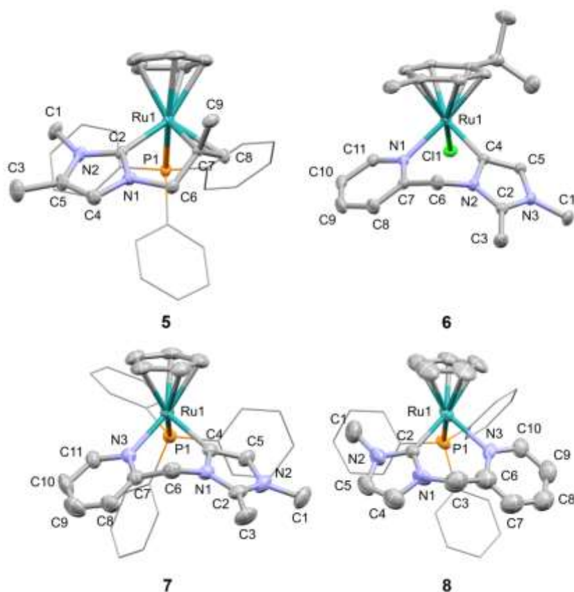
Figure 3: ORTEP plots of complexes 5–8 . Thermal ellipsoids are drawn at 50% level. For clarity, the phenyl moieties of PPh 3 are shown as wireframe presentations, and non-coordinating anions and hydrogens are omitted (structures of 7 and 8 have been obtained from a co-crystal).
