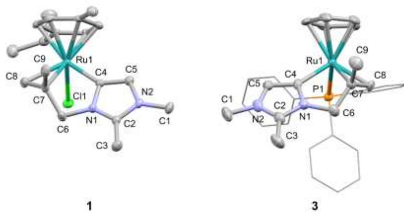
Figure 2: ORTEP plots of compounds 1 and 3 . Thermal ellipsoids are drawn at 50% level. For clarity, the phenyl moieties of PPh 3 are shown as wireframe presentations, and non-coordinating anions and hydrogens are omitted.
