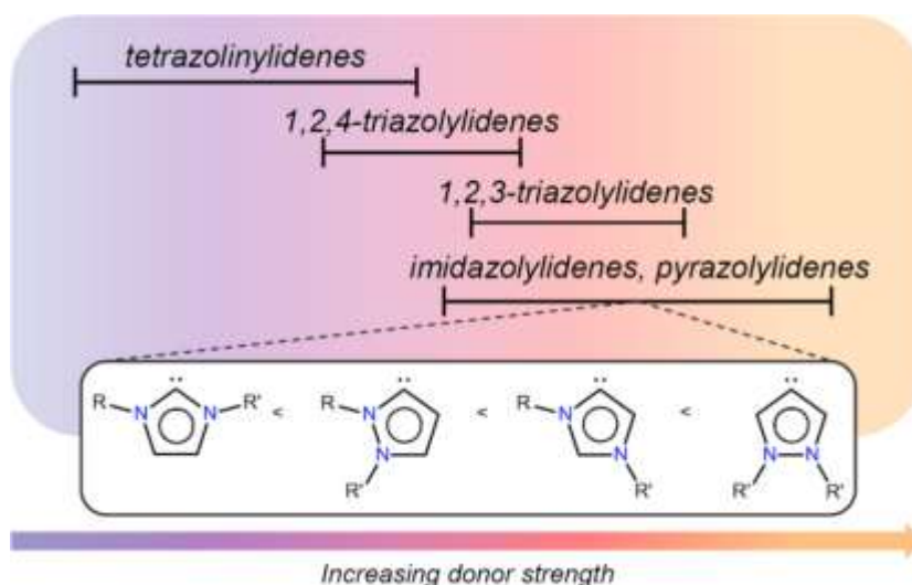
Figure 1: Order of donor strength of imidazolylidene and pyrazolylidene-based NHCs.
