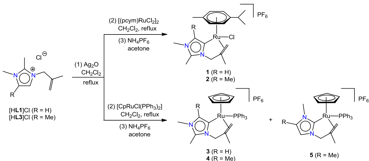
Scheme 2: Synthesis of aNHC half-sandwich Ru(II) complexes with an alkenyl chelating group.
