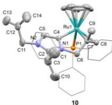
Figure 4: ORTEP plot of compound 10 . Thermal ellipsoids are drawn at 50% level. For clarity, the phenyl moieties of PPh 3 are shown as wireframe presentations, and non-coordinating anions and hydrogens are omitted.
