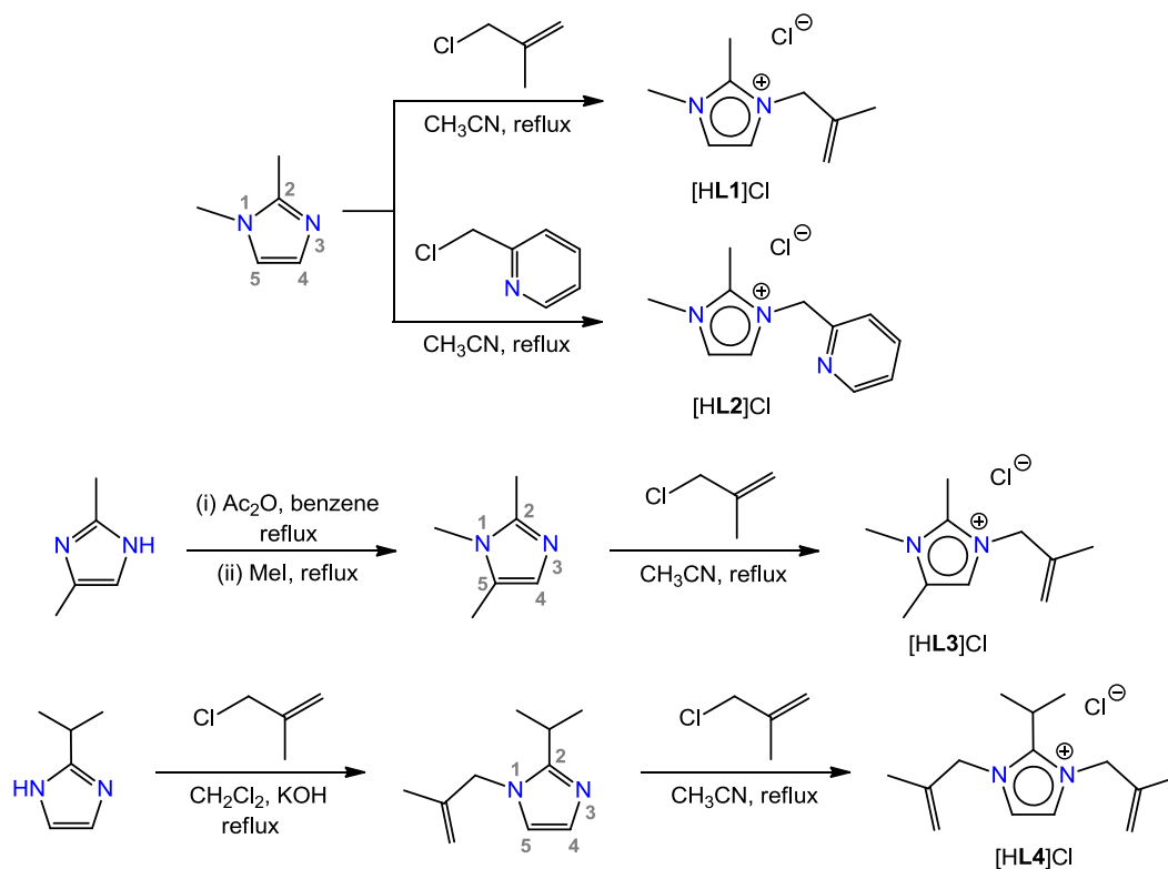
Scheme 1: Synthesis of the aNHC ligand precursors.
