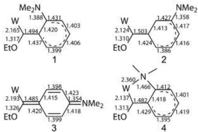
Figure 8. Bond distances (Å) [standard deviations are 0.002–0.004 Å (W–C), and 0.003–0.005 Å (all other bonds)] in the η 6 -coordinated arene rings and at the carbene carbons showing areas of delocalization for 1 and 2 and alternating long-short C–C arene bonds of 3 . Bond distances shown for 2 are mean values for the two independent molecules in the structure.
