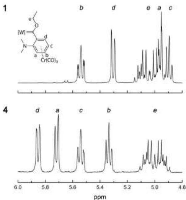
Figure 4. 1 H NMR spectra of the aromatic region of 1 (top) and 4 (bottom) in CDCl 3 at 298 K
