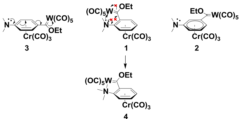
Figure 3. \pi -Resonance stabilization effects between the heteroatom and the carbene substituent in \pi -coordinated (arene)Cr(CO) 3 complexes of dimethylaniline
