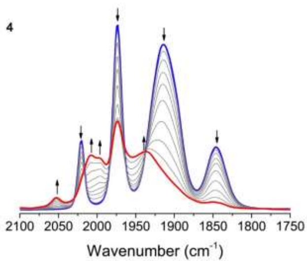
Figure 13. IR spectroscopic changes upon the oxidation of complexes 2 and 4 inside an OTTLE cell (1,2- \text{C}_2\text{H}_4\text{Cl}_2/\text{NBu}_4\text{PF}_6 , 298 K)
