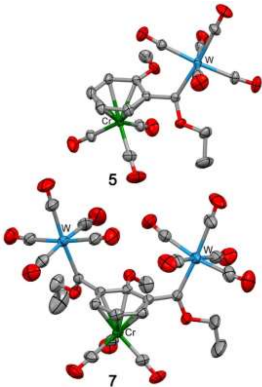
Figure 9. ORTEPs [40] of compounds 5 and 7 . Ellipsoids are set at 50% probability and hydrogen atoms omitted for clarity. Selected bond lengths [ \text{\AA} ]: W–C carb ( 5 ) 2.168(2), ( 7 ) 2.141(2), 2.144(3); C Ph –C carb ( 5 ) 1.503(3), ( 7 ) 1.504(3), 1.503(3); C carb –OEt ( 5 ) 1.316(3), ( 7 ) 1.301(3), 1.308(3) and torsion angles [ ^\circ ]: W–C carb –C ipso –C Ph ( 5 ) 60.6(2), ( 7 ) 102.3(2), -78.2(3) ; OEt–C carb –C ipso –C Ph ( 5 ) 54.1(2), ( 7 ) 114.0(2), -76.9(3)
