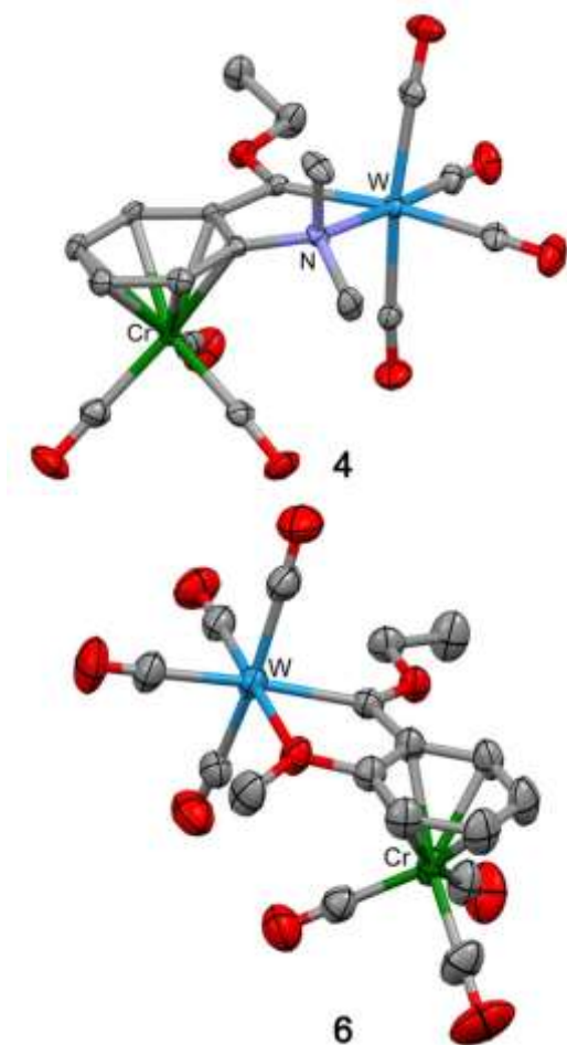
Figure 10. ORTEPs [40] of the \sigma,\pi -coordinated bimetallic carbene complexes 4 and 6 . Ellipsoids are set at 50% probability for \sigma,\pi -coordinated bimetallic carbene complexes. Hydrogen atoms omitted for clarity
