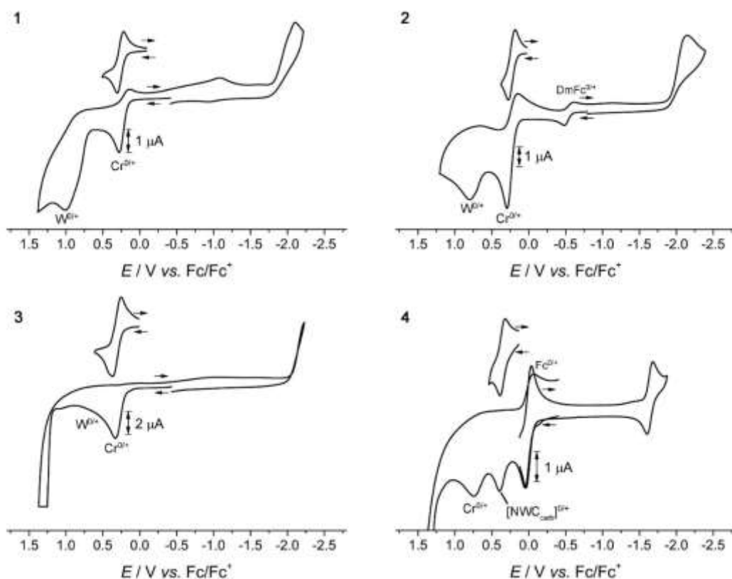
Figure 11. Cyclic voltammograms of complexes 1-4 in CH_2Cl_2/0.1 M NBu_4PF_6 against the ferrocene/ferrocenium standard at \nu = 100 mV/s
