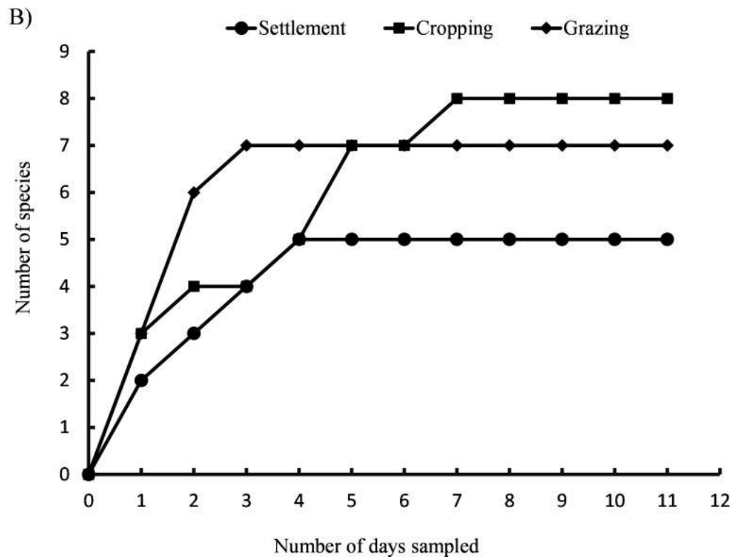
Supplementary Figure 2. Species accumulation curves to show sampling adequacy.
