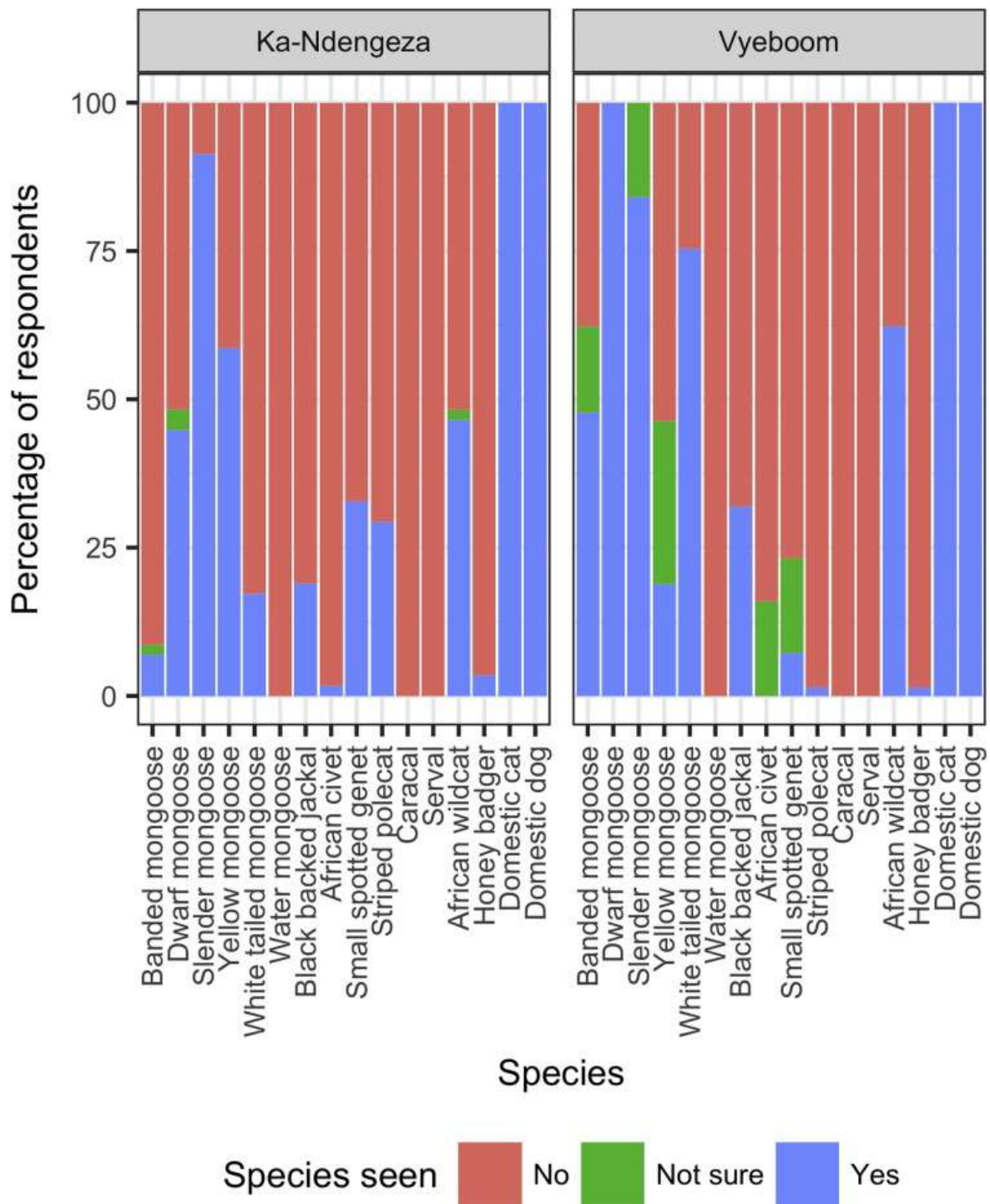
Supplementary Figure 3. Percentage of respondents in Ka-Ndengeza and Vyeboom that reported seeing species of small carnivores.
