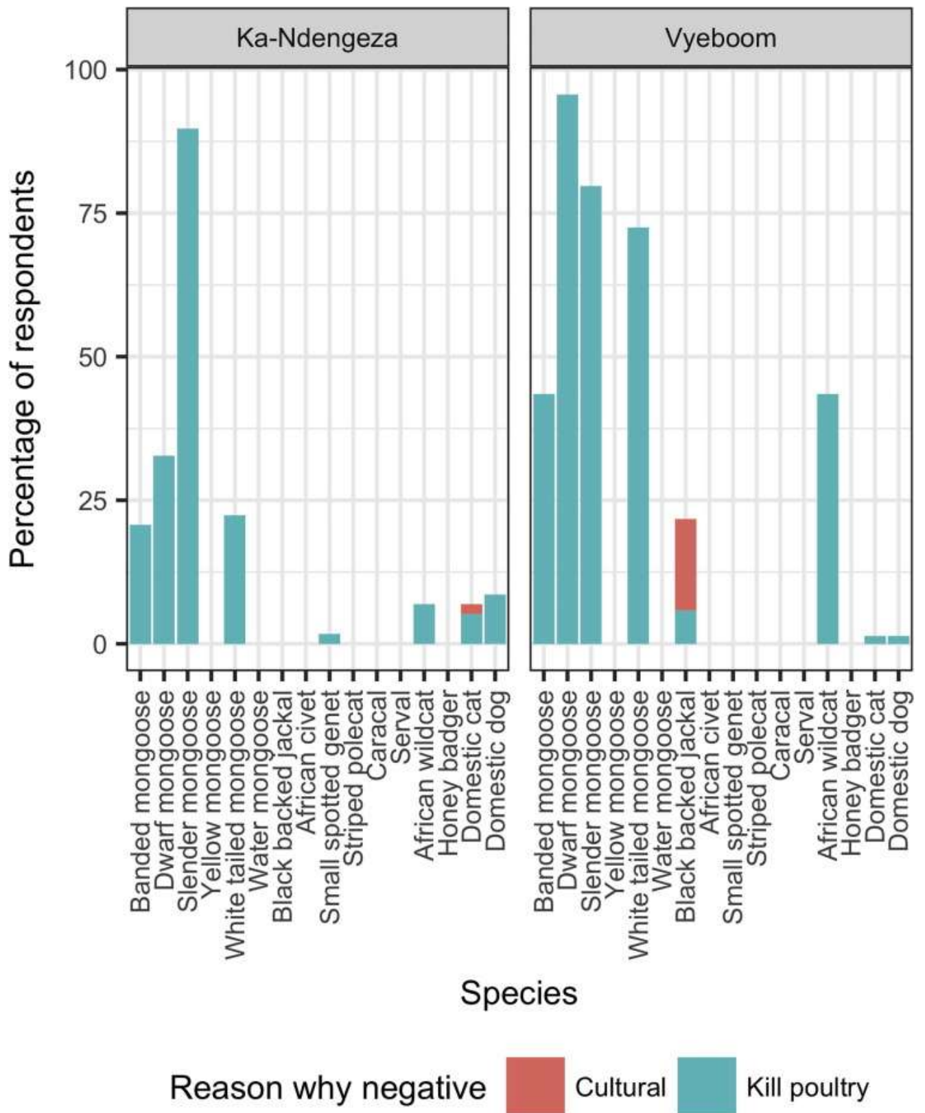
Supplementary Figure 4. Reasons provided why carnivores have impacted respondents negatively for Ka-Ndengeza and Vyeboom.
