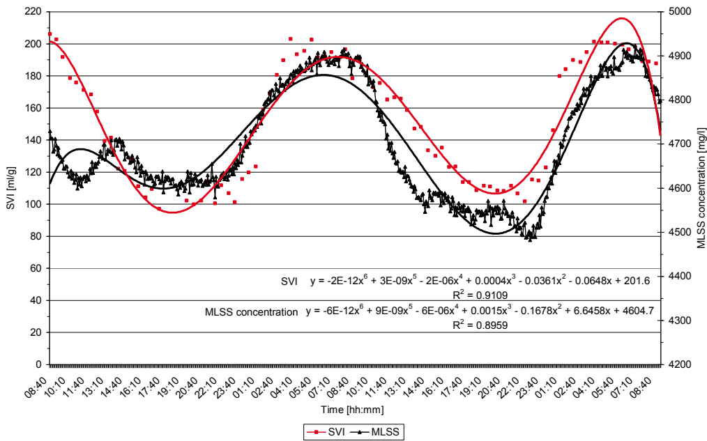
Figure 1 Experimental data and fitted curves of temporal variations in MLSS concentration and SVI
