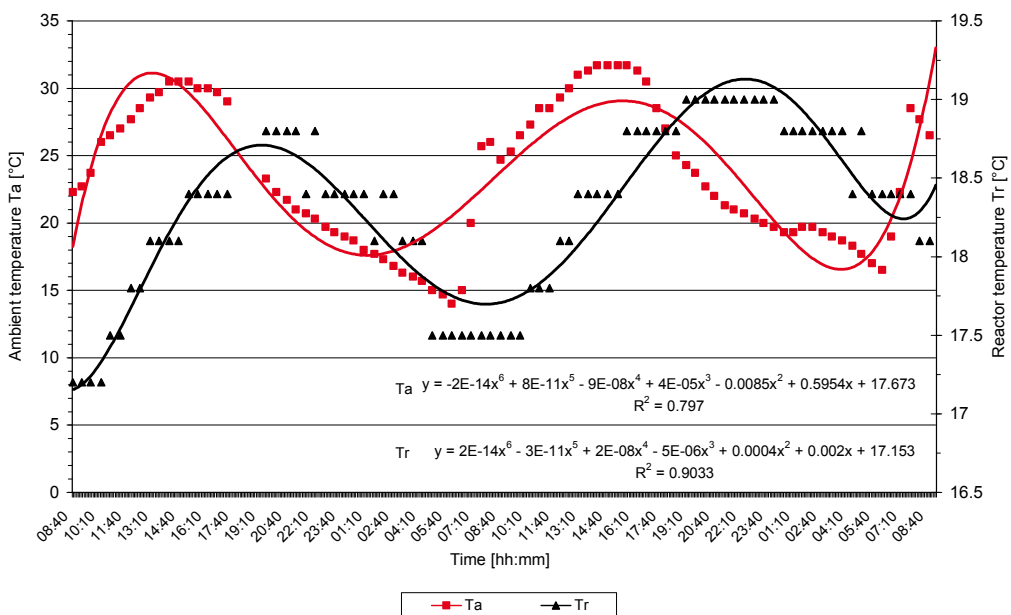
Figure 3 Experimental data and fitted curves of temporal variations in T_a and T_r
