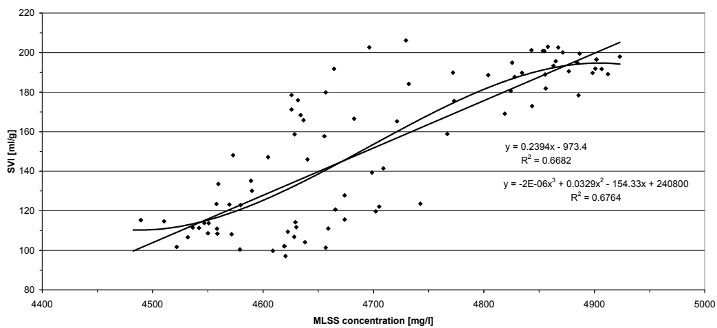
Figure 2 SVI and reactor MLSS concentration relationship
