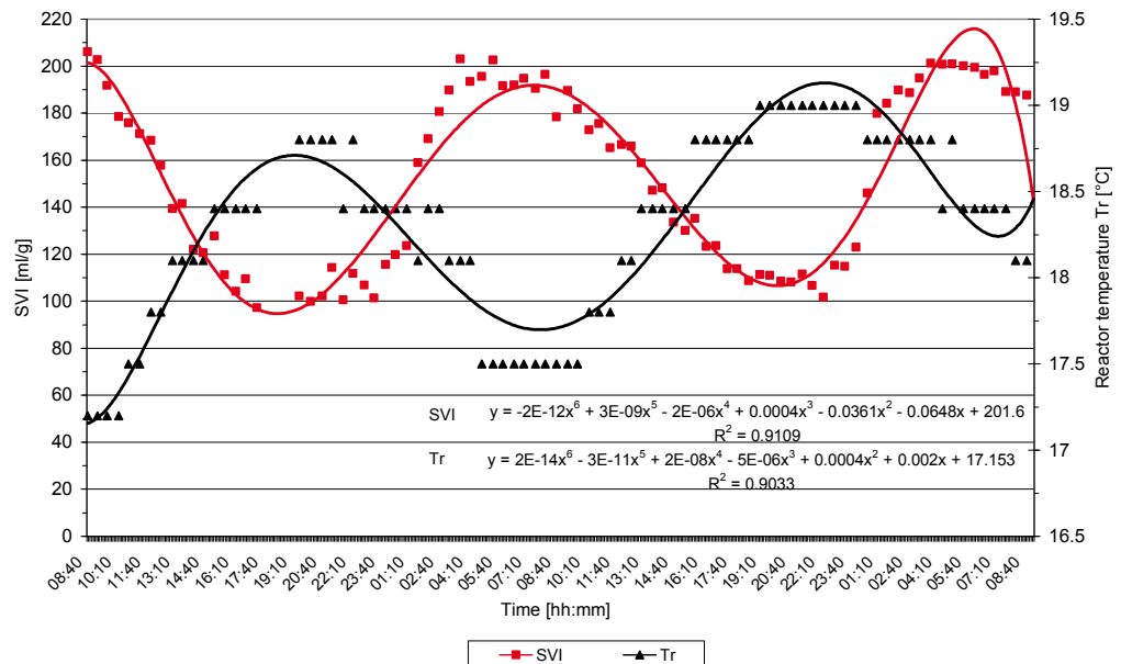
Figure 4 Experimental data and fitted curves of temporal variations in SVI and T_r
