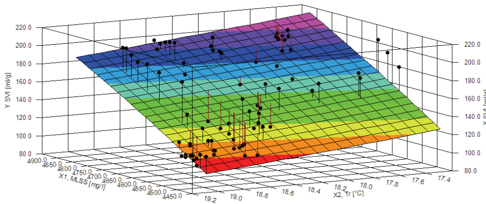
Figure 5 Experimental data points and modelled three-dimensional response surface of SVI ( y ) over the dependable variables MLSS concentration ( x_1 ) and T_r ( x_2 )
