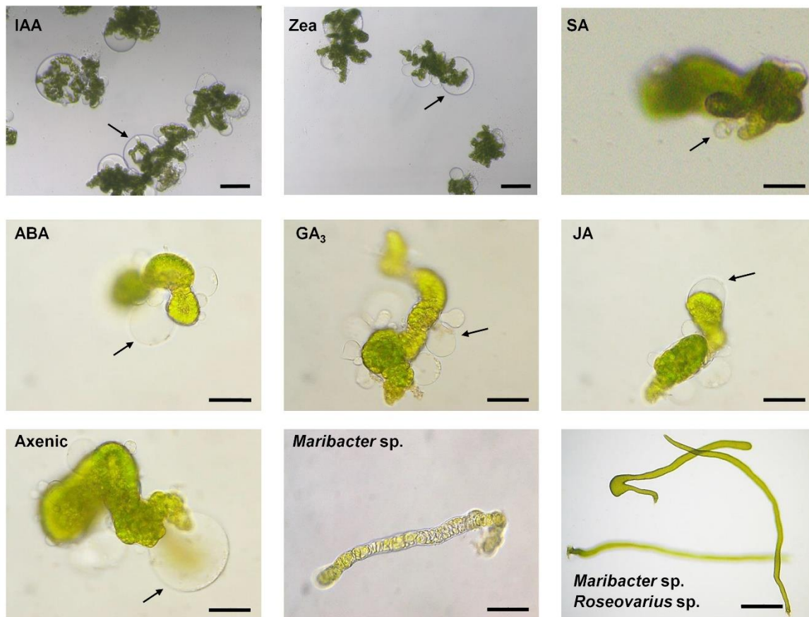
Figure S3. Morphogenetic bioassays of gametes inoculated with phytohormones. Related to Figure 6.
