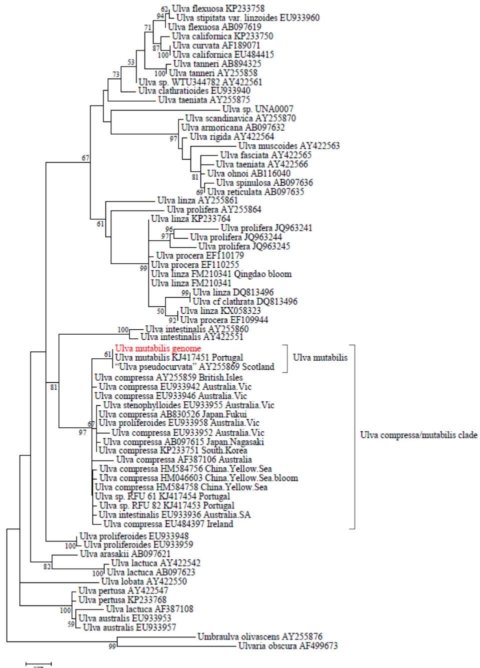
Figure S1. Phylogenetic position of the sequenced Ulva mutabilis strain. Related to Figure 1.
