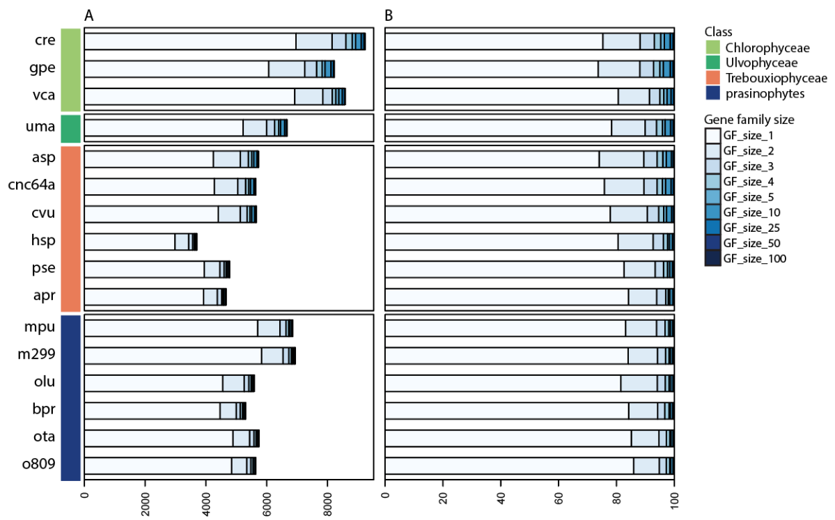
Figure S2. Distribution of gene family sizes in the green algal classes. Related to Figure 2.
